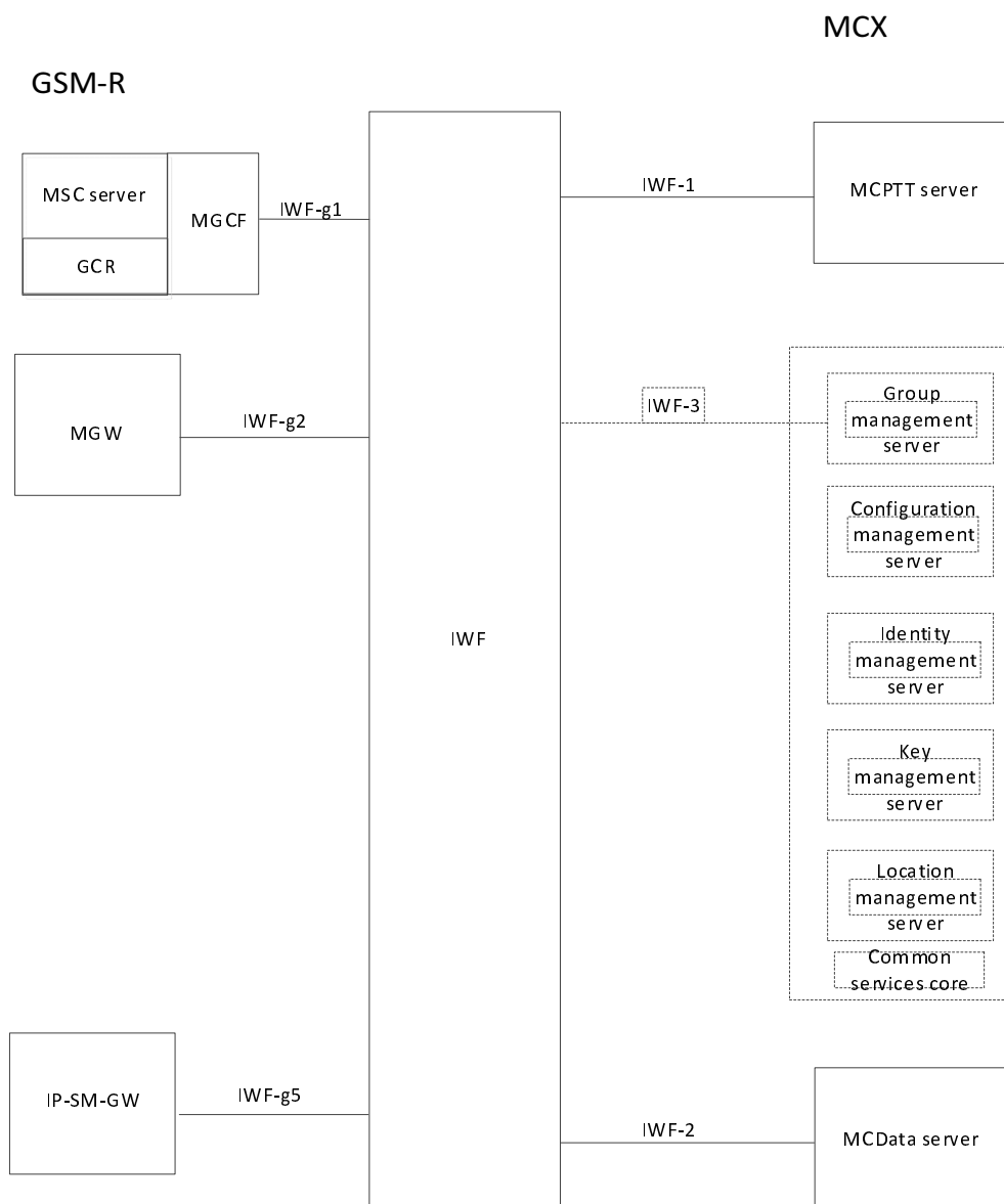
Figure 5.1-1: Interworking functional model
