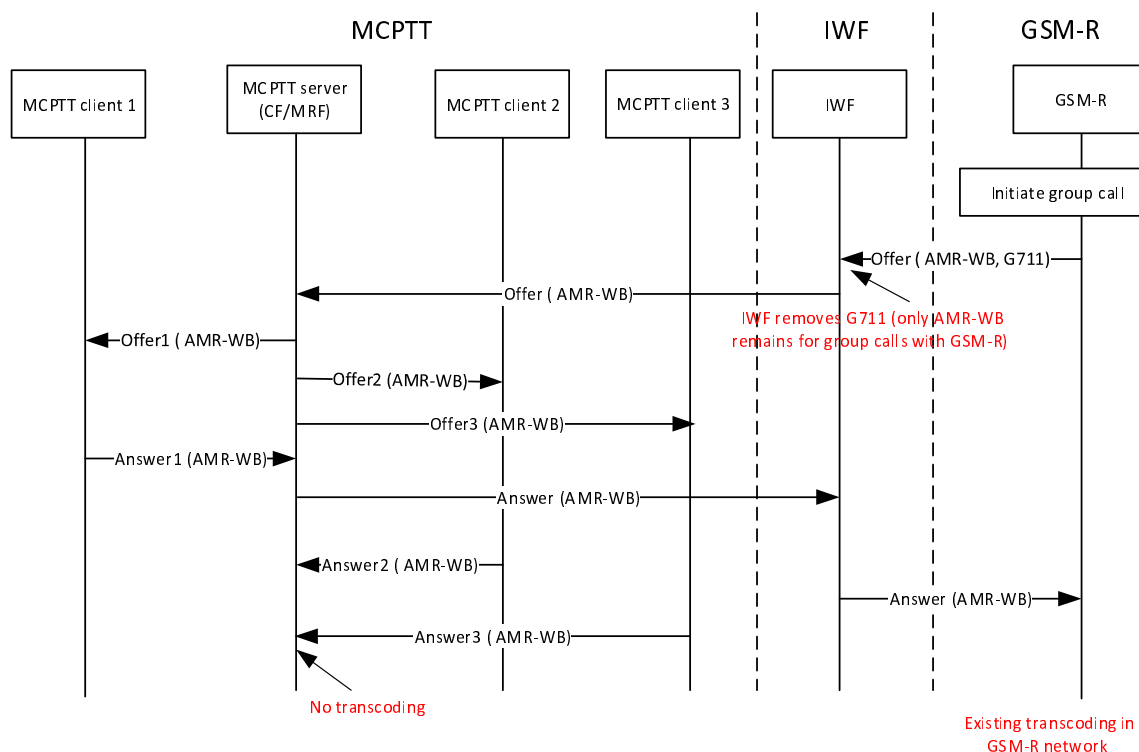
Figure 7.2.8.2-1: Codec negotiation for call initiated by a GSM-R user
