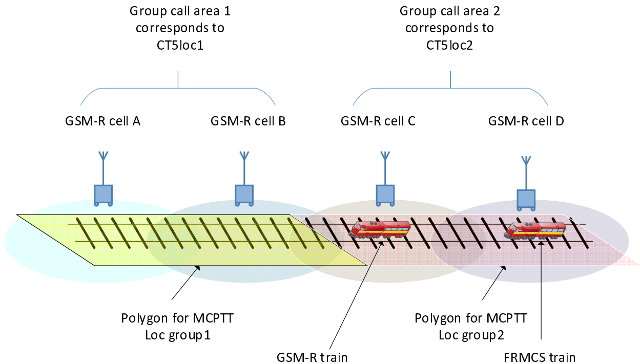
Figure 7.1.0-1: Network overview
