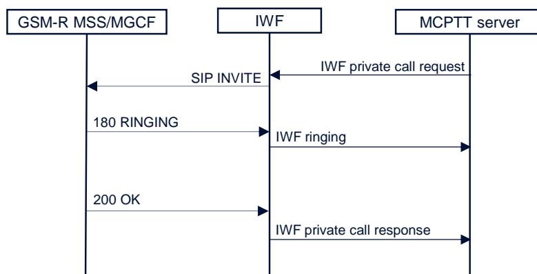
Figure 8.3.1.1-1: Point-to-point call initiated by an MCPTT user (stage 2)
