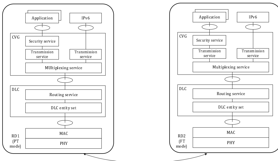
Figure 4.1-1: DECT-2020 Protocol Stack
