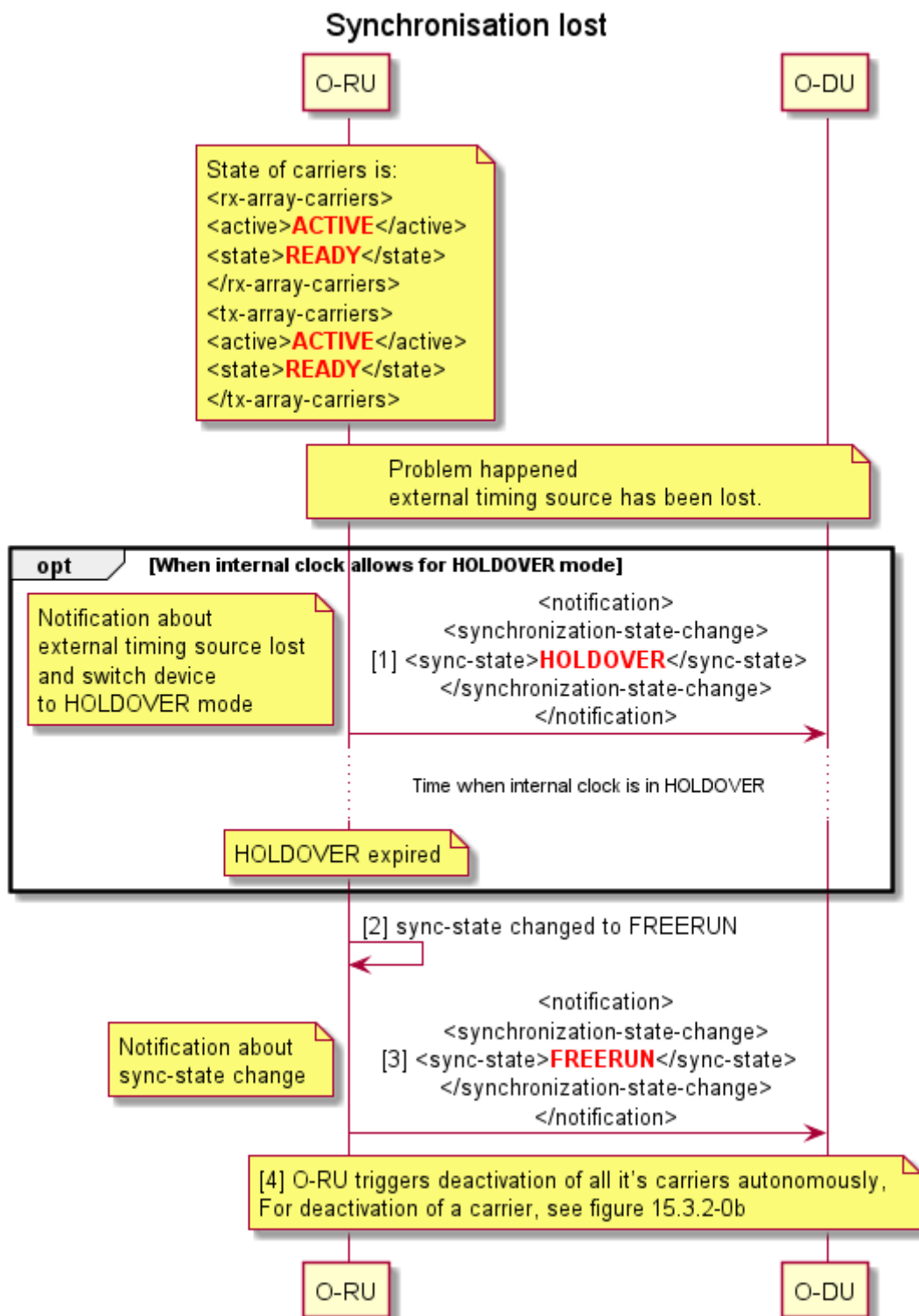
Figure 15.3.3.2-1: Synchronization lost scenario
