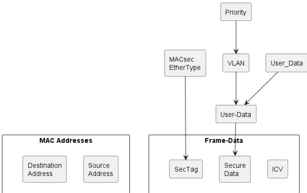
Figure 7.13.3-1: Base interface MACsec Frame, VLAN TAG and Priority Field
