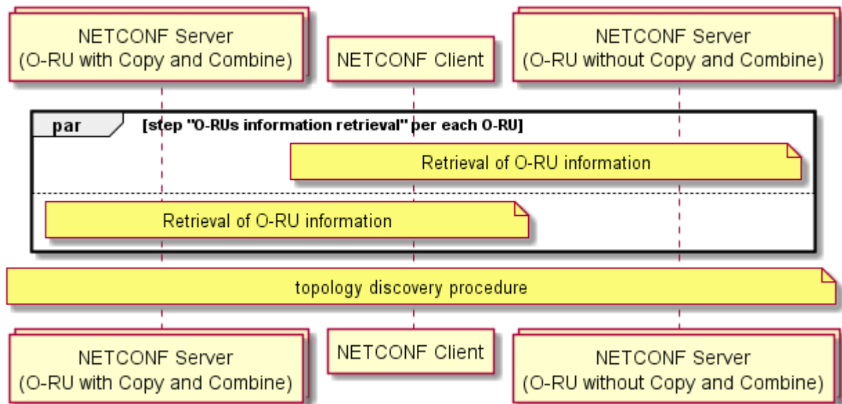
Figure 17.3-2: RU information retrieval and topology detection at the start-up
