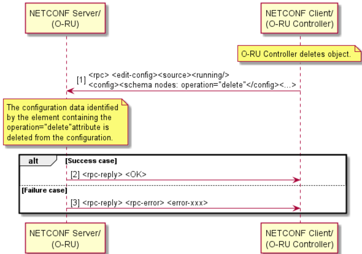
Figure 9.1.6-1: Delete Parameters
