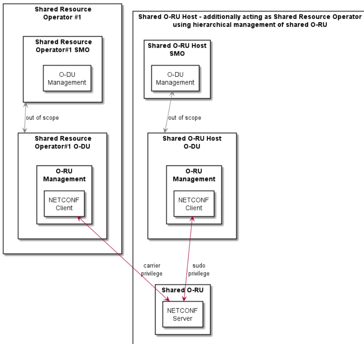
Figure 19.2-3: Shared O-RU M-Plane Architecture where the Shared O-RU Host is additionally a Shared Resource Operator managing Shared O-RU using hierarchical approach
