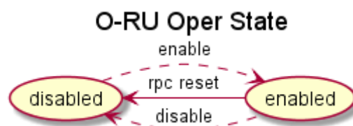
Figure 9.1.3-5: Oper State
