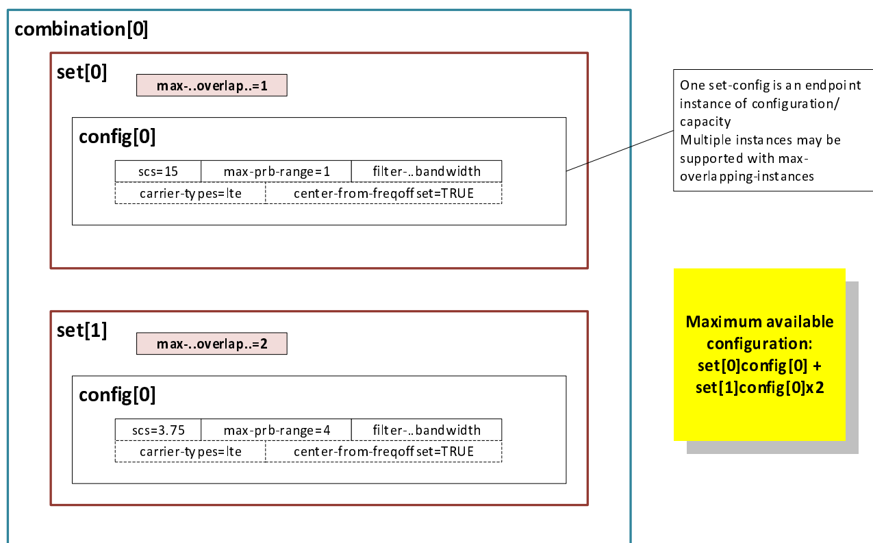
Figure 15.9-2: Example a static-low-level-rx-endpoint indirectly indicating support for a single NB-IoT carrier support with one NPUSCH and two NPRACH channels
