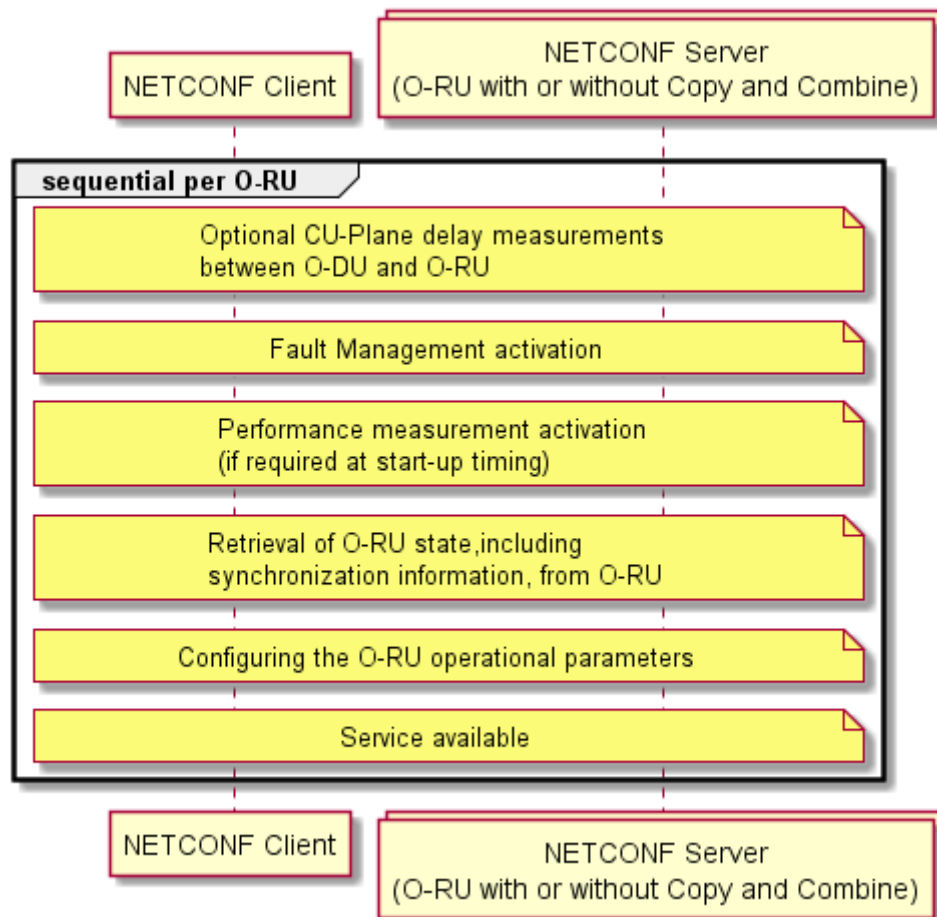
Figure 17.3-5: Further steps for start-up procedure
