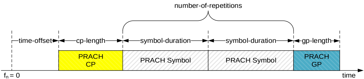
Figure 15.6.4-1: Timing-related parameters of single PRACH occasion
