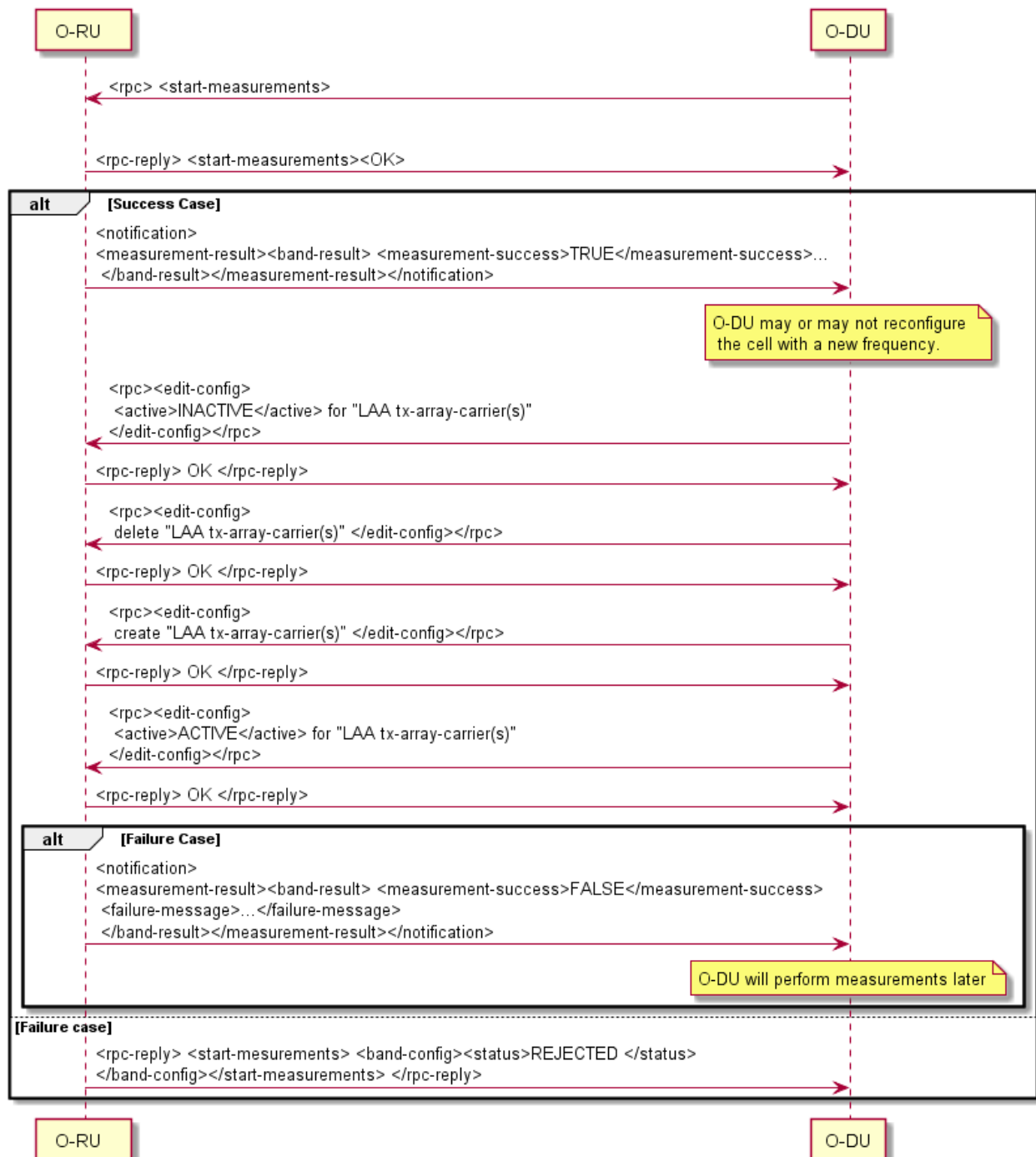
Figure 16.1-1: Carrier-Selection Call-flow
