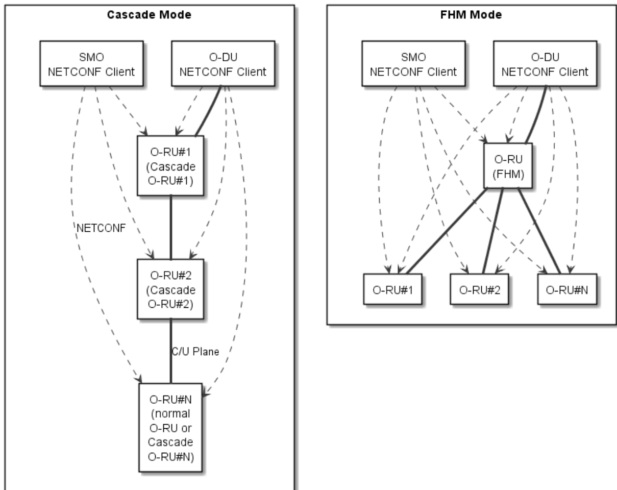
Figure 17.2-1: M-Plane Connection
