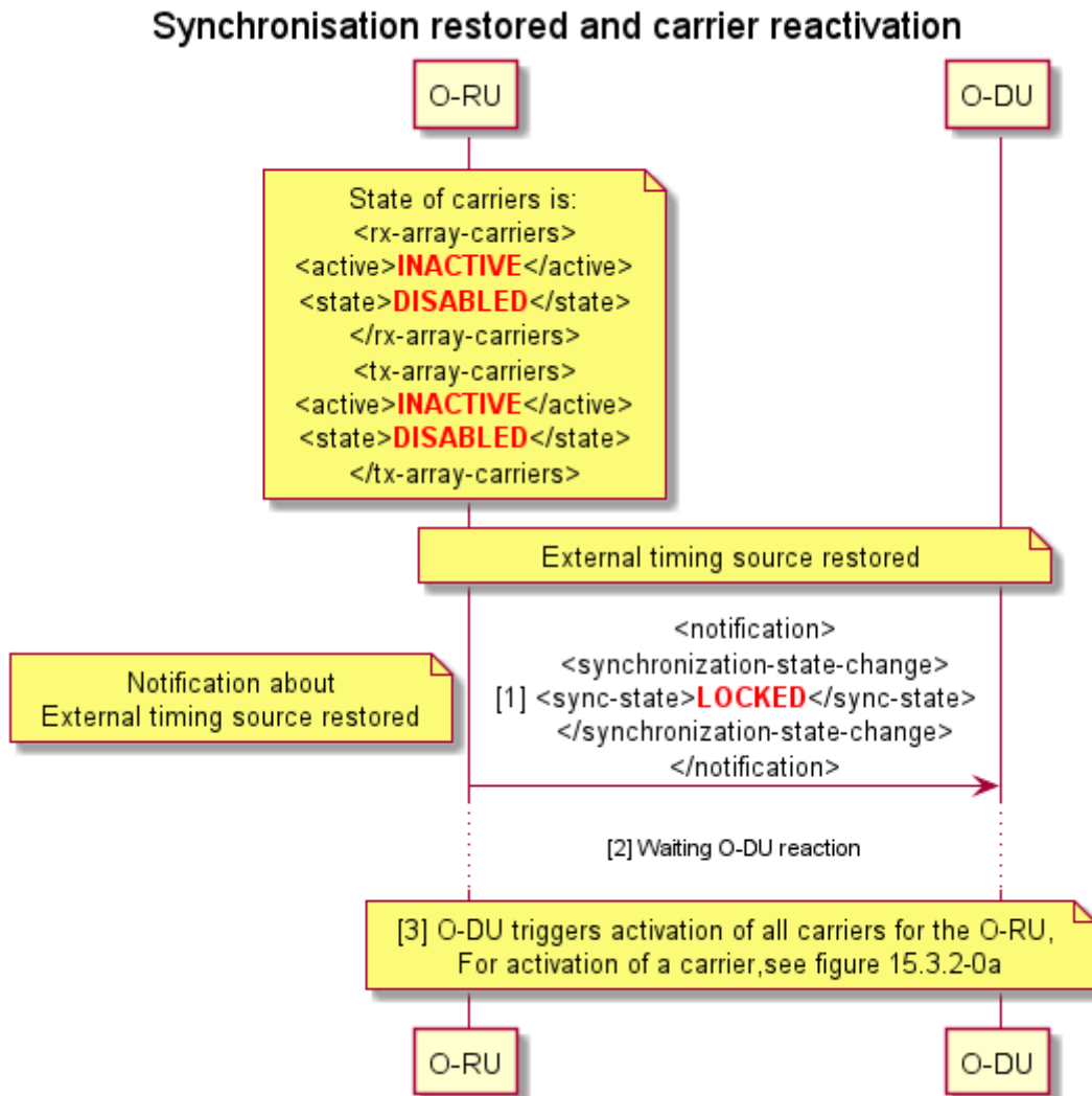
Figure 15.3.3.3-1: Synchronization restored and carrier reactivation scenario
