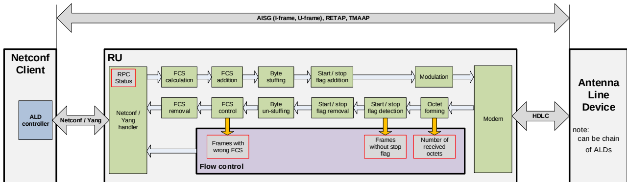
Figure 14.4.2-1: ALD Reference Architecture
