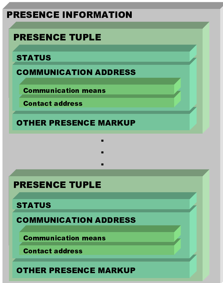
Figure 4: Presence information
