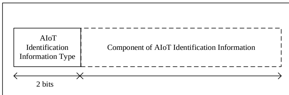
Figure 31.7.1: Structure of AIoT Identification Information
