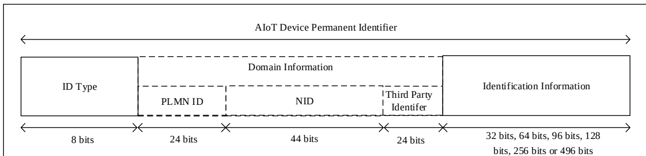
Figure 31.2-1: Structure of AIoT Device Permanent Identifier
