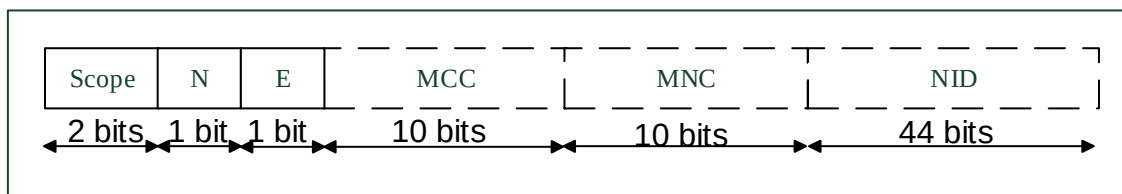
Figure 24.3.2-1: Structure of PLMN ID in ProSe Application Code
