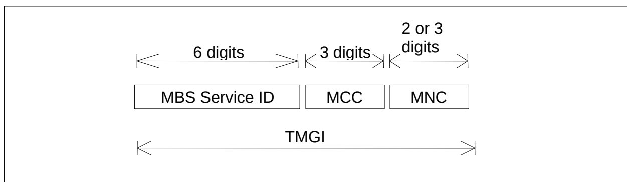
Figure 30.2.1: Structure of TMGI
