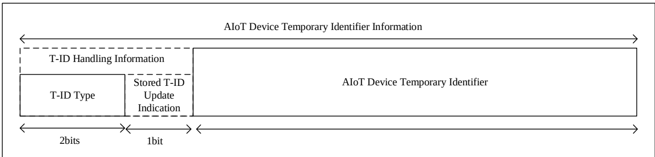
Figure 31.6-1: Structure of AIoT Device Temporary Identifier Information
