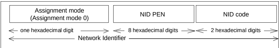
Figure 12.7.2-1: NID of assignment mode 0
