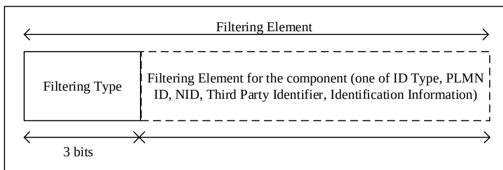
Figure 31.3.2: Structure of Filtering Element
