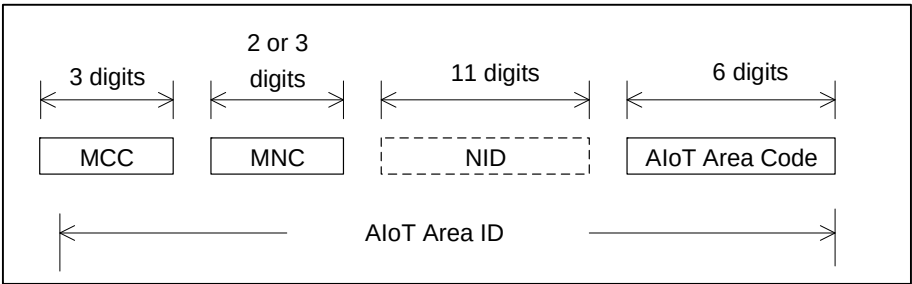
Figure 31.4.1: Structure of the AIoT Area ID
