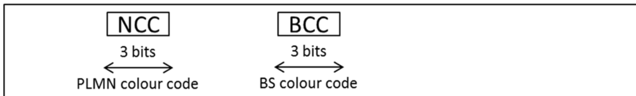
Figure 6: Structure of 6 bit BSIC
