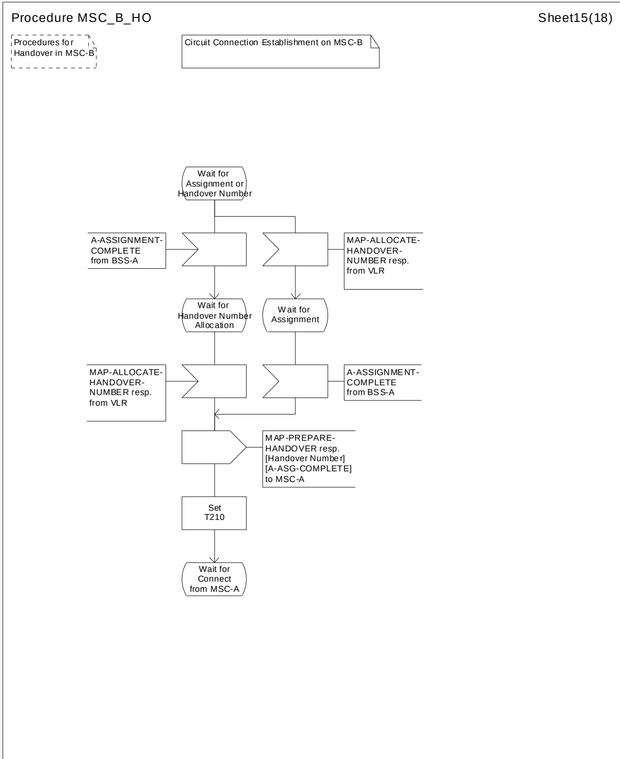
Figure 42 (Sheet 15 of 18): Handover control procedure in MSC-B
