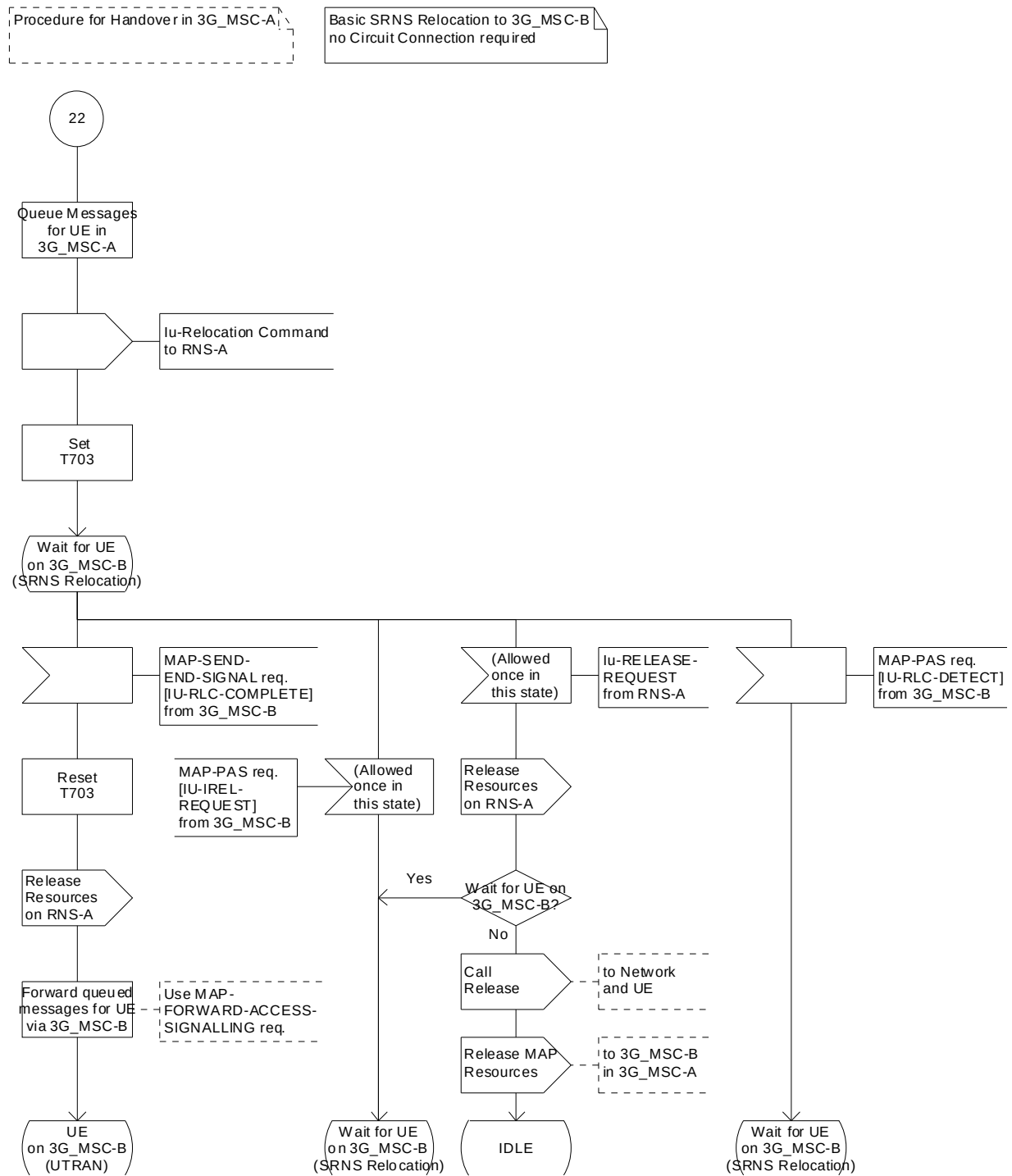
Figure 43 (sheet 71 of 78): Handover control procedure in 3G_MSC-A
