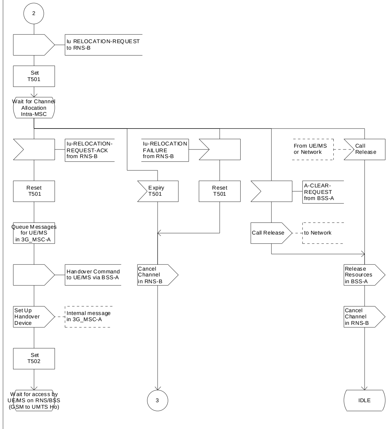
Figure 43 (sheet 2 of 78): Handover control procedure in 3G_MSC-A
