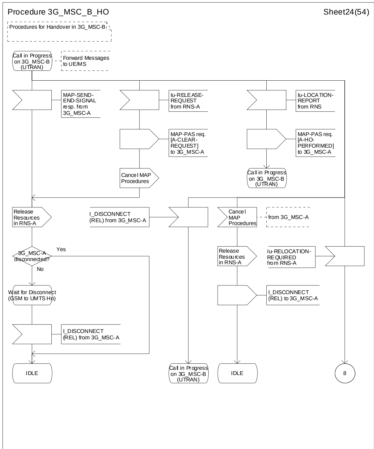
Figure 44 (sheet 24 of 54): Handover control procedure in 3G_MSC-B
