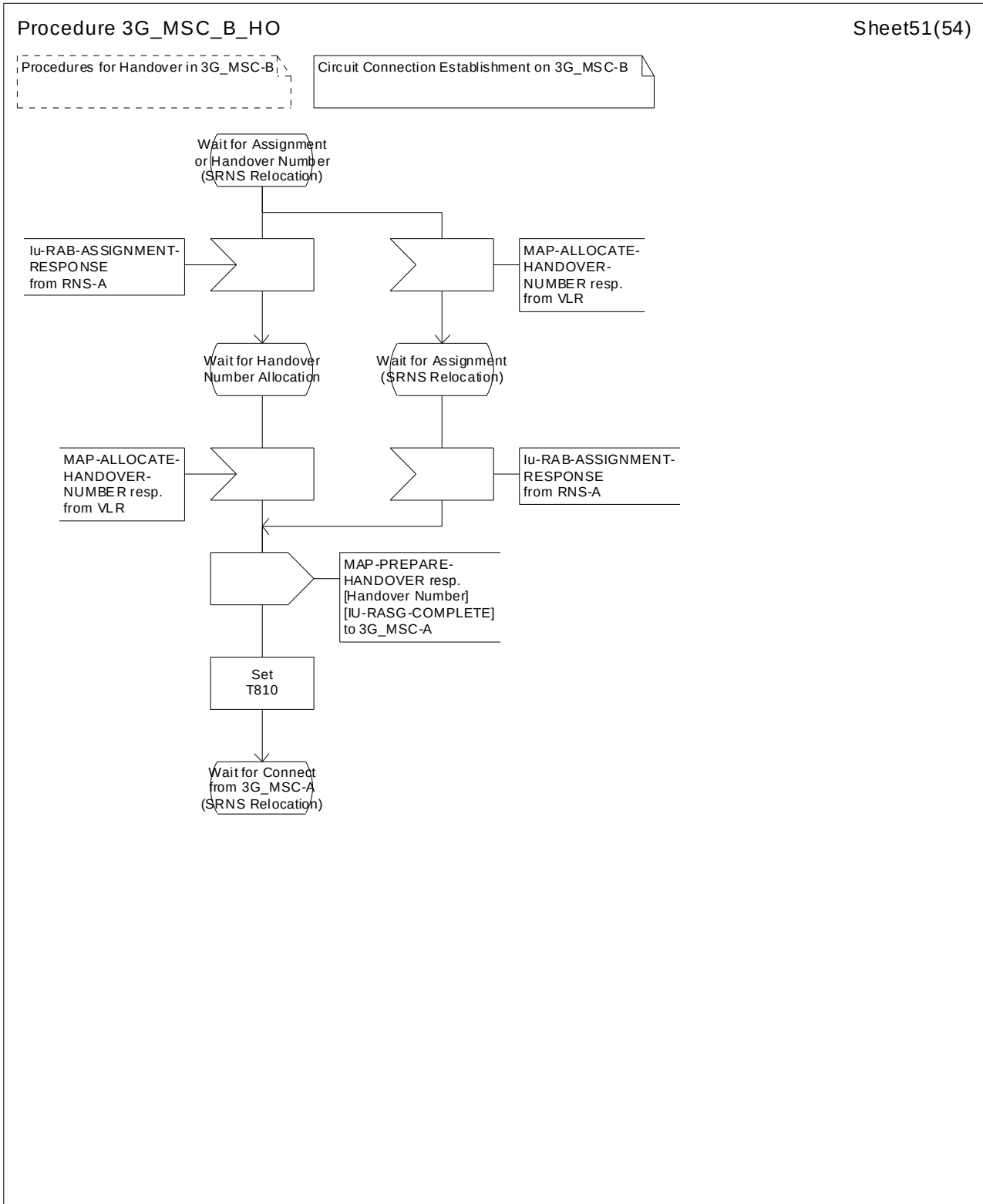
Figure 44 (sheet 51 of 54): Handover control procedure in 3G_MSC-B
