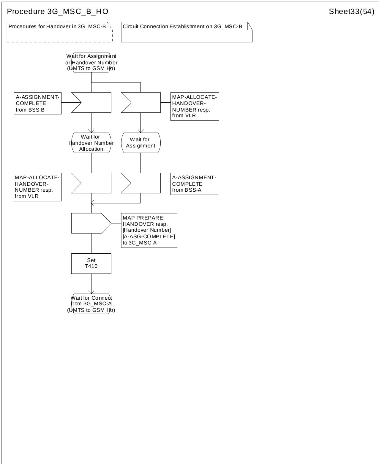
Figure 44 (sheet 33 of 54): Handover control procedure in 3G_MSC-B
