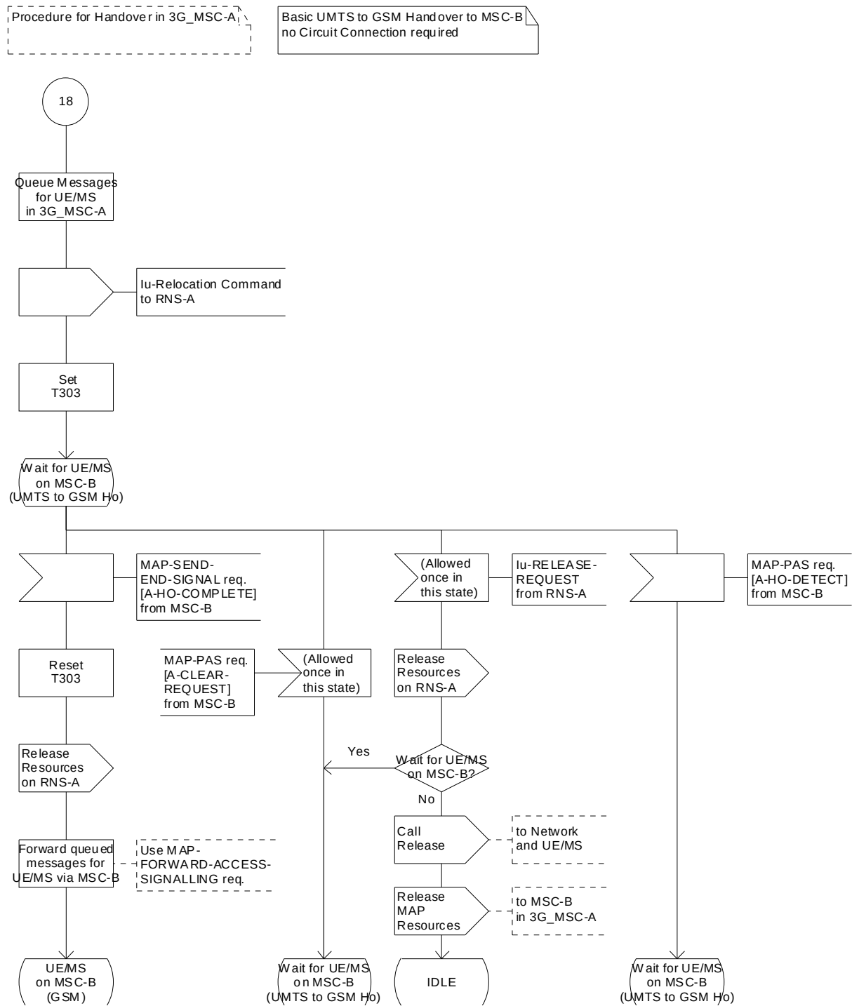
Figure 43 (sheet 49 of 78): Handover control procedure in 3G_MSC-A
