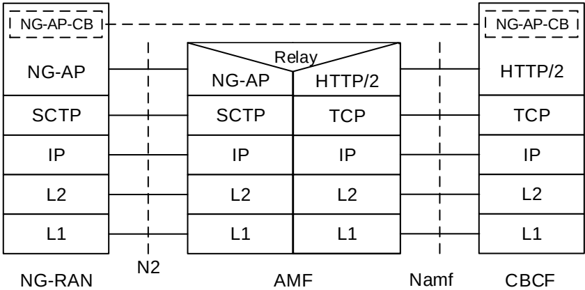
Figure 9.1.6-1: CBCF - NG-RAN
