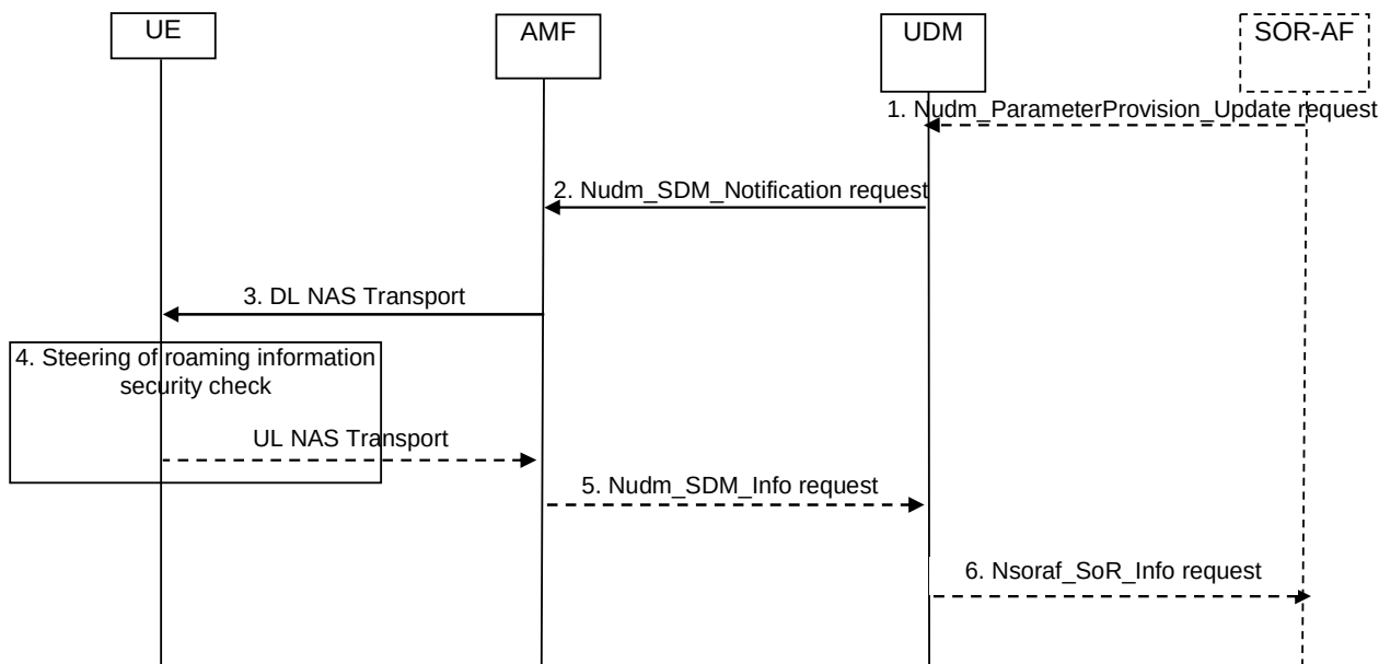
Figure C.7.1: Procedure for configuring UE with SOR-SNPNI-SI or SOR-SNPNI-SI-LS in a PLMN after registration
