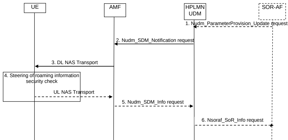
Figure C.3.1: Procedure for providing list of preferred PLMN/access technology combinations and the SOR-CMCI, if any, or secured packet after registration
