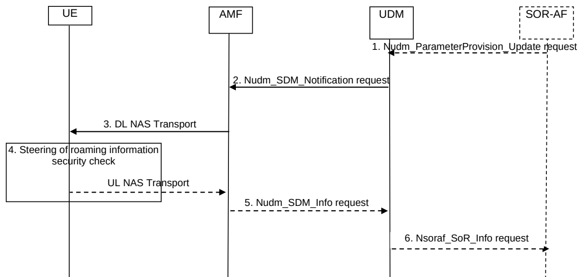
Figure C.7.1: Procedure for configuring UE with SOR-SNP-SI or SOR-SNP-SI-LS in a PLMN after registration
