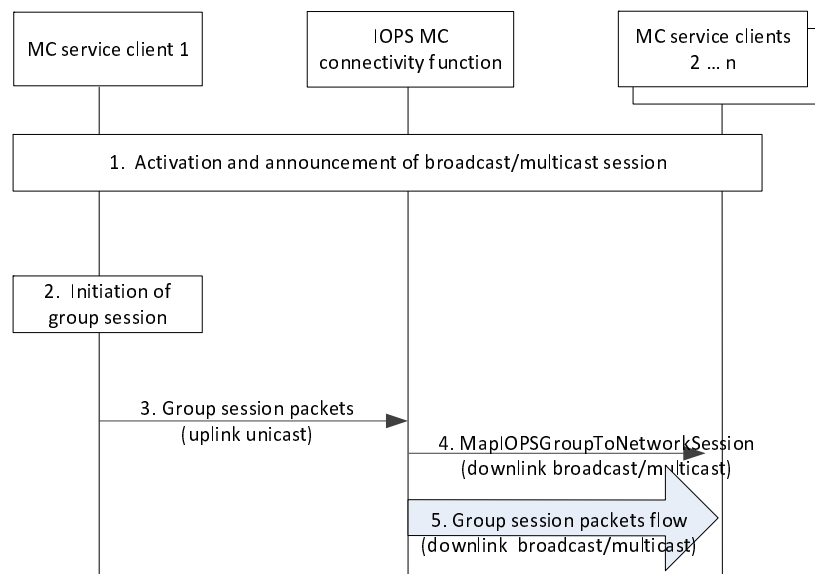
Figure 10.4.5.2.1-1: Group session connect on broadcast/multicast session (IP connectivity functionality)
