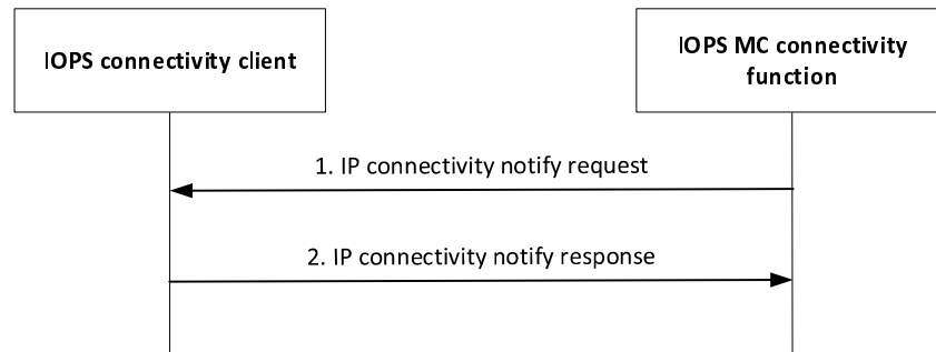
Figure 10.3.3-2 IP connectivity notification in the IOPS mode of operation
