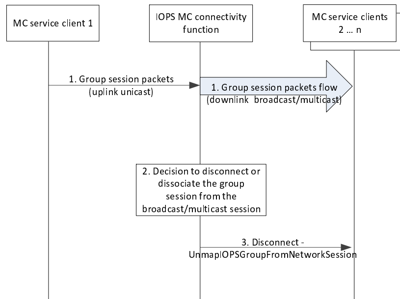
Figure 10.4.5.2.2-1: Group session disconnect on broadcast/multicast session (IP connectivity functionality)
