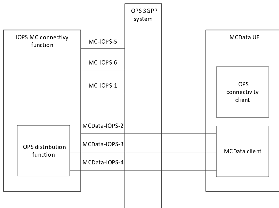
Figure 7.3.4-1: MCDATA functional model for the application plane in the IOPS mode of operation
