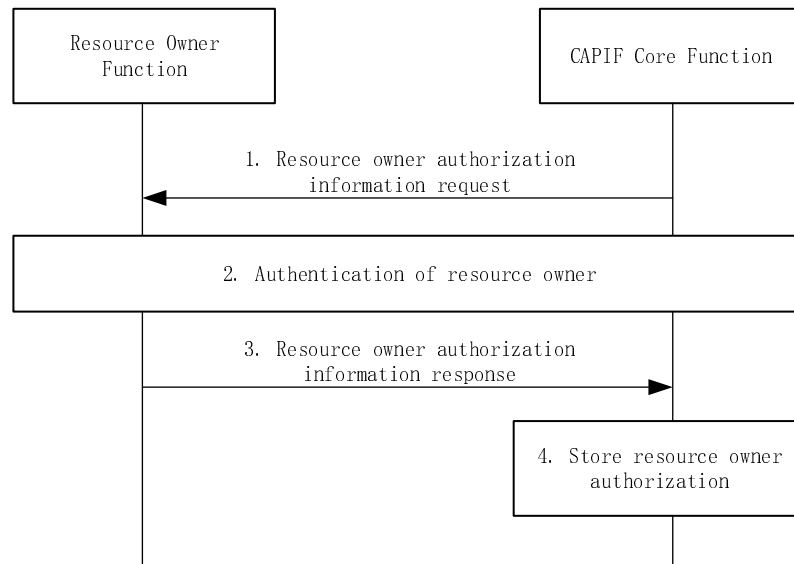
Figure 8.36.3-1: Procedure for obtaining resource owner authorization
