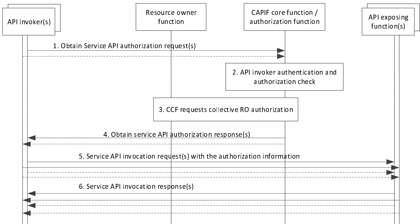
Figure 8.33.3-1: Procedure for obtaining collective authorization from resource owner
