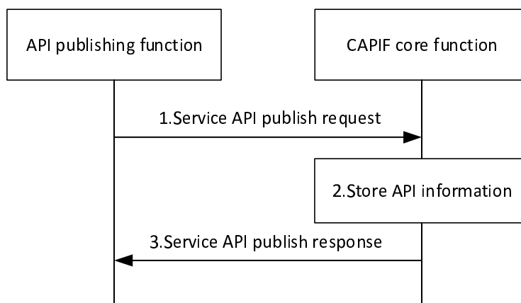
Figure 8.3.3-1: Publish service APIs
