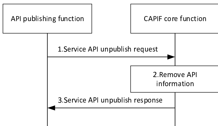
Figure 8.4.3-1: Unpublish service APIs
