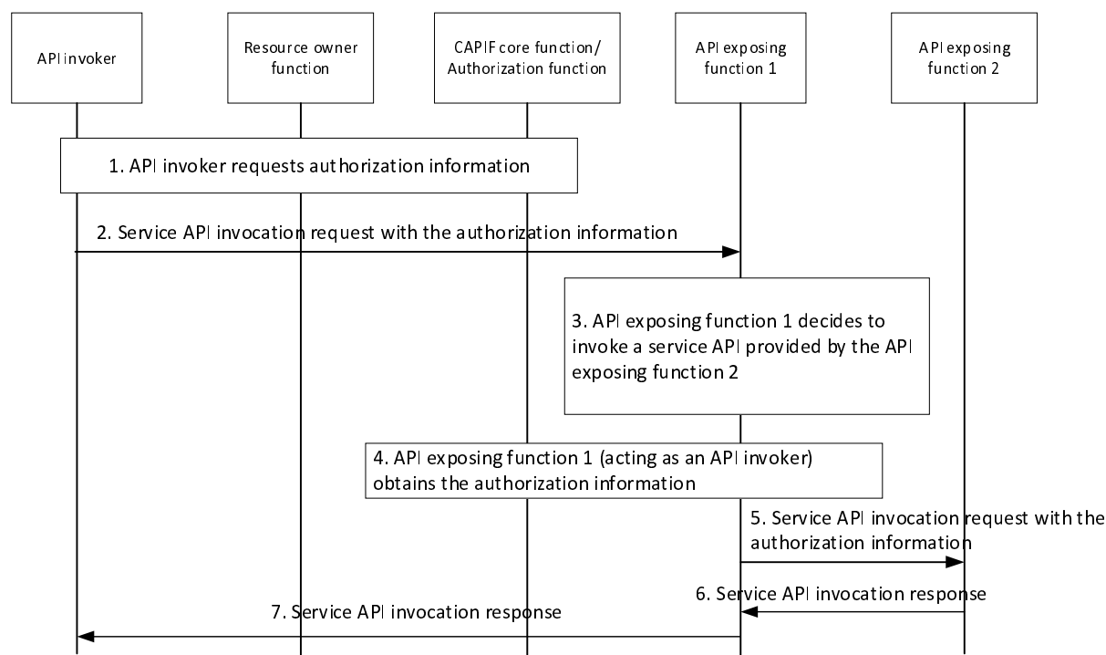
Figure 8.32.3-1: Procedure for obtaining authorization information in a nested API invocation
