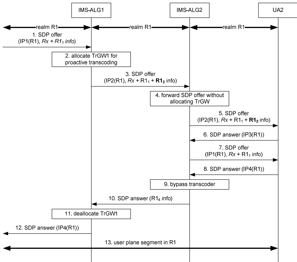
Figure Q.7: IMS-ALG bypasses its TrGW and prior unrequired proactive transcoder
