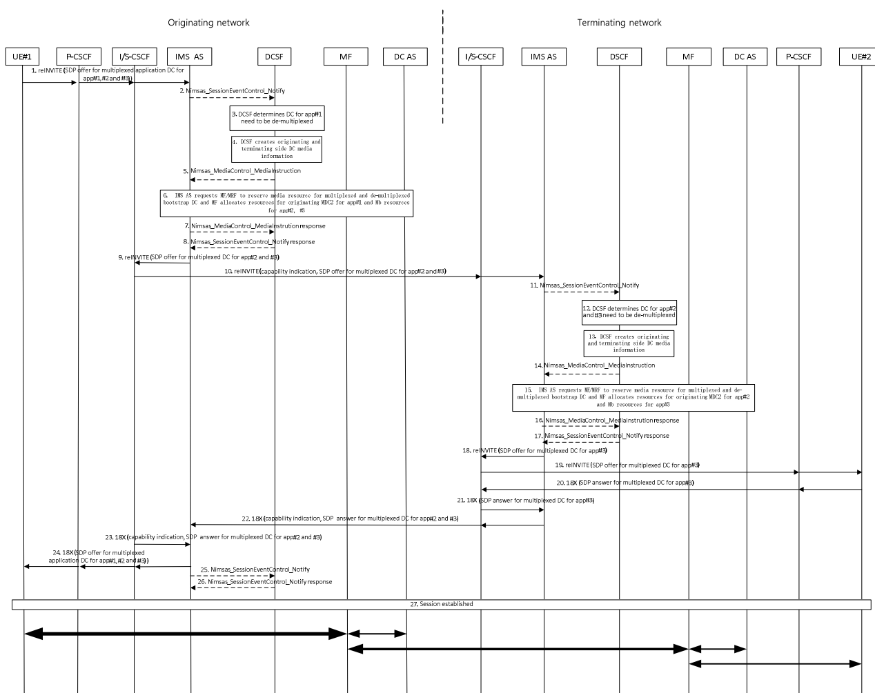
Figure AC.7.10.4.2.1-1: Application data channel multiplexing when both originating and terminating networks support data channel multiplexing
