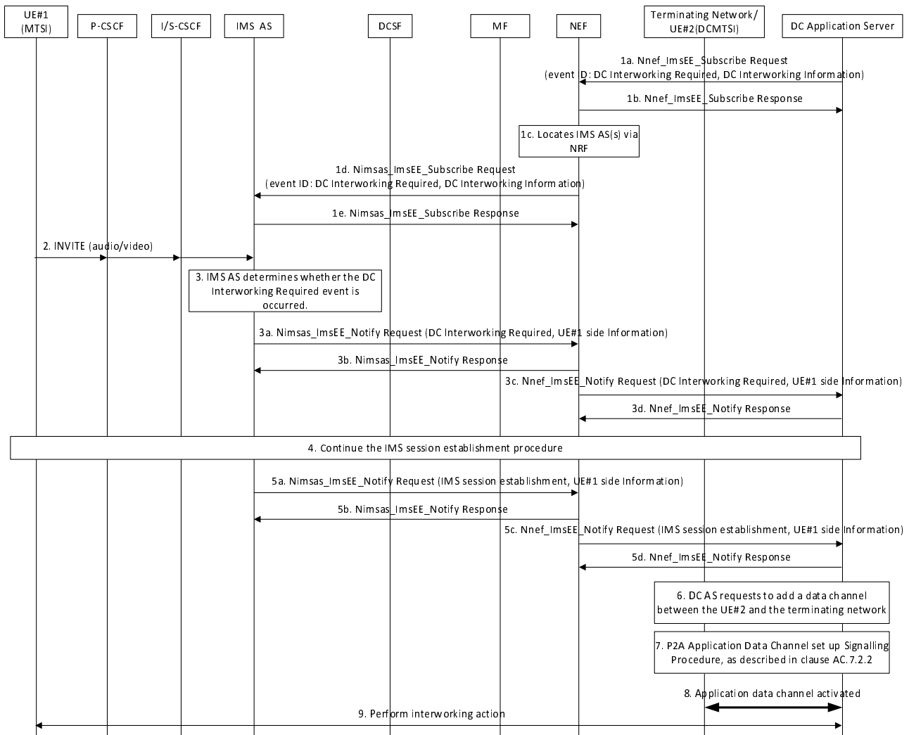
Figure AC.7.9.4-1: Application Data Channel set up signalling procedure for IMS data channel interworking with originating MTSI UE via DC application server
