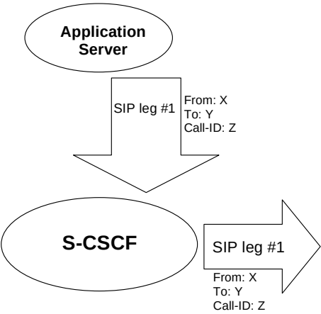
Figure 4.3b: Application Server acting as originating UA
