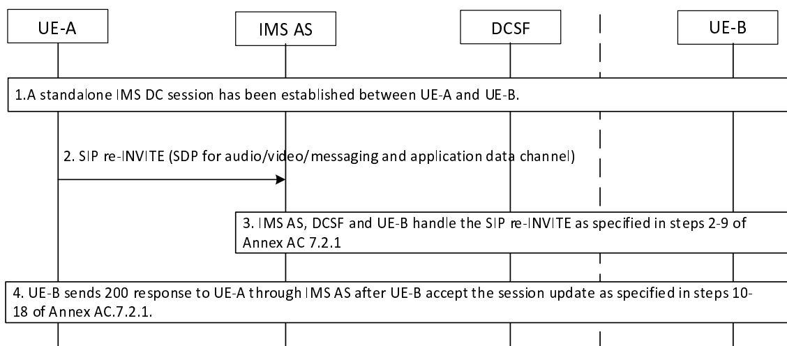
Figure AC.10.2.4-1: Adding MMTel Media to standalone IMS data channel session
