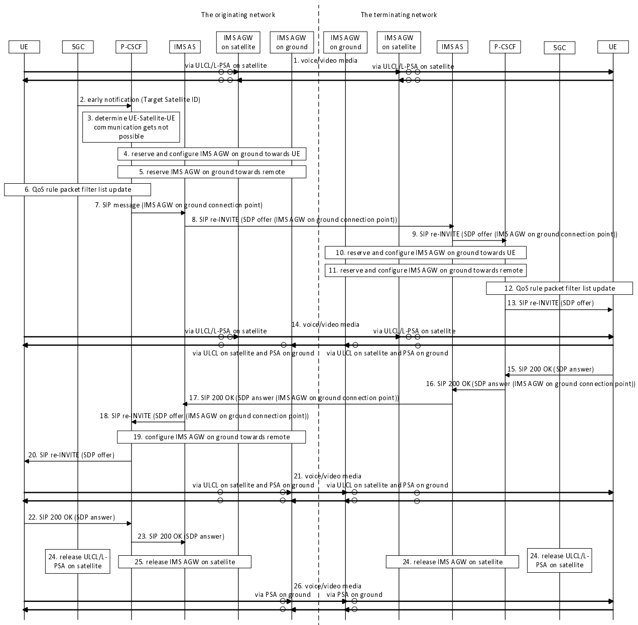
Figure AE.5.2.2-1: Ground fallback procedure
