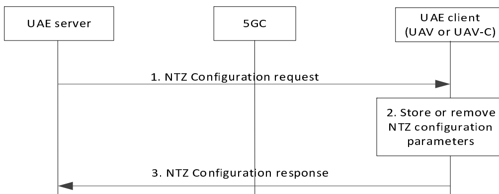
Figure 7.11.2.2-1: NTZ configuration
