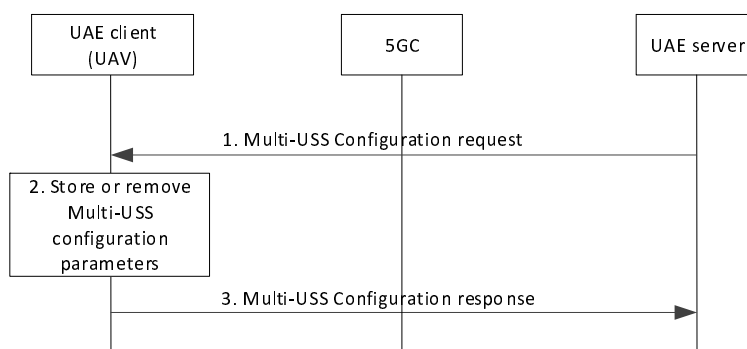
Figure 7.6.2.2-1: Multi-USS configuration
