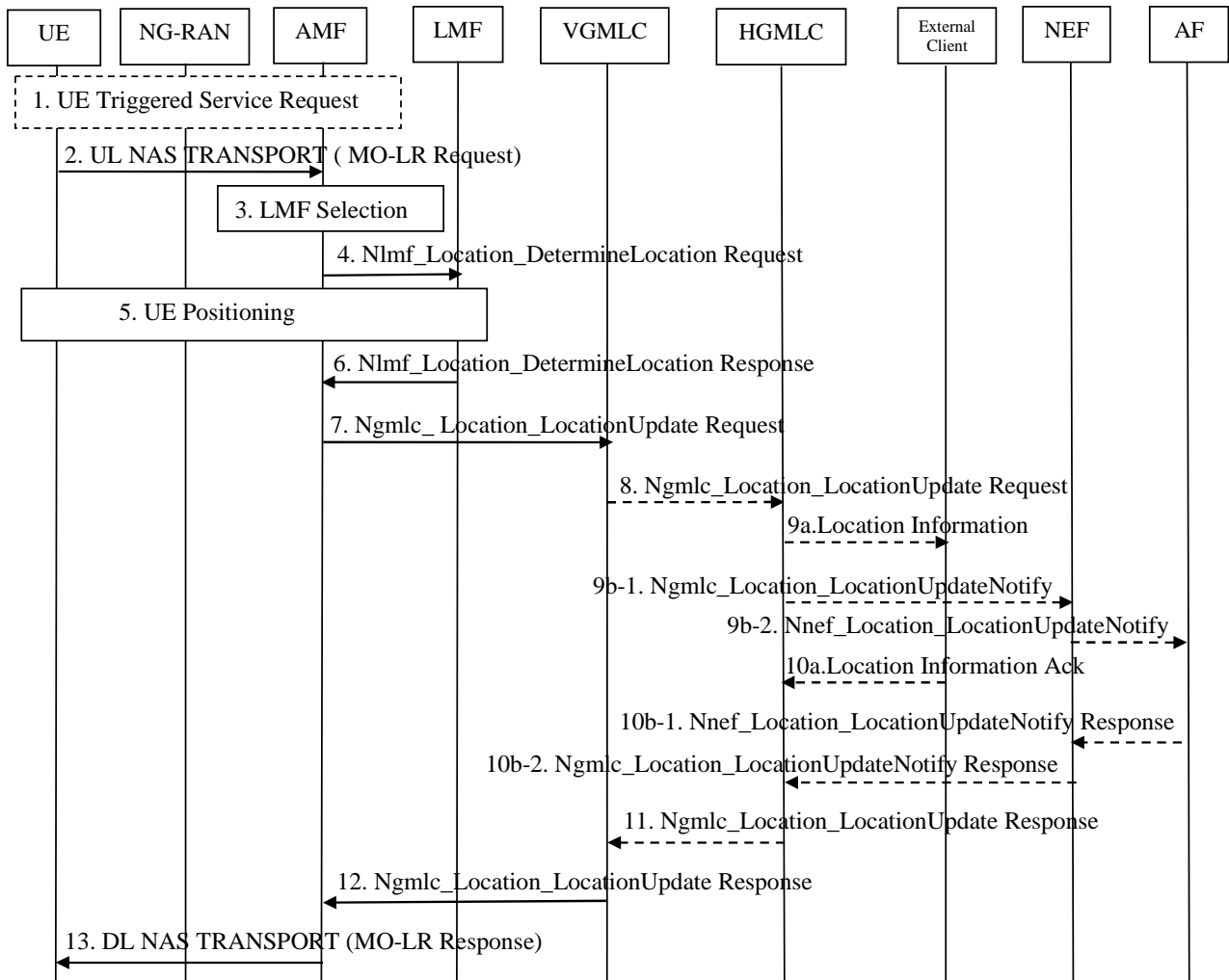
Figure 6.2-1: 5GC-MO-LR Procedure
