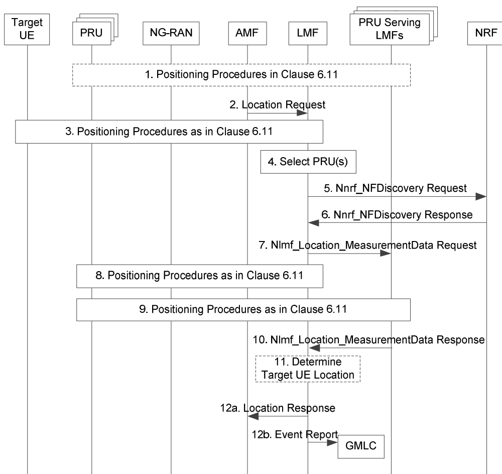
Figure 6.17.4-1: Location of a target UE using PRUs
