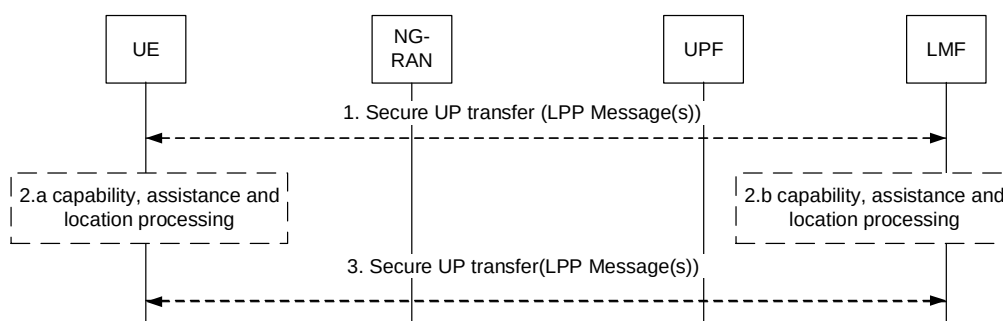
Figure 6.11.4-1: Positioning Procedure over User Plane
