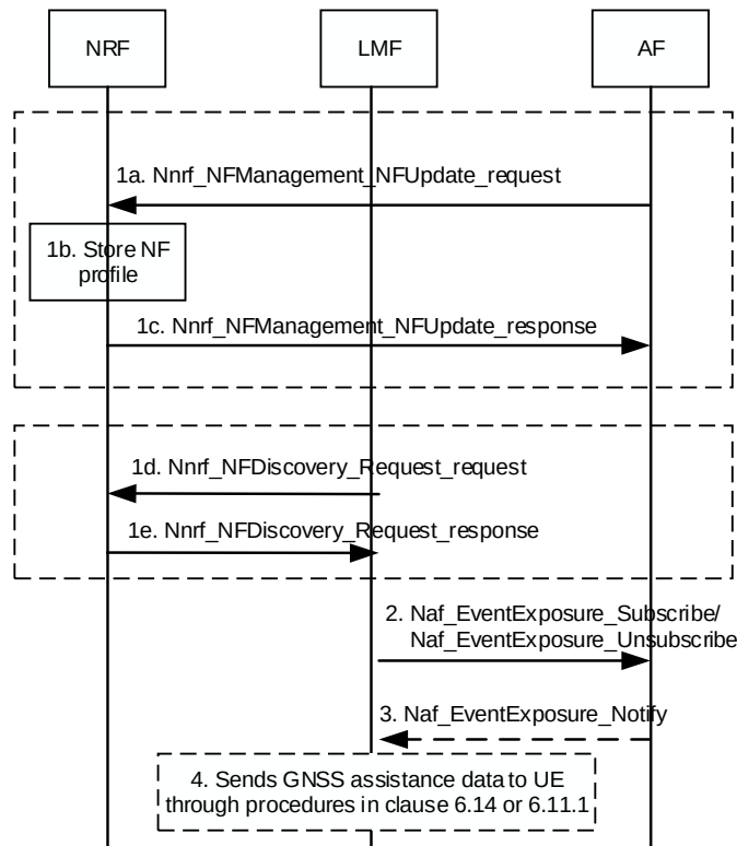
Figure 6.15.2-1: GNSS assistance data collection from trusted AF
