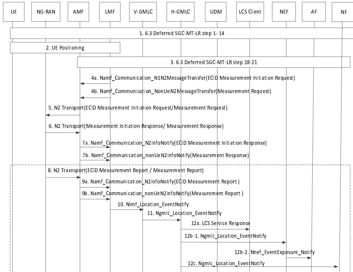
Figure 6.3.5.1-1: Deferred 5GC-MT-LR for Periodic Events based on NRPPa Periodic Measurement
