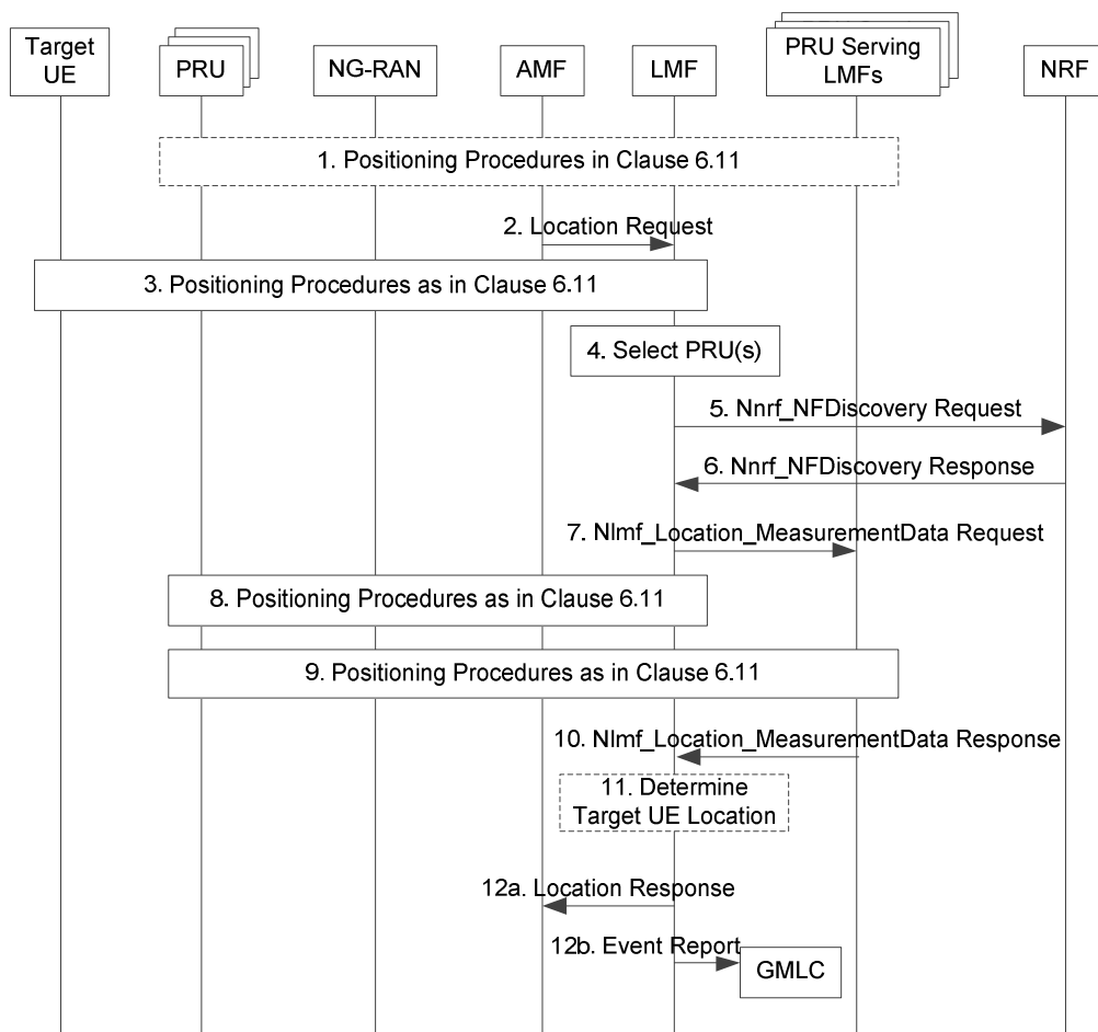
Figure 6.17.4-1: Location of a target UE using PRUs
