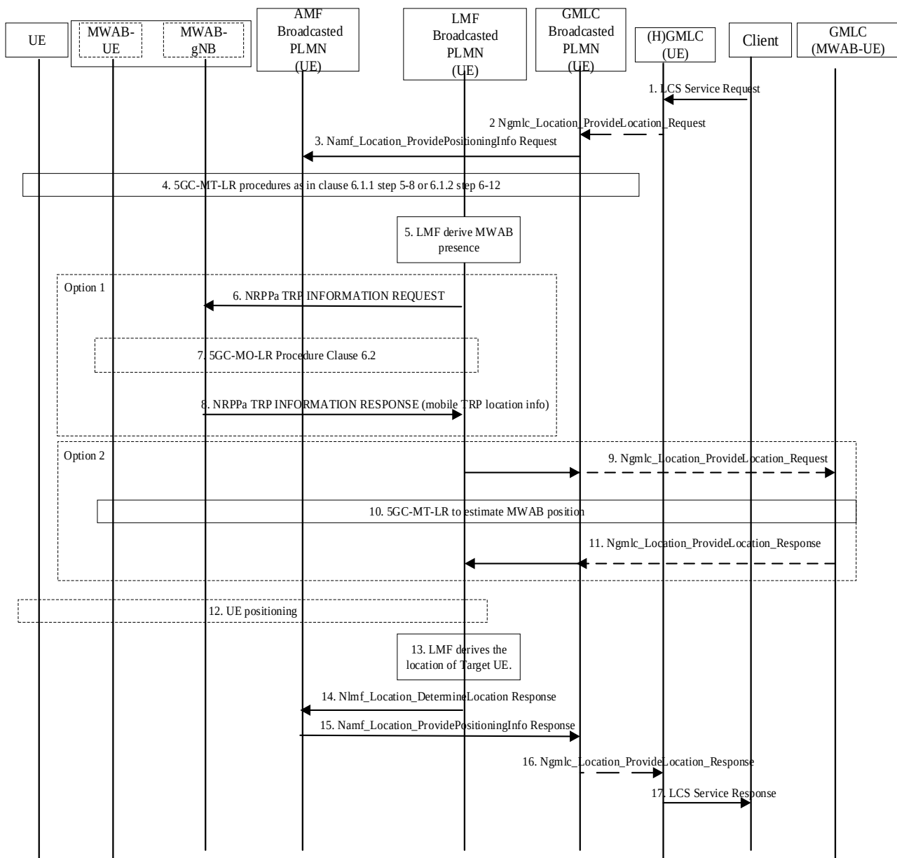
Figure 6.1.5-1: 5GC-MT-LR procedure involving MWAB
