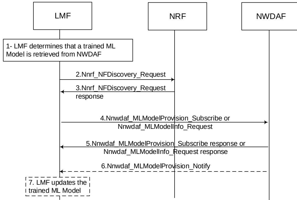
Figure 6.22.5-1: Retrieval of trained ML model(s) for LMF-based AI/ML positioning from NWDAF
