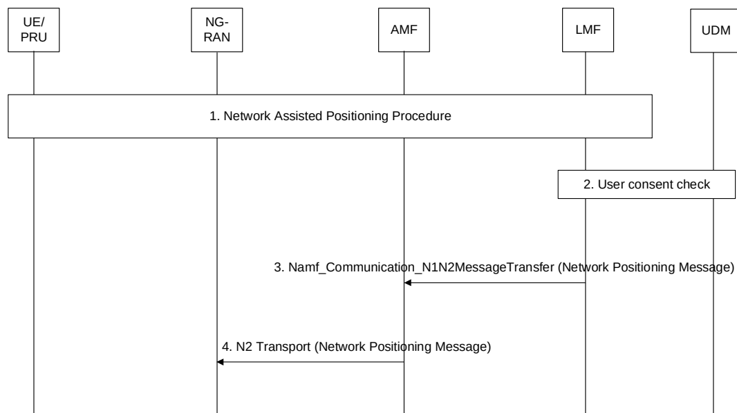
Figure 6.23.2-1: Data Collection for NG RAN-sided models for UEs under positioning
