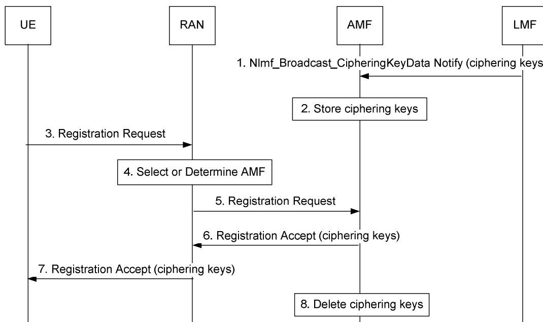
Figure 6.14.2-1: Delivery of Ciphering Keys to UEs for Broadcast Assistance Data
