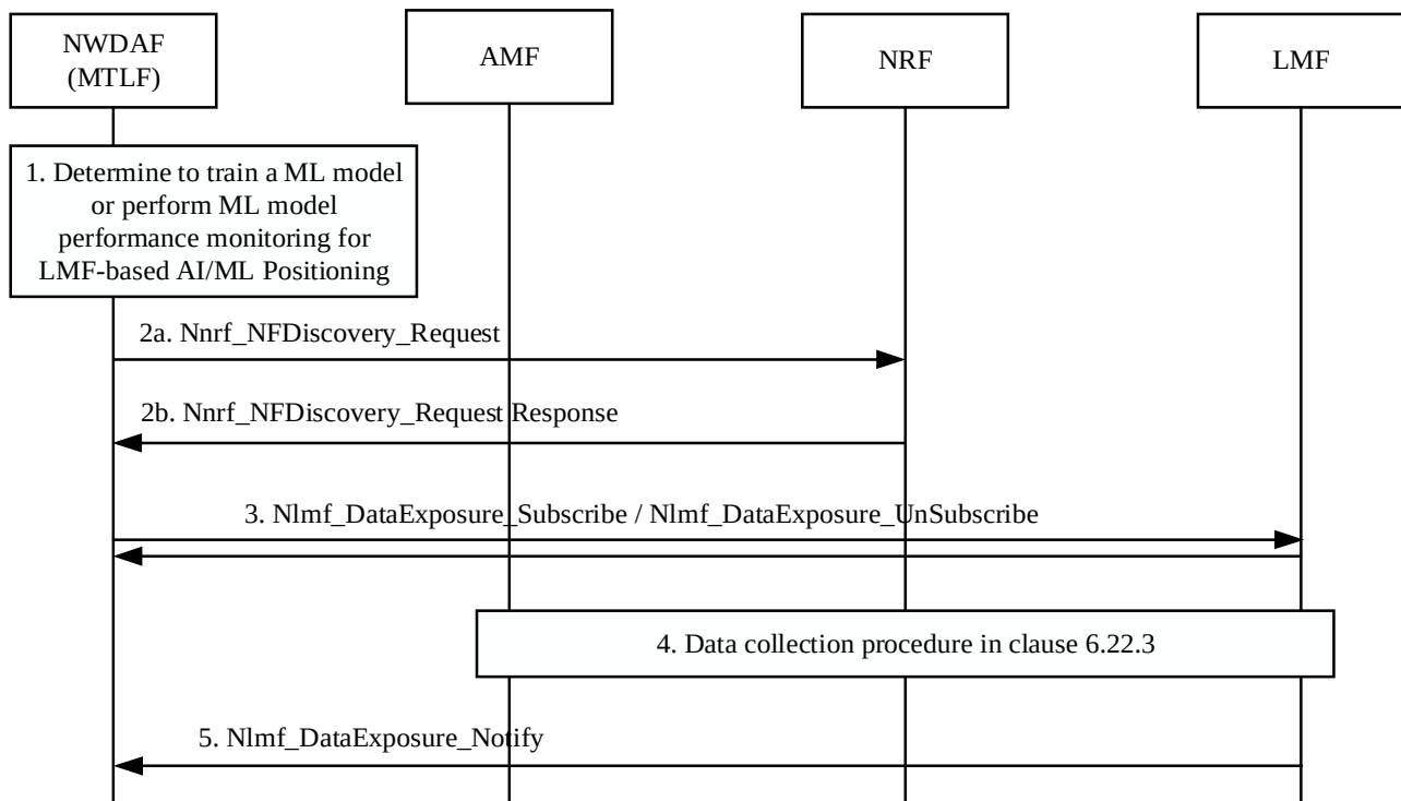
Figure 6.22.4-1: Procedure of input data collection from LMF
