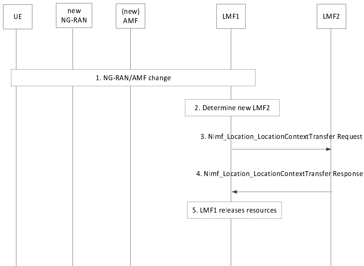
Figure 6.4.1-1: Change of serving LMF for Periodic Events based on NRPPa Periodic Measurement
