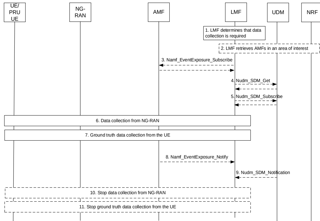
Figure 6.22.3-1: Data collection by LMF to train the AI/ML based positioning model using NG-RAN measurements
