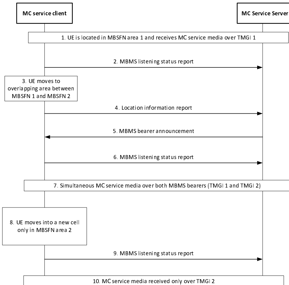
Figure 10.7.3.7.2-2: Service continuity when moving from one MBSFN to another
