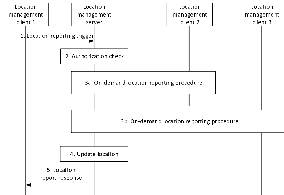
Figure 10.9.3.8.1-1: One-time location information report for shared functional alias
