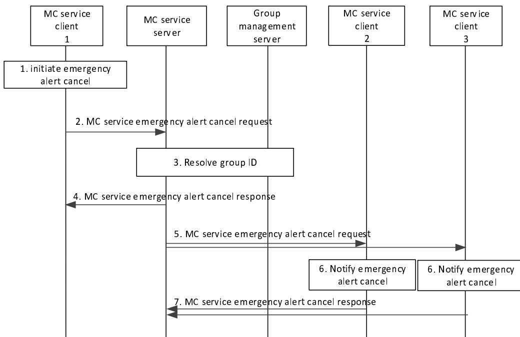
Figure 10.10.1.2.2-1 MC service emergency alert cancel
