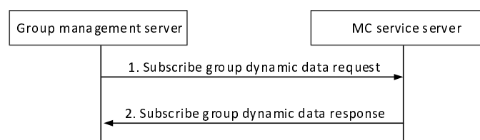
Figure 10.1.5.6.3-1: Subscription for group affiliation status
