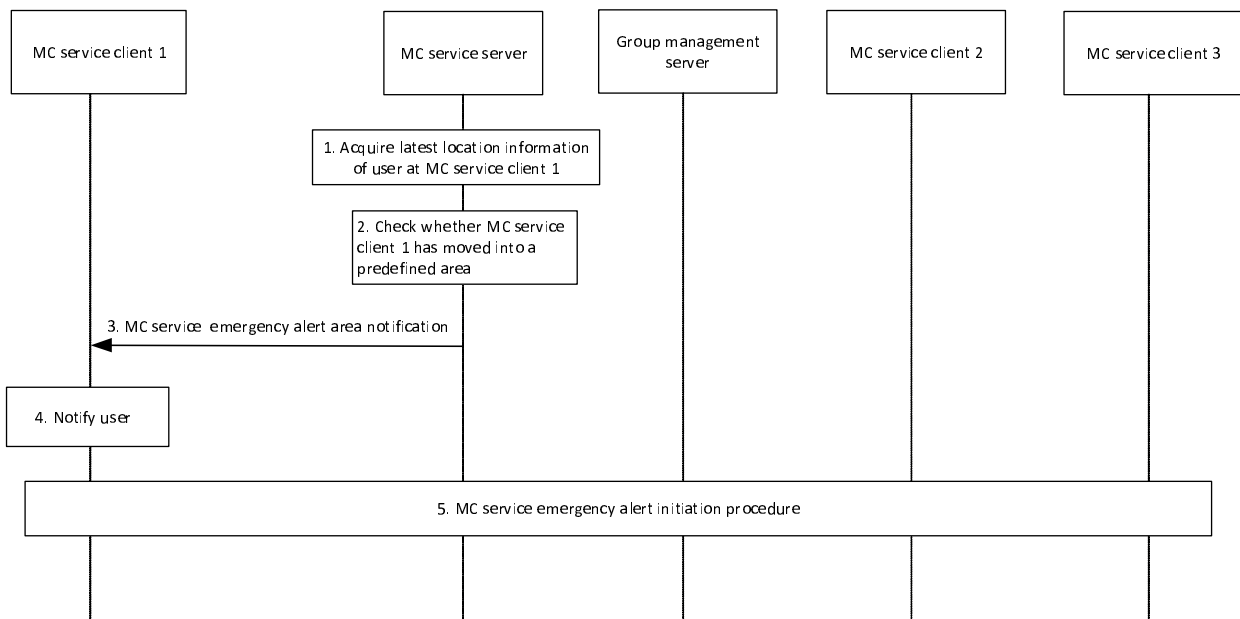
Figure 10.10.1.2.3-1 Entering MC service emergency alert area
