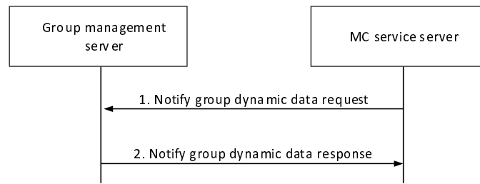
Figure 10.1.5.6.3-2: Notification of group affiliation status
