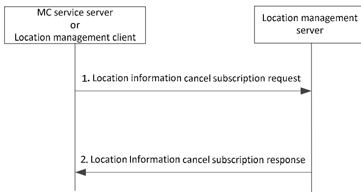
Figure 10.9.3.7-1: Location information cancel subscription request procedure
