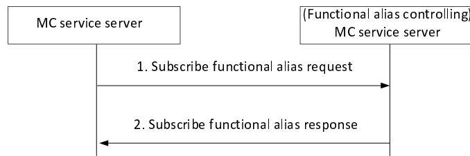
Figure 10.13.10.2-1: Subscription for functional alias
