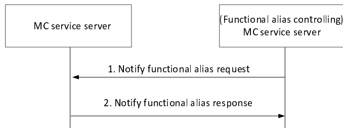
Figure 10.13.10.3-1: Notification for the functional alias
