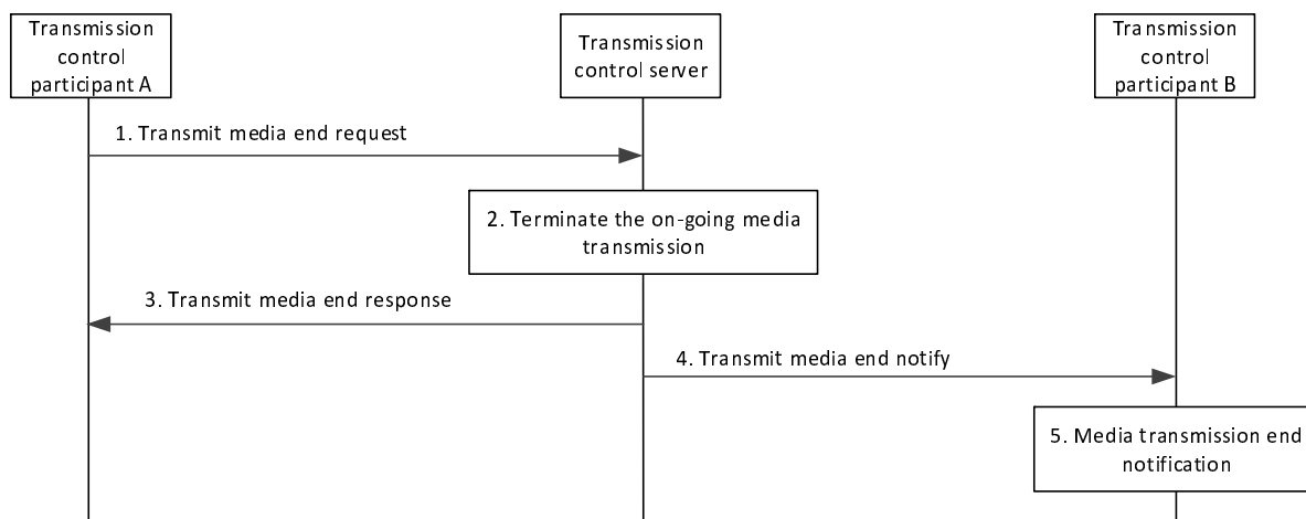
Figure 7.7.1.3.6.1-1: End a media transmission by an MCVideo user
