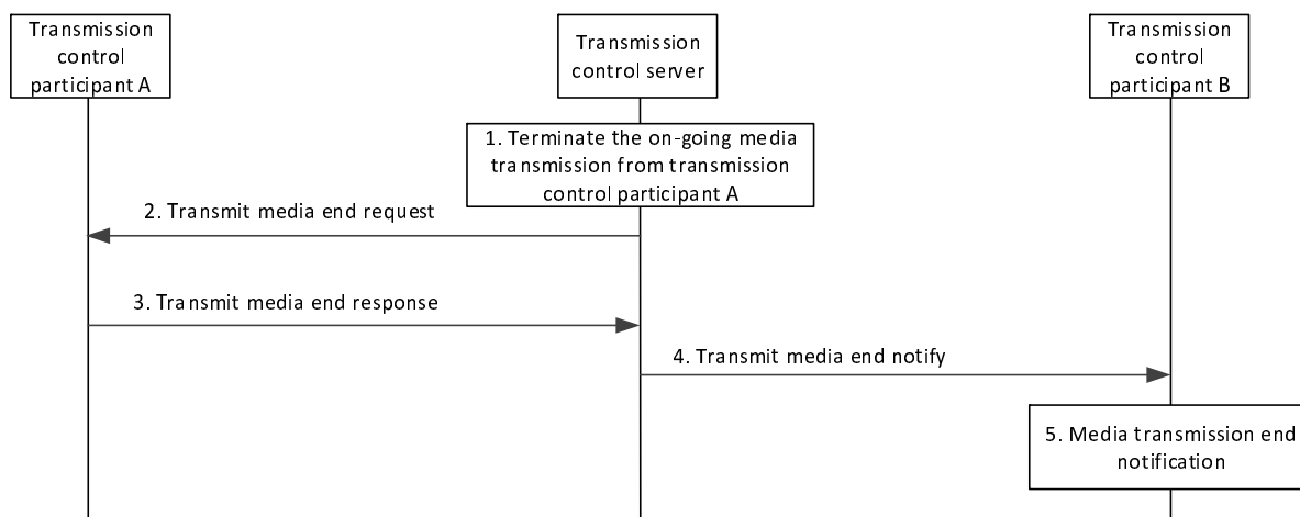
Figure 7.7.1.3.6.2-1: End a media transmission by the transmission control server
