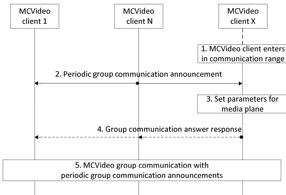
Figure 7.1.3.4.2-1: Passive join to MCVide group communication
