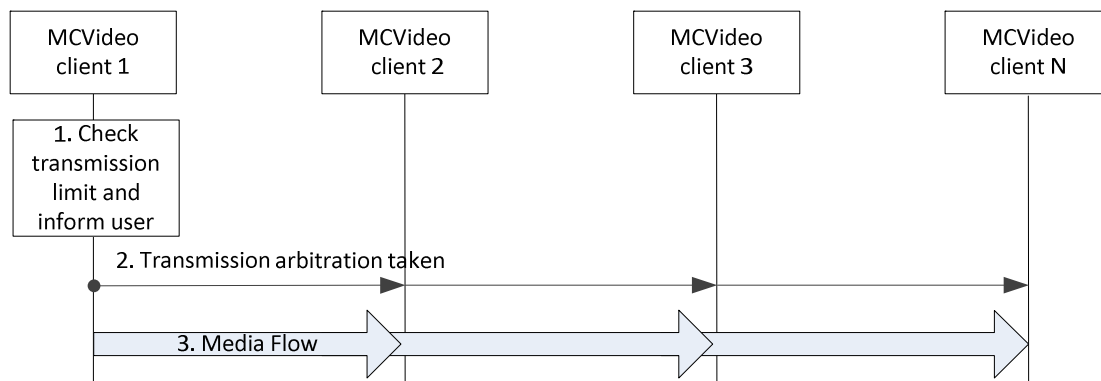
Figure 7.7.2.3a-1: Initializing transmission control, self arbitration case
