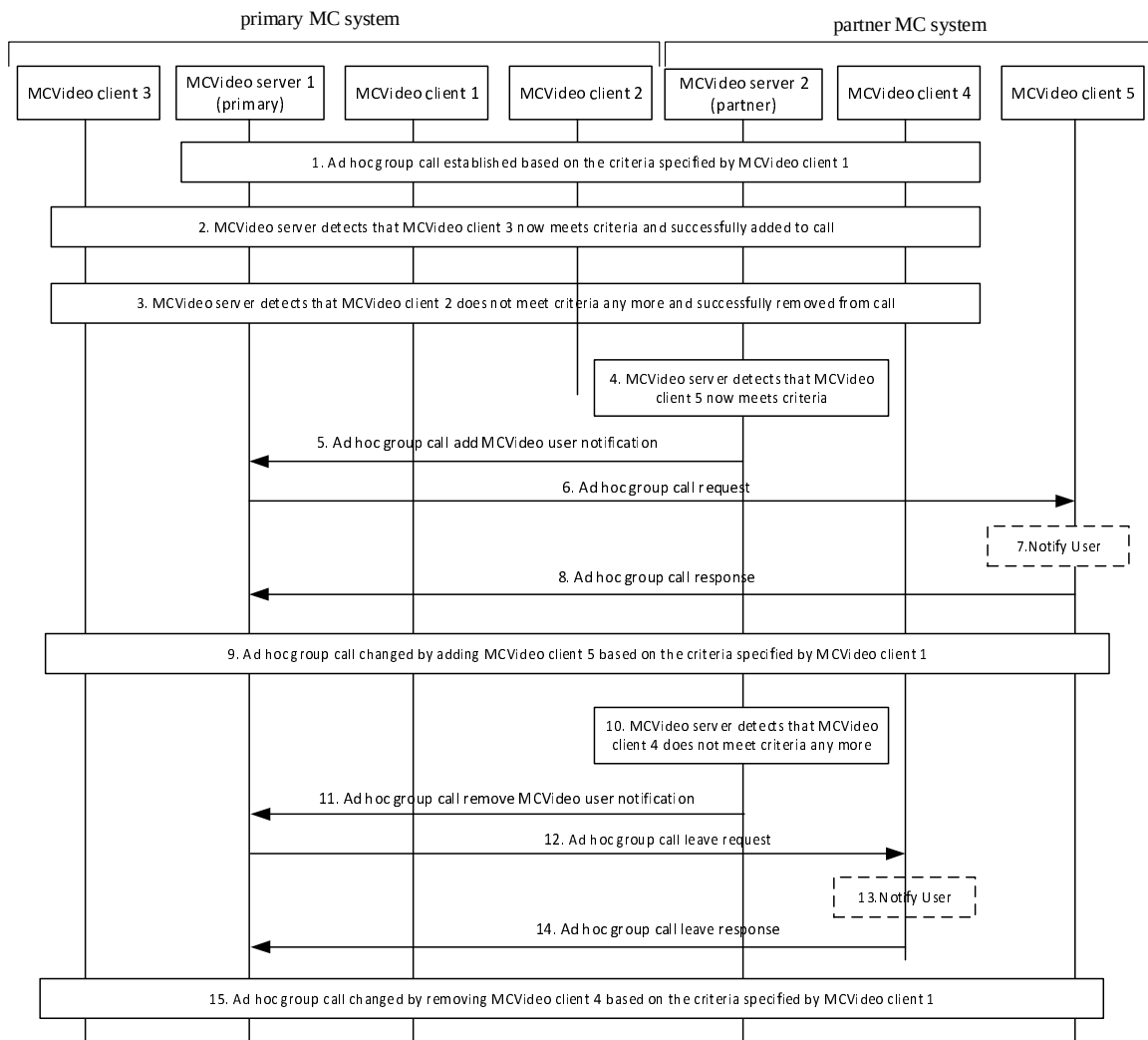
Figure 7.19.3.2.2-1: Modification of ad hoc group call participants by the MCVide server
