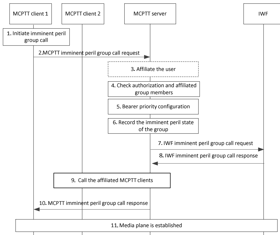
Figure 10.6.3.2-1: Imminent peril group call initiated by a MCPTT user to an interworking group defined in the MCPTT system
