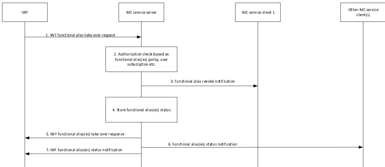
Figure 10.14.3.5-1: IWF functional alias taking over procedure within an MC system
