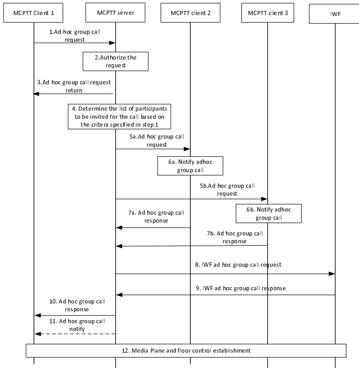
Figure 10.17.3.1-1: Ad hoc group call setup initiated by an MCPTT user in the MCPTT system
