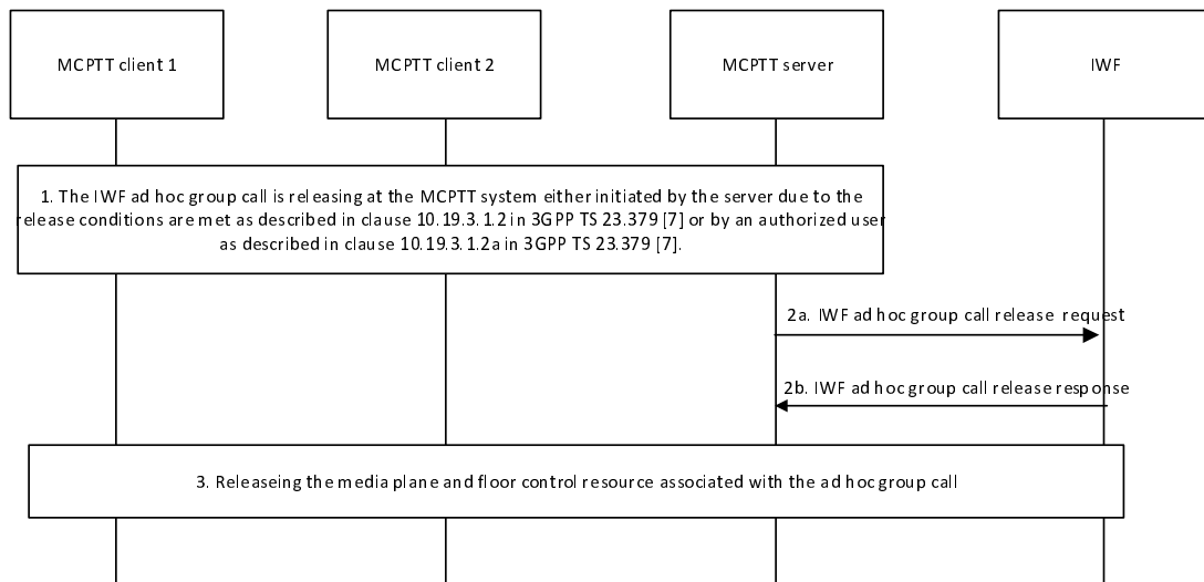
Figure 10.17.3.3-1: Release IWF ad hoc group call by the MC system
