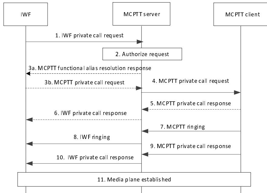
Figure 10.4.3.2-1: Private call setup in manual commencement mode, initiated by an LMR user
