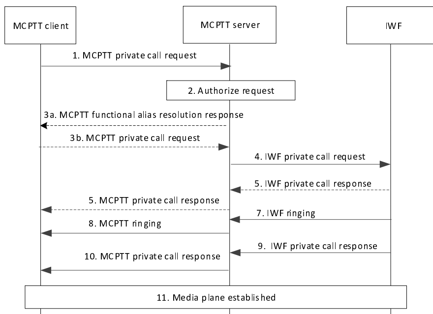
Figure 10.4.3.1-1: Private call setup in manual commencement mode – initiated by an MCPTT user
