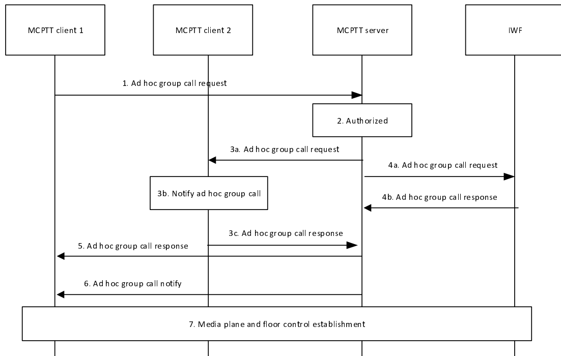
Figure 10.17.3.5-1: Ad hoc group call setup initiated by an MCPTT user in the MCPTT system
