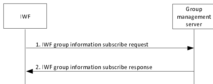
Figure 10.2.3.6-1: Subscription from the IWF to the MC system for MC service group configuration
