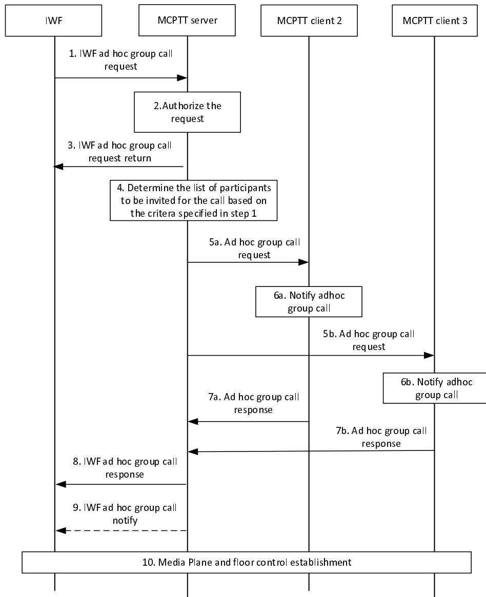
Figure 10.17.3.2-1: Ad hoc group call setup initiated by an LMR user in the MCPTT system
