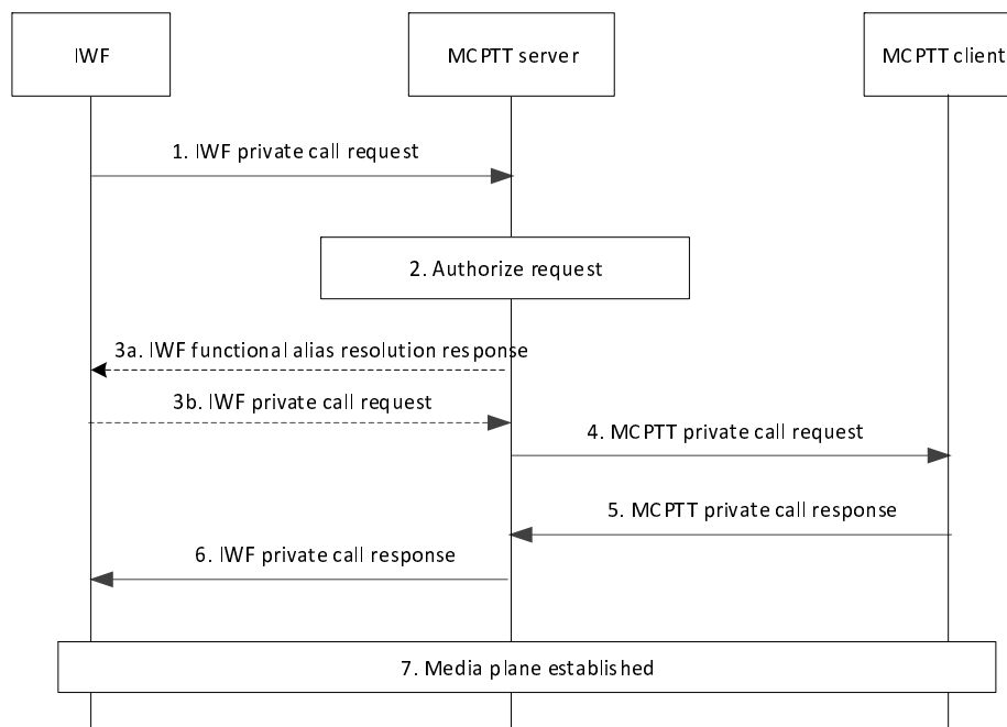
Figure 10.4.2.2-1: Private call setup in automatic commencement mode, initiated by an LMR user
