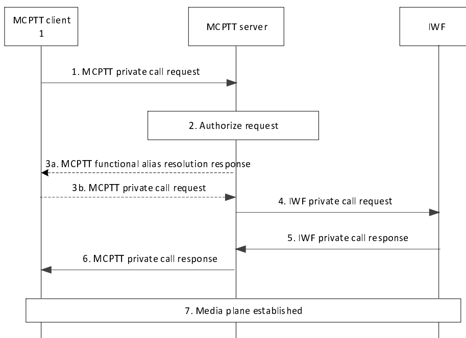
Figure 10.4.2.1-1: Private call setup in automatic commencement mode, initiated by an MCPTT user
