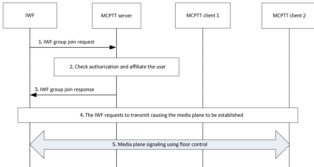
Figure 10.3.5.3-1: LMR user initiated chat group call in an interworking group defined in the MCPTT system
