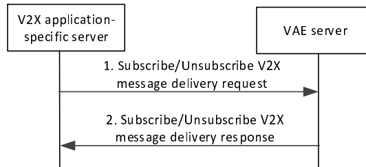
Figure 9.4.6-1: Procedure for subscription to message delivery
