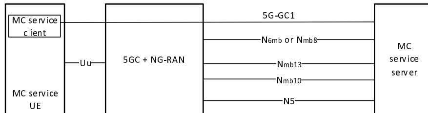
Figure 4.7.3.3-1: Architectural view of a mission critical system when using MBS without optional NEF entity and its associated interfaces
