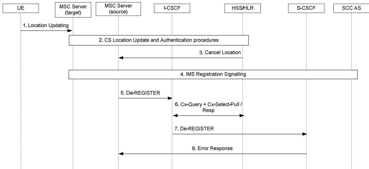
Figure 7.2.1.5-1: IMS Deregistration via CS Access by source MSC Server enhanced for ICS when moving to a target MSC Server enhanced for ICS
