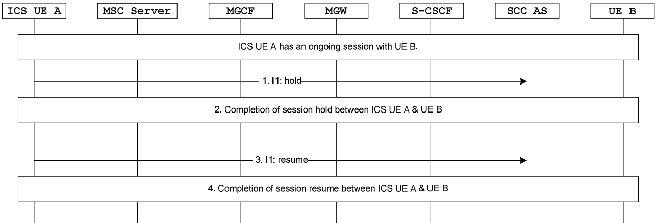
Figure 7. 6.1.2.3.4-1: IMS communication Hold and Resume by ICS UE
