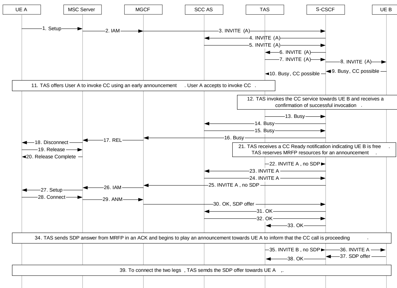
Figure 7.6.3.10.2-1: IMS Communication Completion via MSC Server not enhanced for ICS
