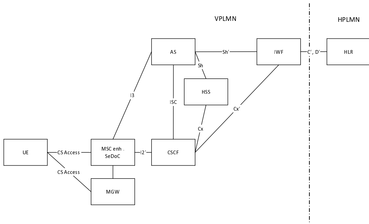
Figure H.5.2.1-1: Architecture for inbound roamer support
