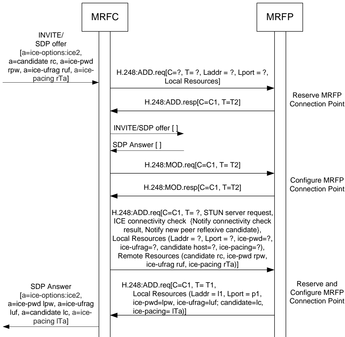
Figure 6.2.18.2.1: Procedure for interactive connectivity establishment using full ICE towards the offerer
