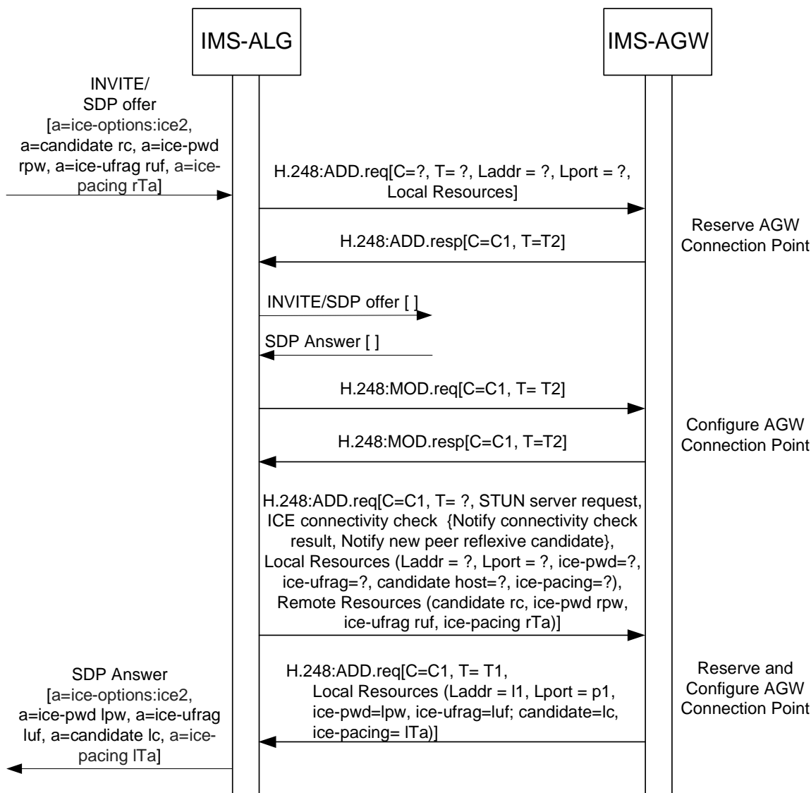
Figure 6.2.17.2.1: Procedure for interactive connectivity establishment using full ICE towards the offerer
