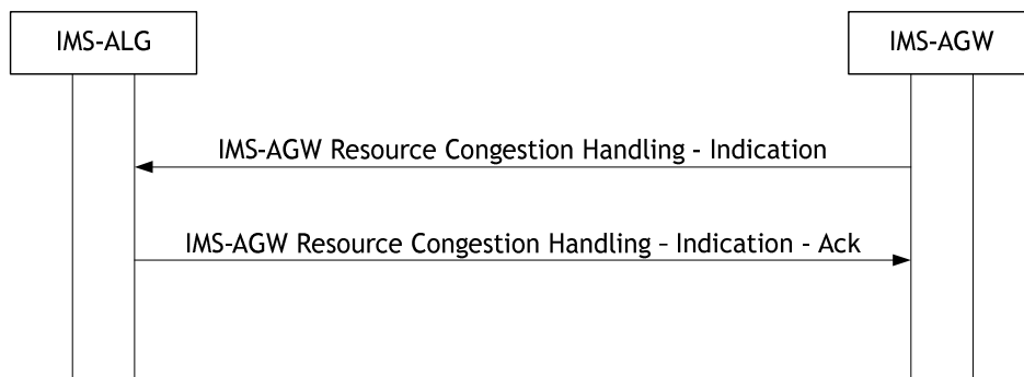
Figure 6.1.12.1: IMS-AGW Resource Congestion Handling – Indication
