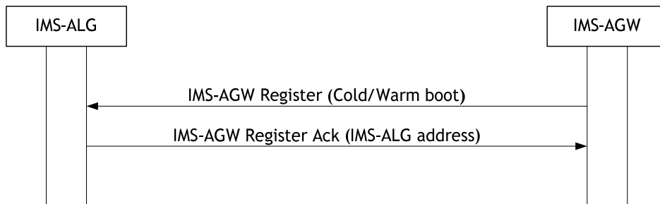
Figure 6.1.4.2 IMS-AGW Registration
