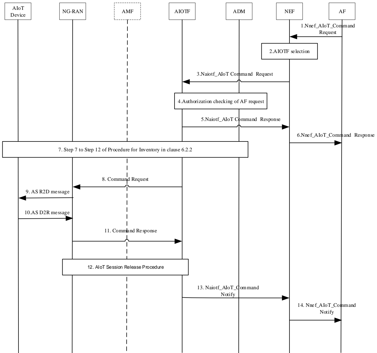
Figure 6.2.3-1: Command Procedure
