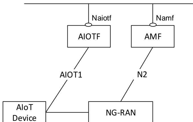
Figure 4.2.2.3-1: NG-RAN - AIOT Indirect connectivity Architecture
