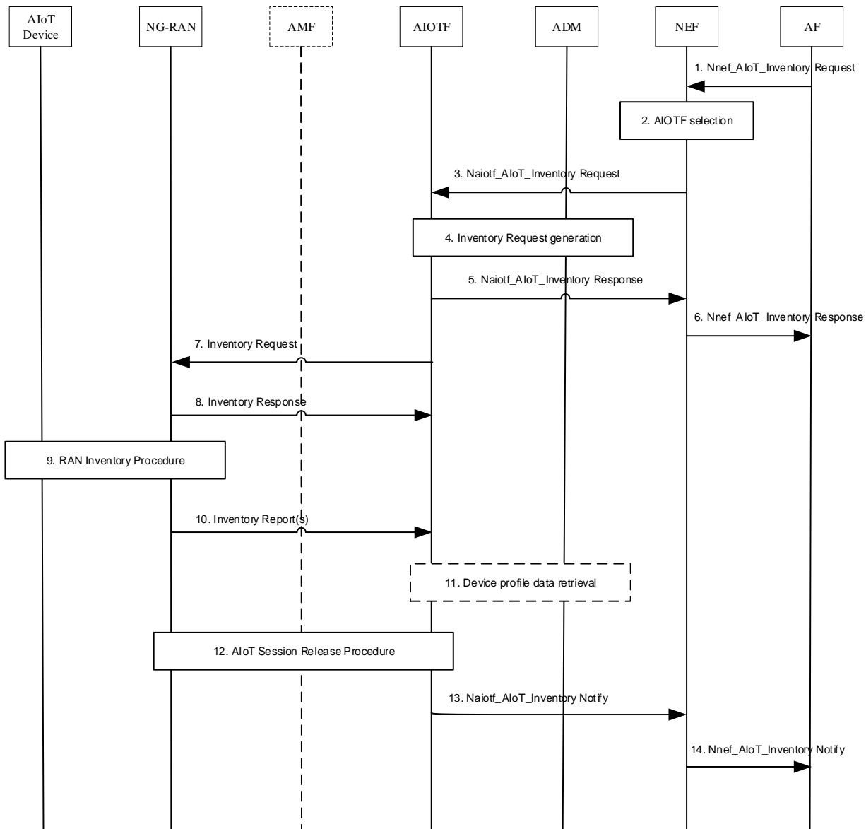
Figure 6.2.2-1: Inventory Procedure
