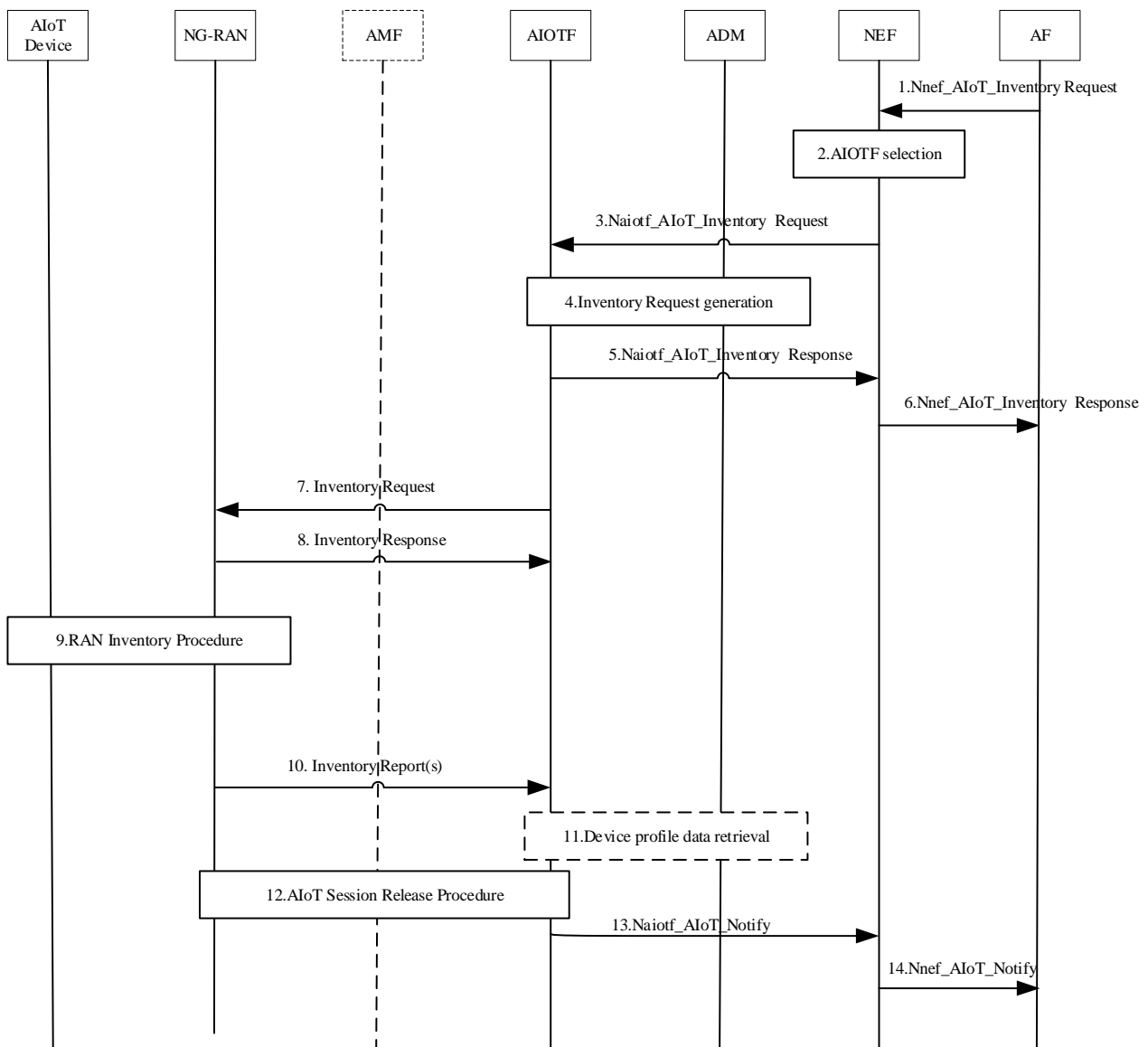
Figure 6.2.2-1: Inventory Procedure
