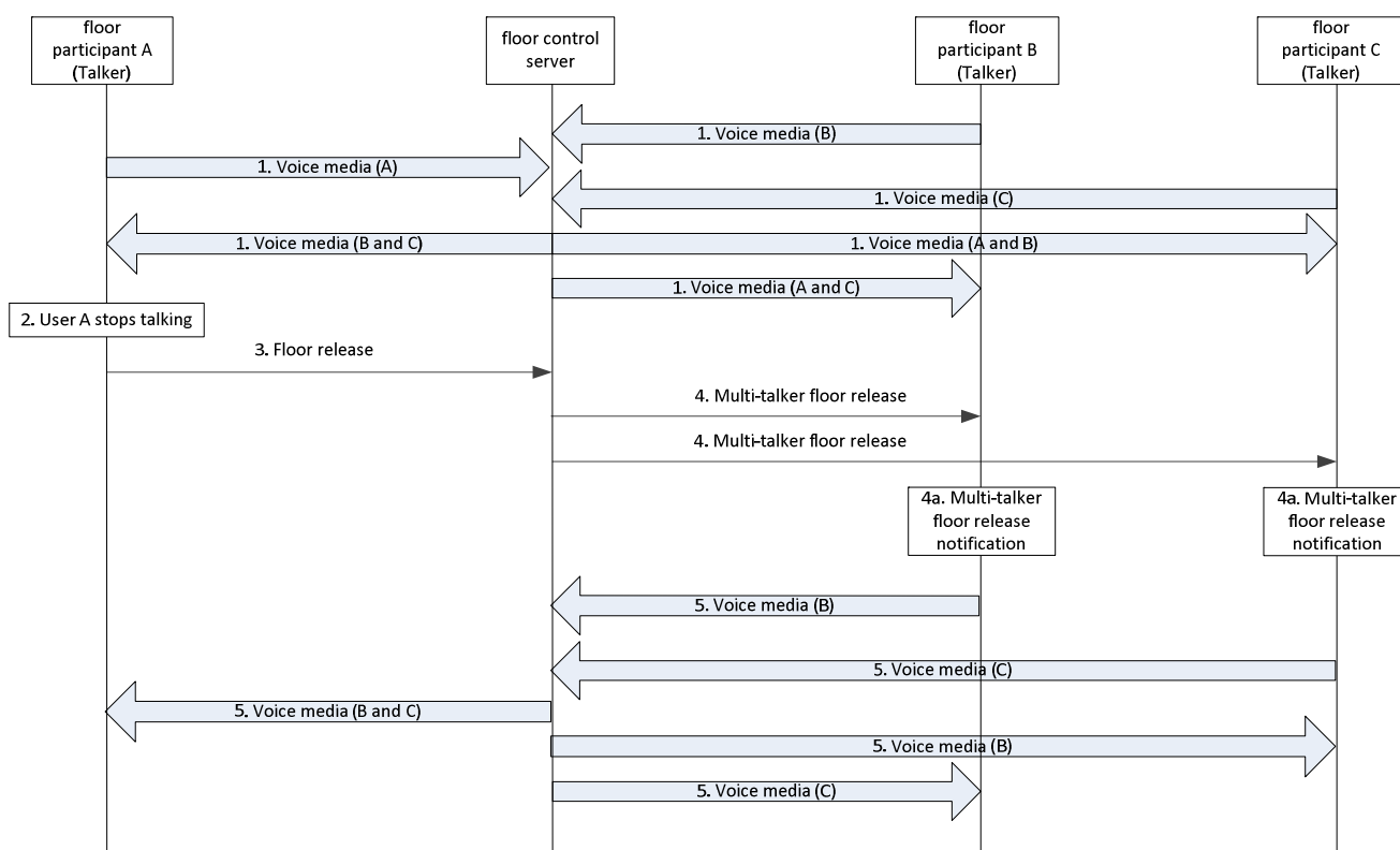
Figure 10.9.1.3.2.4-1: Floor release during an MCPTT session
