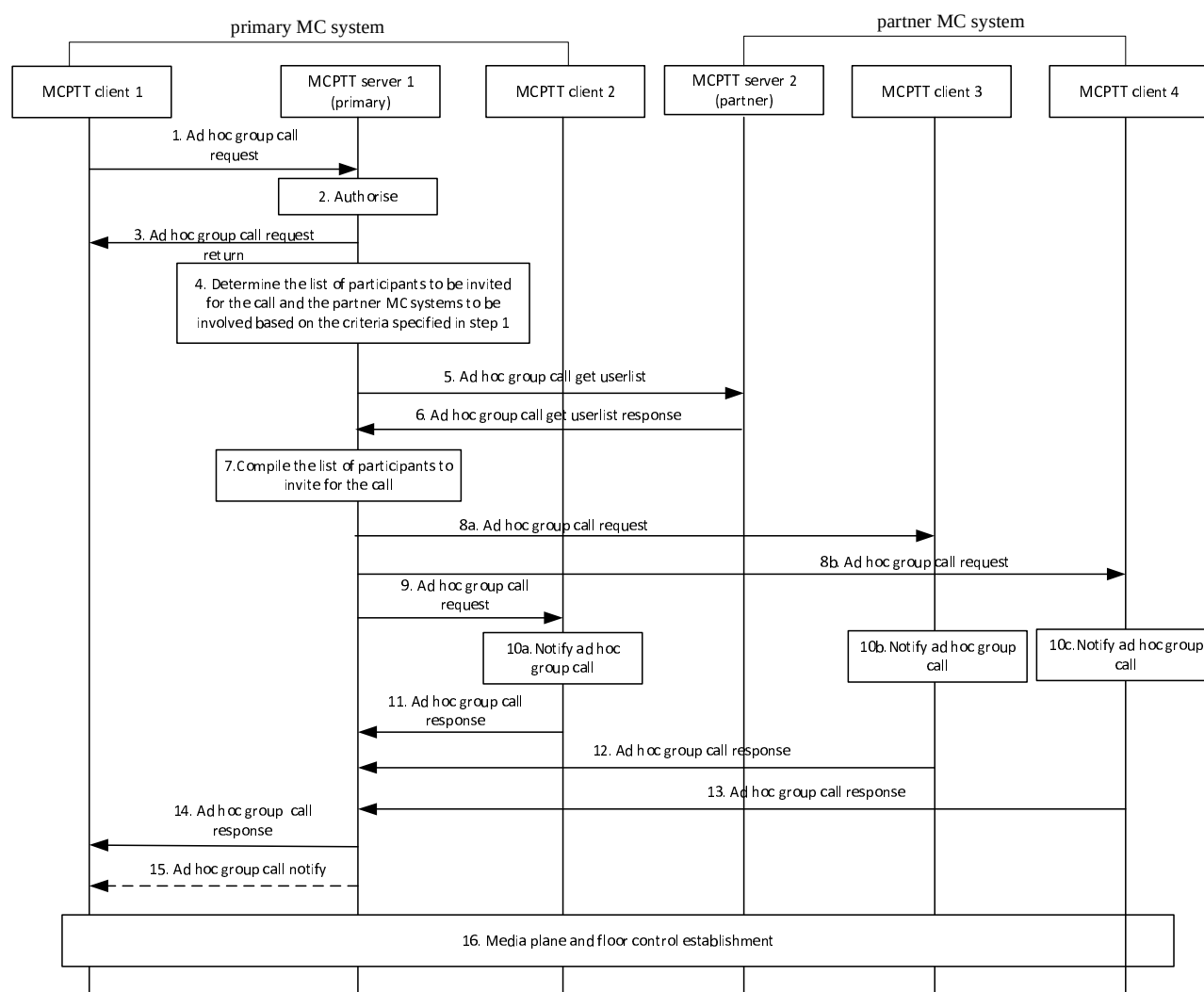
Figure 10.19.3.2.3-1: Ad hoc group call setup involving multiple MCPTT systems
