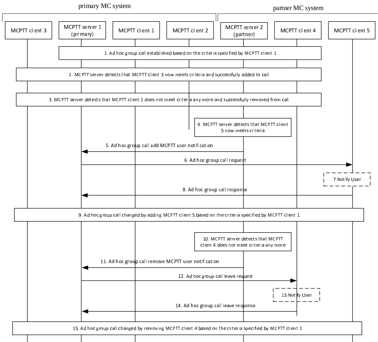
Figure 10.19.3.2.4-1: Modification of ad hoc group call participants by the MCPTT server
