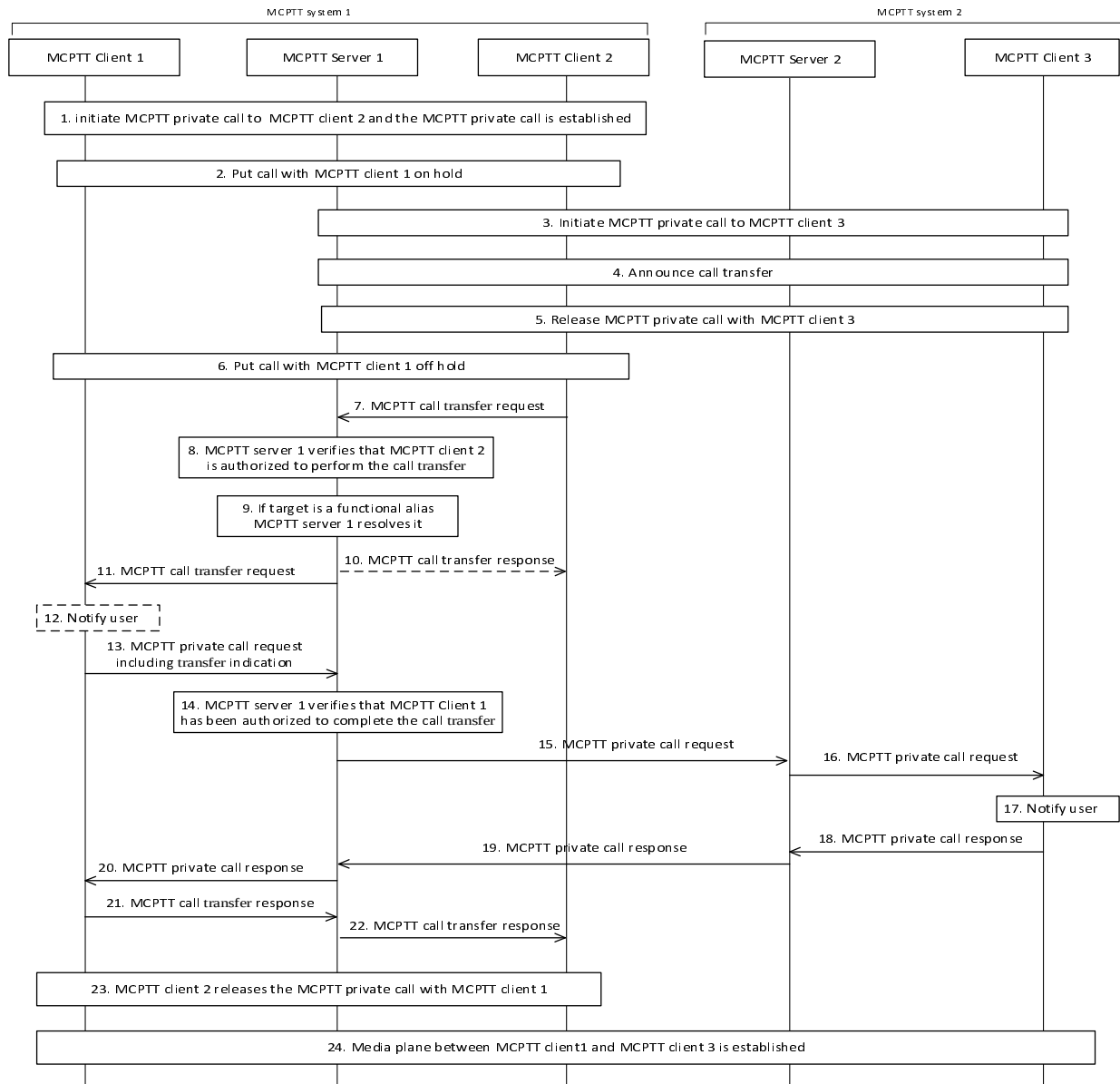
Figure 10.7.6.2.3-1: MCPTT private call announced transfer with target in partner MCPTT system
