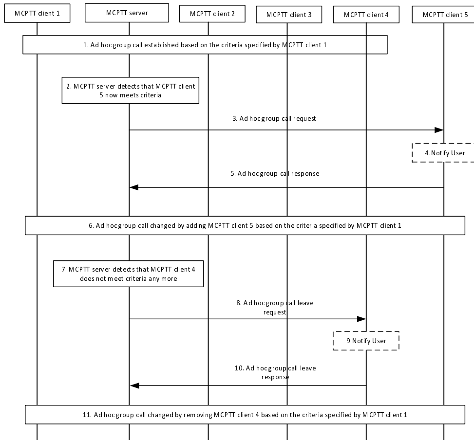
Figure 10.19.3.1.5-1: Modification of ad hoc group call participants by the MCPTT server
