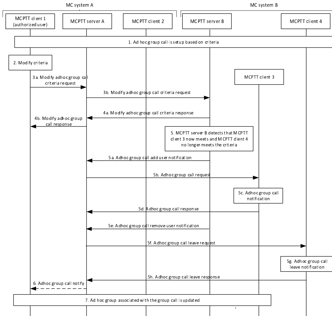
Figure 10.19.3.2.7-1: Modifying the criteria for determining the participants during an ongoing ad hoc group call between multiple MC systems
