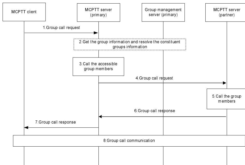
Figure 10.6.2.4.1.1.1-1: Group call setup involving non-broadcast temporary groups from multiple MCPTT systems (originating)
