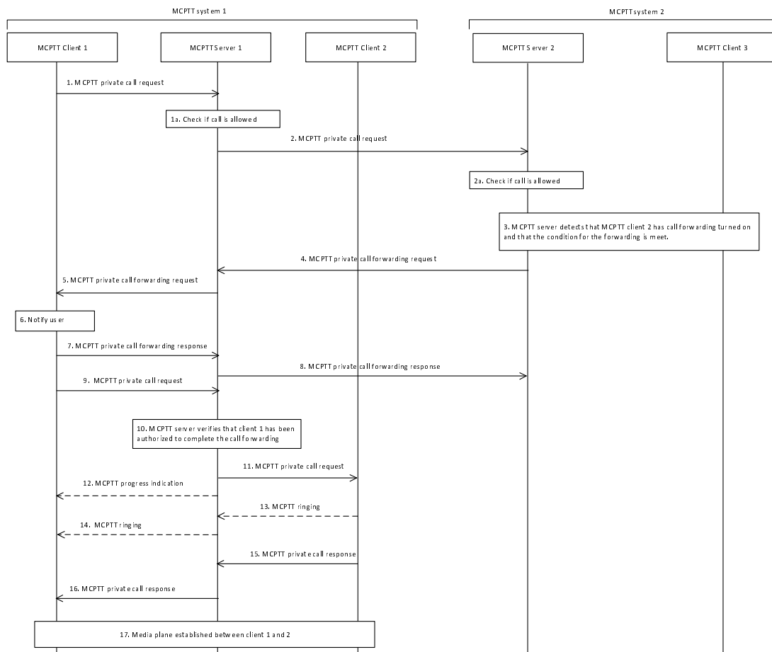
Figure 10.7.5.2.6-1: Simplified private call setup with MCPTT private calls forwarding in manual commencement mode with forwarding in the partner MCPTT systems
