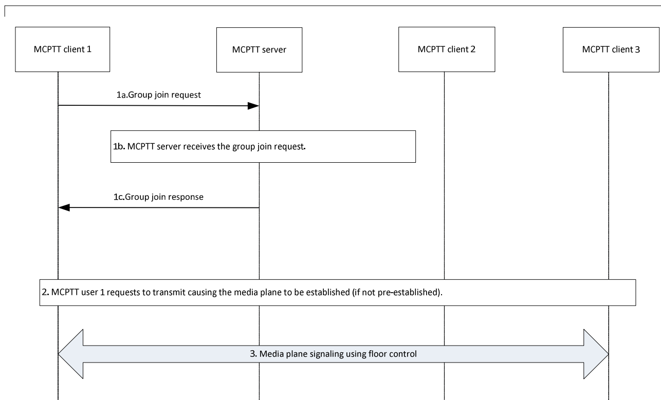
Figure 10.6.2.3.1.2.2-1: MCPTT chat group call
