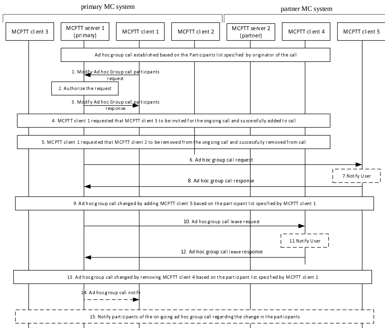
Figure 10.19.3.2.6-1: Modification of ad hoc group call participants by an authorized user
