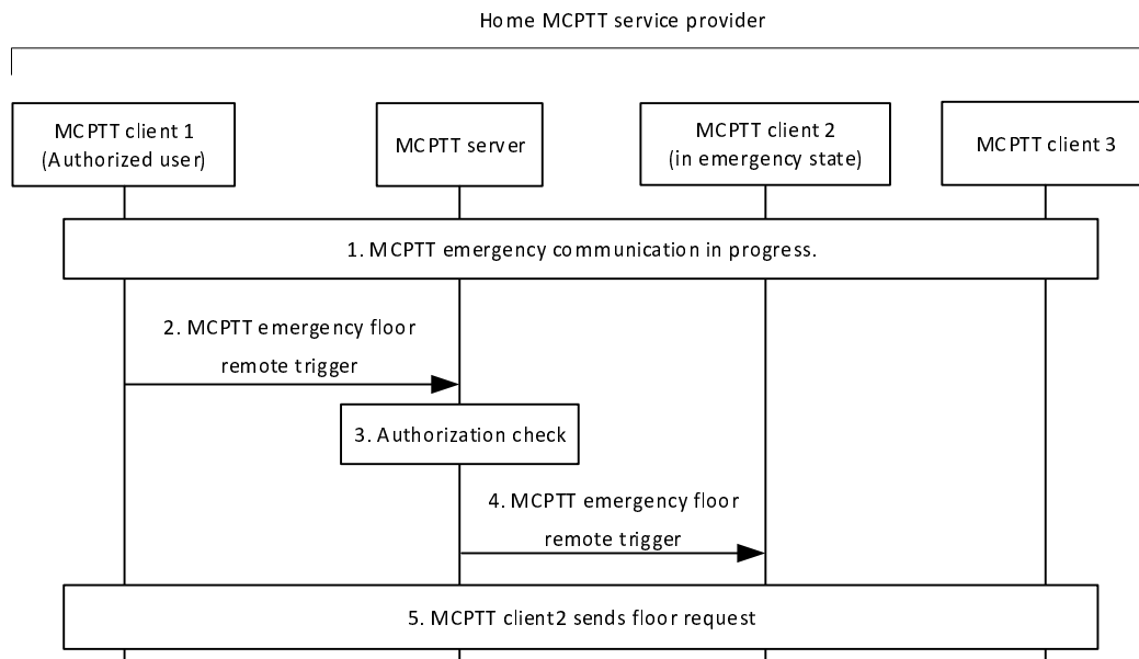
Figure 10.6.2.6.4-1: MCPTT emergency floor remote trigger
