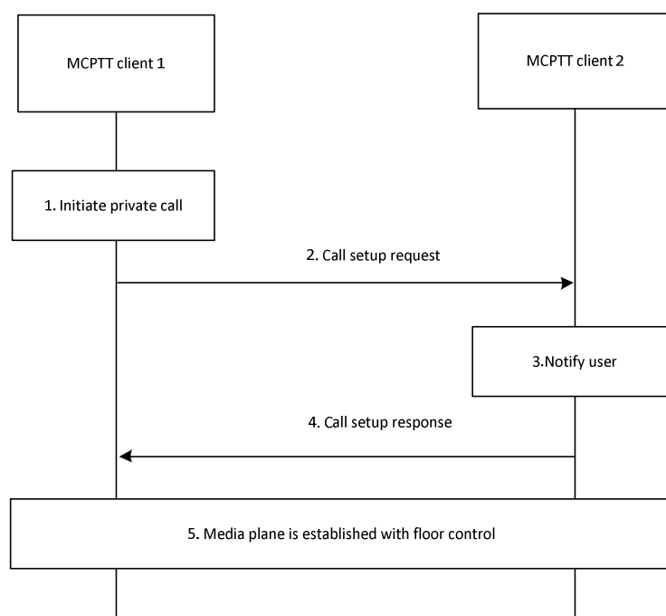
Figure 10.7.3.3-1: Private call setup in automatic commencement mode
