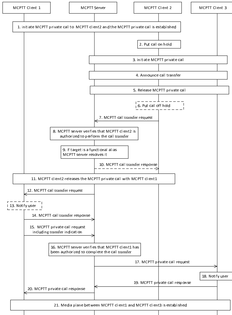
Figure 10.7.6.2.2-1: MCPTT private call announced transfer
