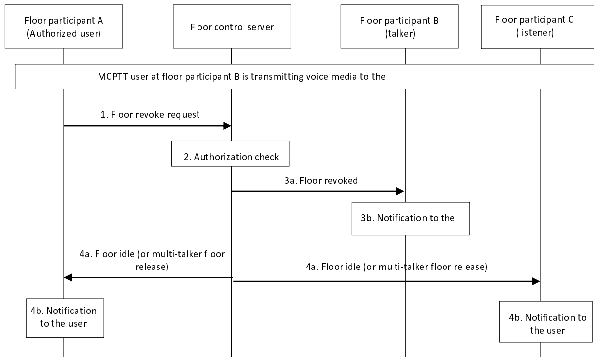
Figure 10.9.1.6.1-1: Floor revoke by authorized user
