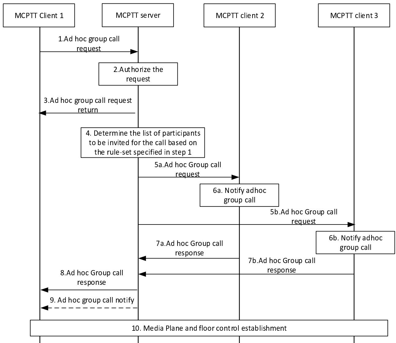
Figure 10.19.3.1.3-1: Ad hoc group call participants determined by MCPTT server
