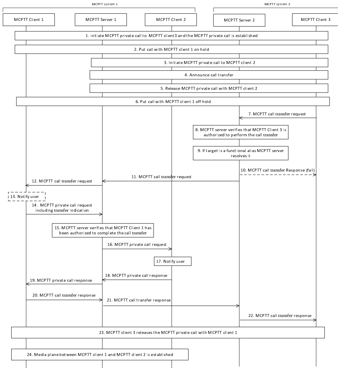
Figure 10.7.6.2.4-1: MCPTT private call announced transfer transferring MCPTT user in partner MCPTT system
