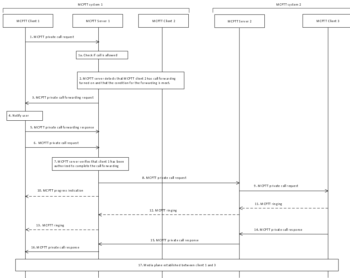
Figure 10.7.5.2.5-1: Simplified private call setup with MCPTT private calls forwarding in manual commencement mode with forwarding target in the partner MCPTT system
