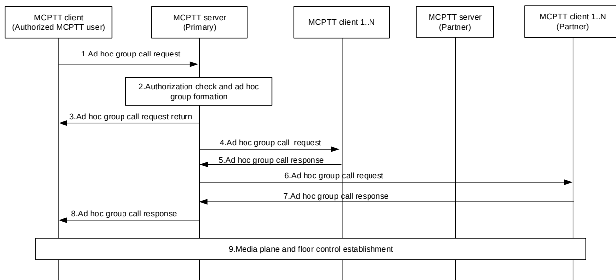
Figure 10.19.3.2.1-1: Ad hoc group call setup
