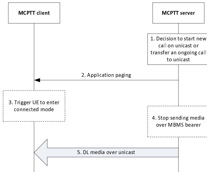
Figure 10.10.6.2-1: Application paging over an MBMS bearer
