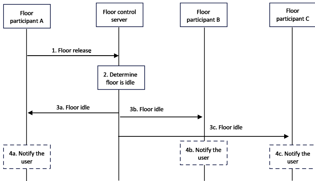
Figure 10.9.1.3.5.1-1: Floor idle during an MCPTT session
