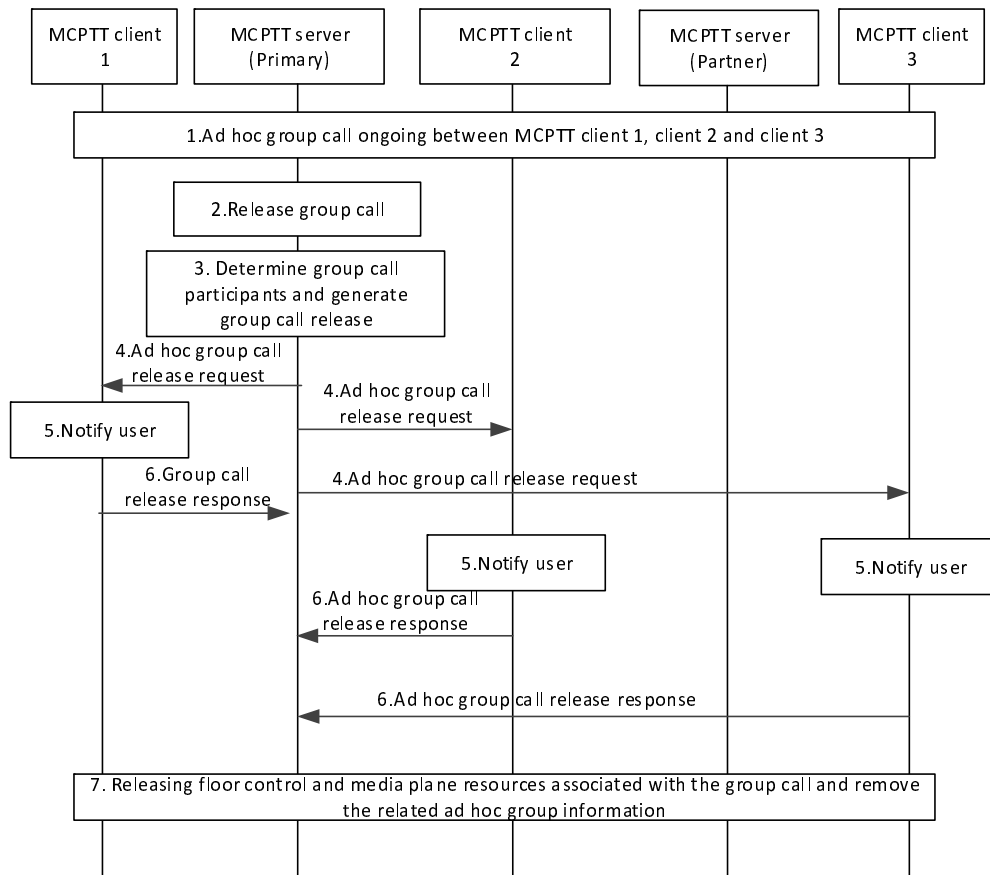
Figure 10.19.3.2.2-1: Ad hoc group call release
