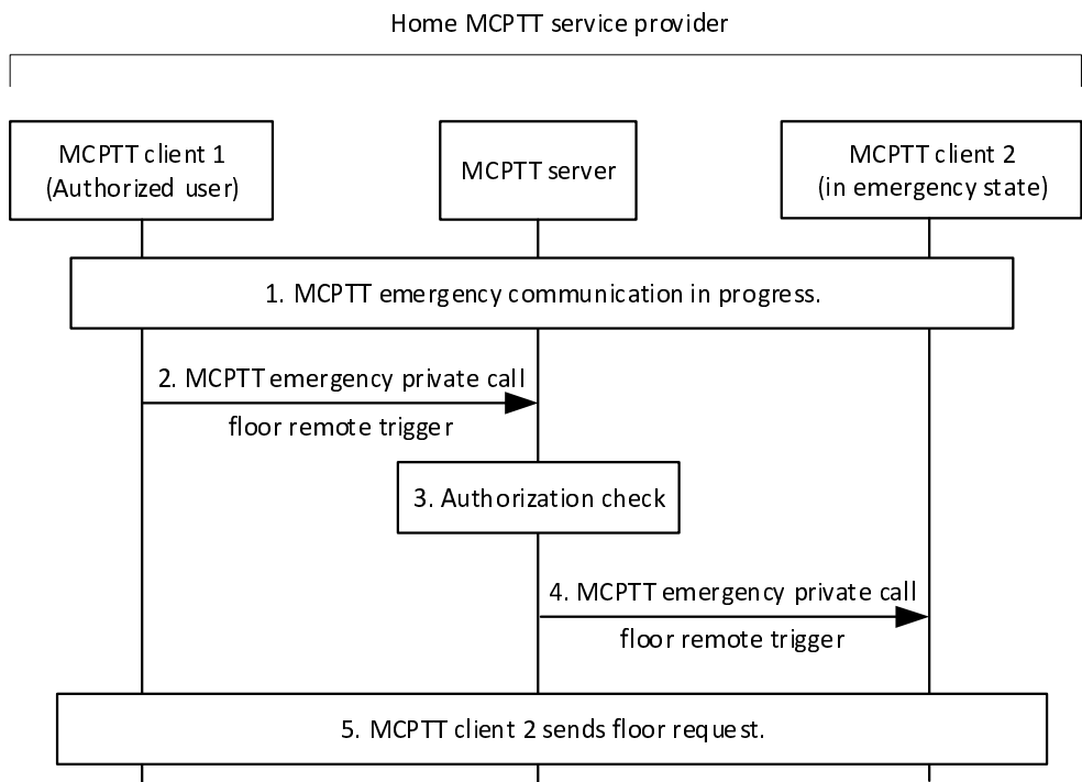
Figure 10.7.2.4.3-1: MCPTT emergency private call floor remote trigger
