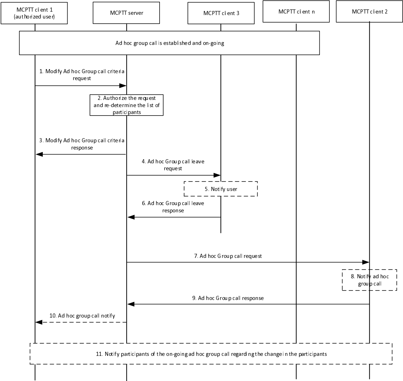
Figure 10.19.3.1.6-1: Modification of ad hoc group call criteria by the authorized user
