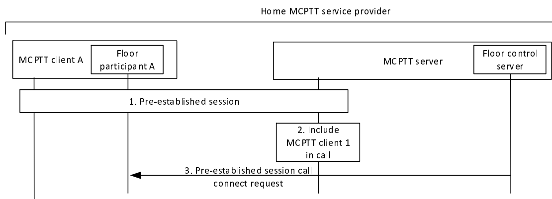
Figure 10.5.3.2.1-1: Connect procedure
