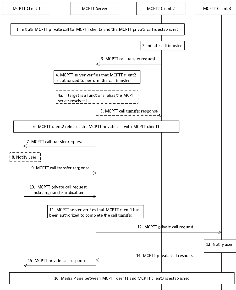
Figure 10.7.6.2.1-1: MCPTT private call unannounced transfer
