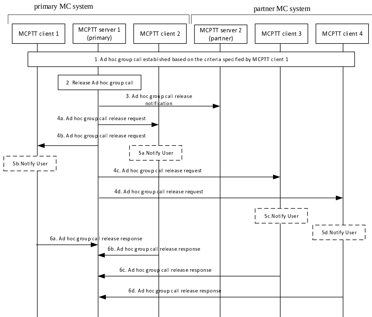
Figure 10.19.3.2.5-1: MCPTT server releases an ad hoc group call and stops the determination of ad hoc group call participants involving multiple MCPTT systems
