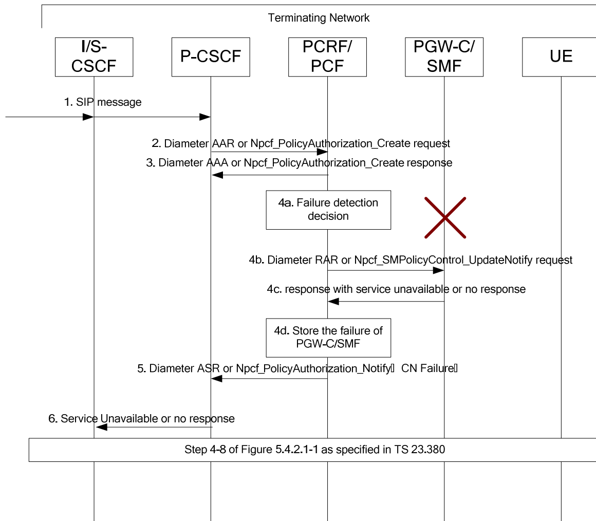
Figure 7.2.3.2-1: P-CSCF receiving EPC/5GC NF failure notification from PCRF/PCF
