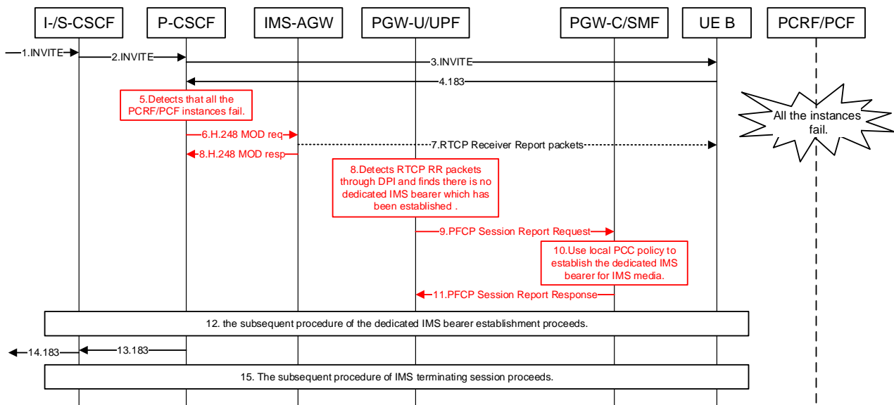
Figure 8.2.4-1: IMS MT procedure of PCRF/PCF bypass
