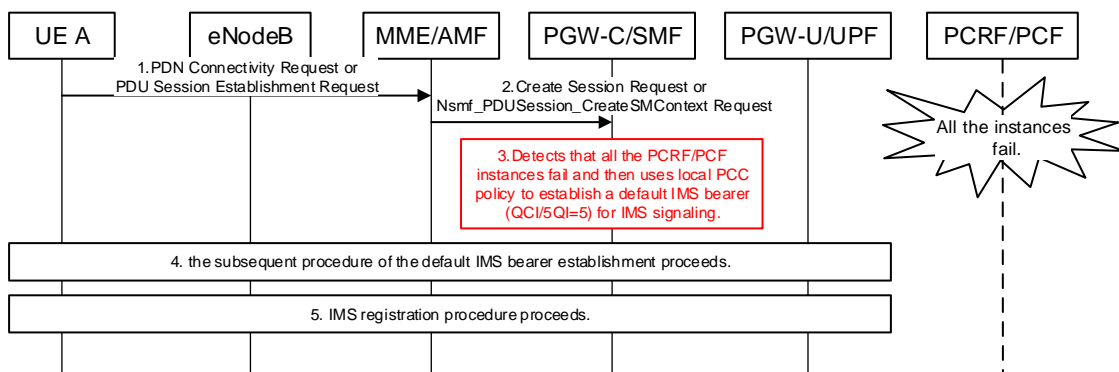
Figure 8.2.2-1: EPS bearer/QoS flow establishment procedure for IMS signalling of PCRF/PCF bypass
