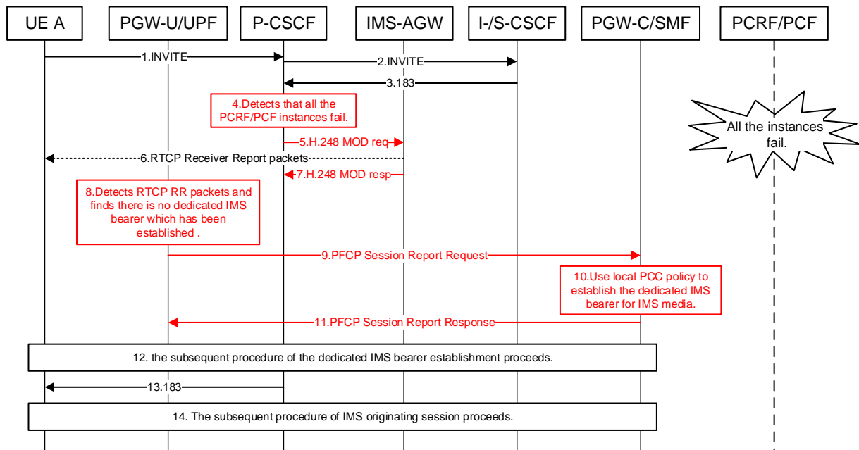
Figure 8.2.3-1: IMS MO procedure of PCRF/PCF bypass
