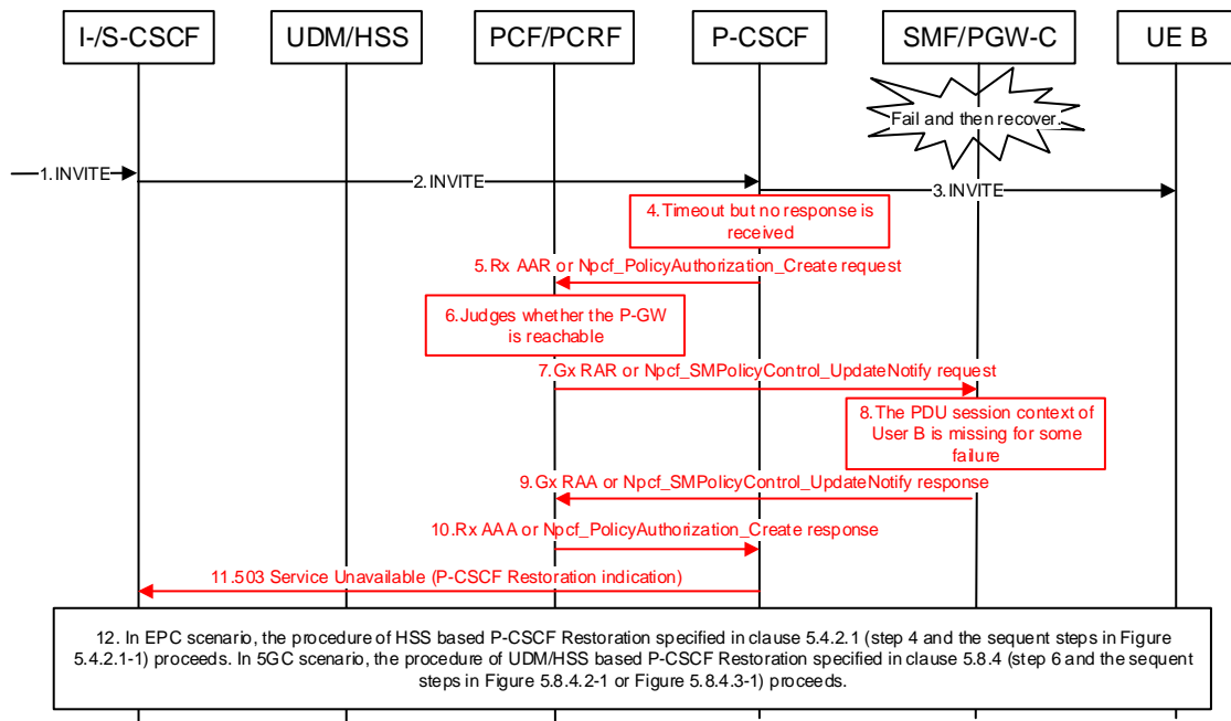
Figure 7.2.2-1: Quick restoration procedure of IMS terminating session
