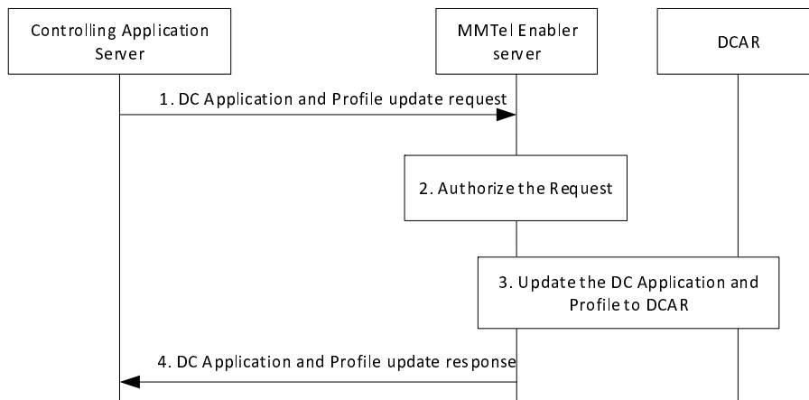
Figure 8.2.3.2-1: DC application and profile update
