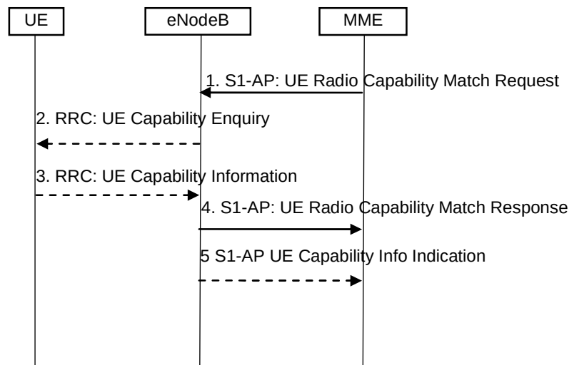
Figure 5.3.14-1: UE Radio Capability Match Request
