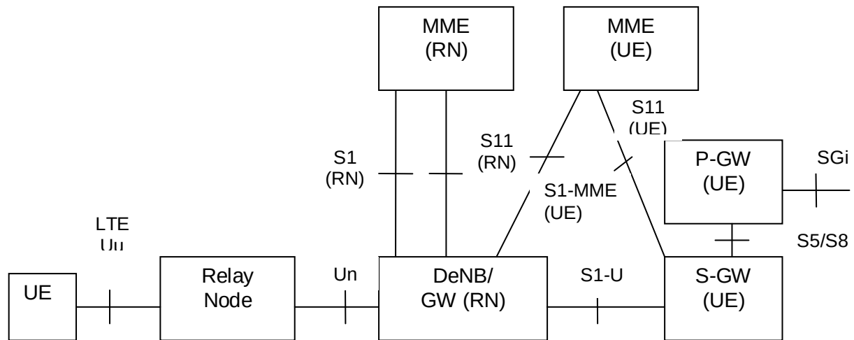
Figure 4.3.20.1-1: Relaying Architecture
