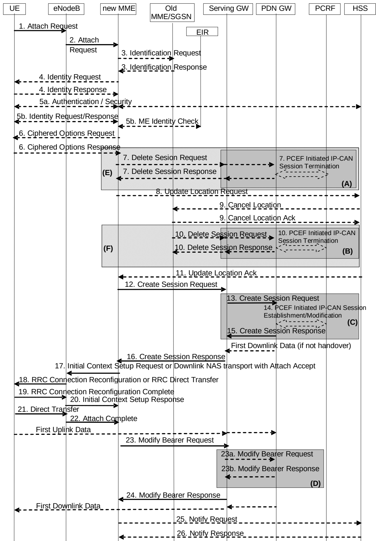
Figure 5.3.2.1-1: Attach procedure
