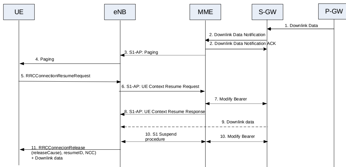
Figure 5.3.5B-1: MT-EDT procedure for User Plane CIoT EPS Optimization
