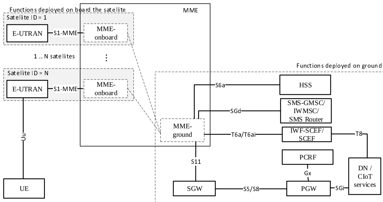
Figure O.2-1: "Split-MME" architecture for supporting Store and Forward Satellite operation for SMS and CP CIoT services
