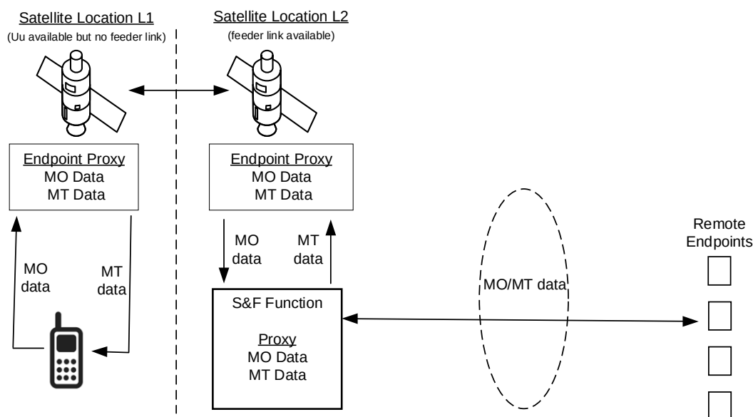
Figure O.3.2-1: Example Architecture of Model B
