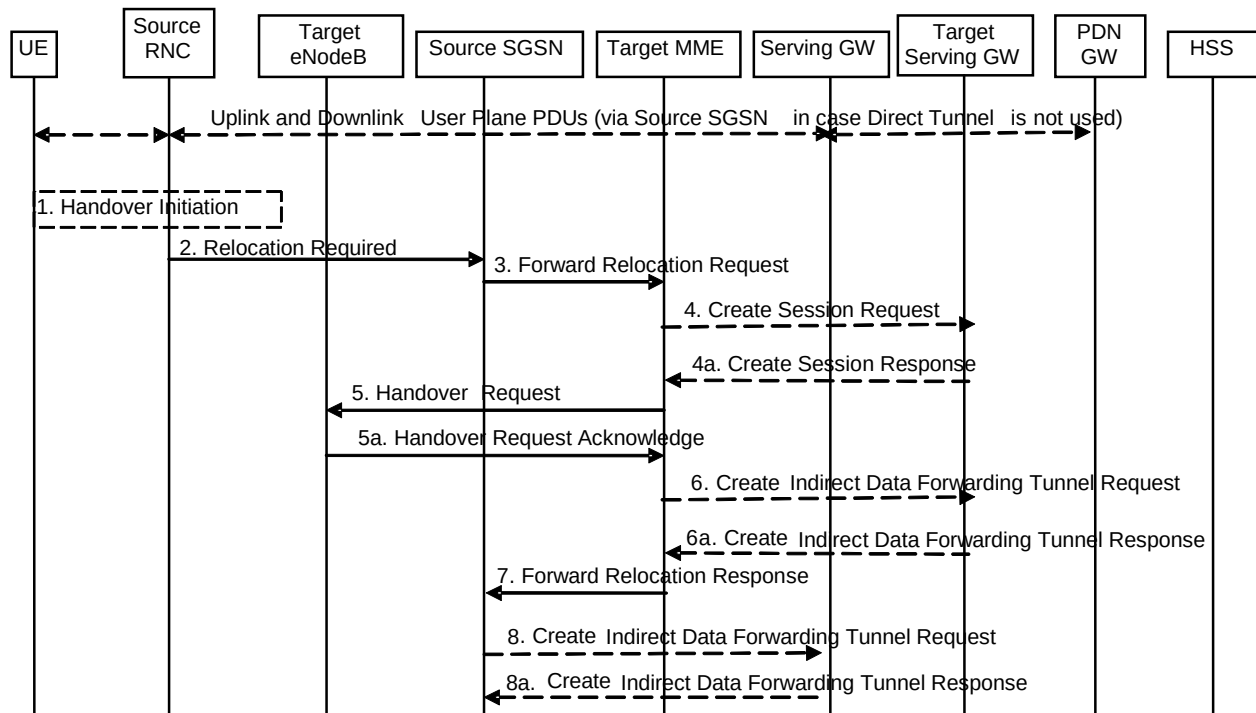
Figure 5.5.2.2-1: UTRAN Iu mode to E-UTRAN Inter RAT HO, preparation phase
