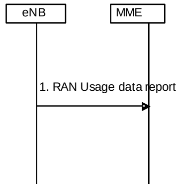
Figure 5.7A.3-1: RAN Secondary RAT usage data Reporting procedure
