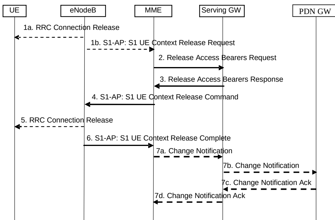
Figure 5.3.5-1: S1 Release Procedure
