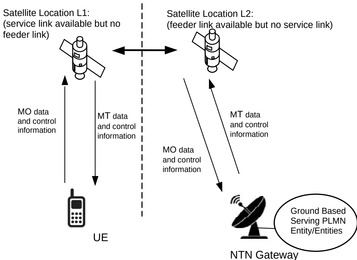
Figure 4.13.9.1-1: Store and Forward Satellite operation
