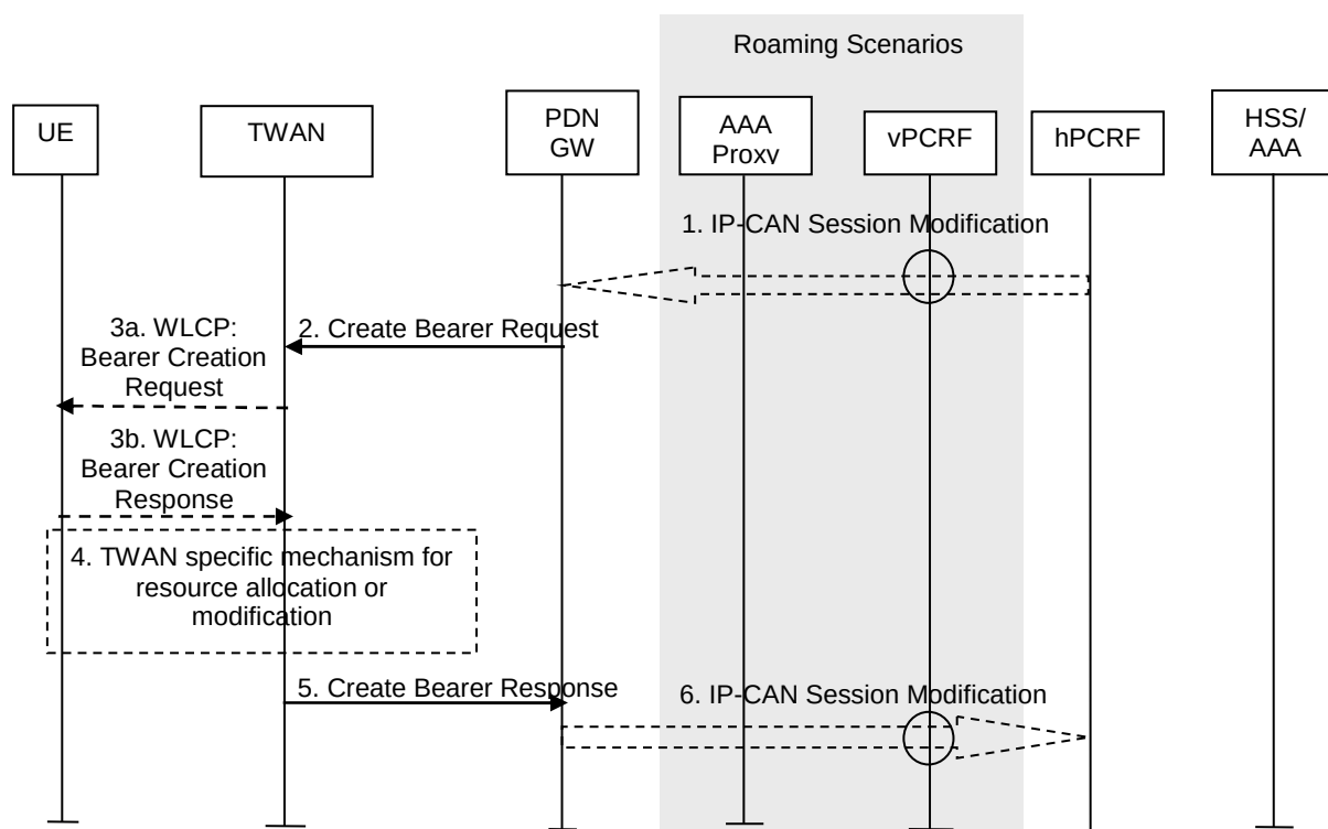
Figure 16.5-1: Dedicated S2a Bearer Activation Procedure with GTP on S2a
