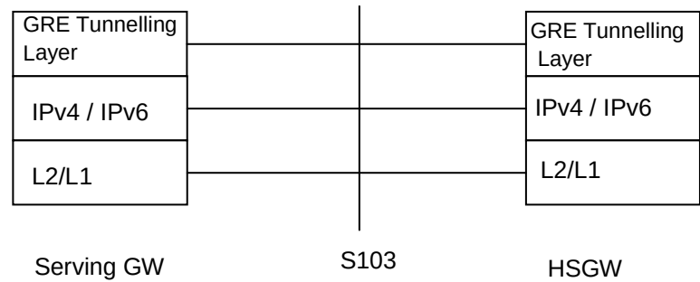
Figure 9.1.2.6-1: Protocol Stack for the S103 Reference Point
