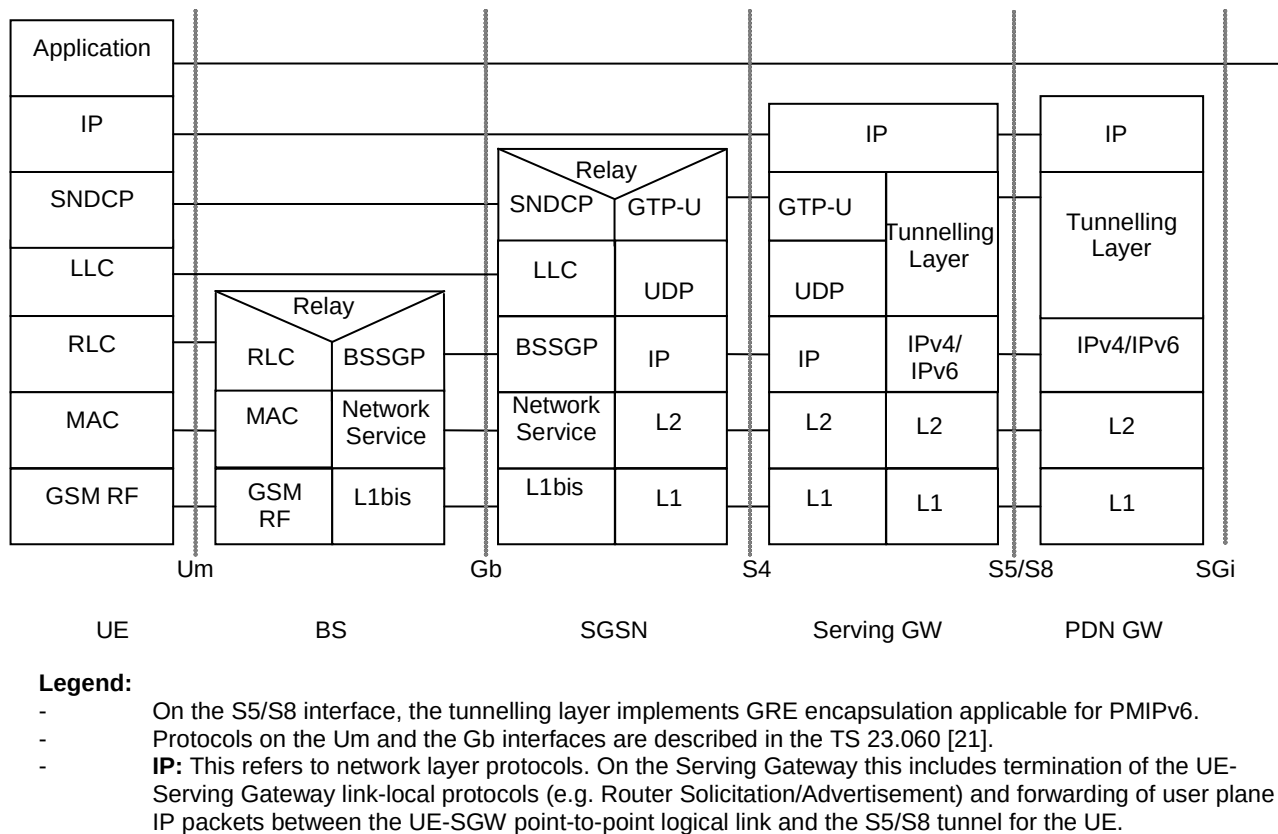
Figure 5.1.4.2-1: User Plane for A/Gb mode
