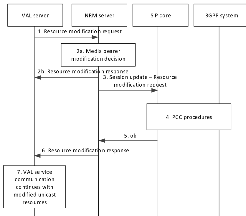
Figure 14.3.3.2.2-1: Bearer modification request
