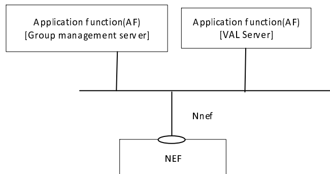
Figure 10.2.2-3: Architecture for group management utilizing the 5GS network services based on the 5GS SBA – Service based representation
