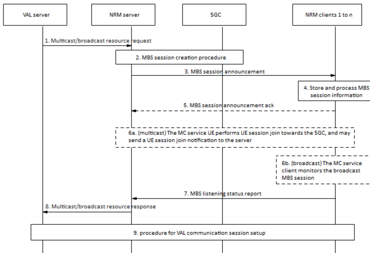
Figure 14.3.4A.1.2-1: Use of pre-created MBS session.
