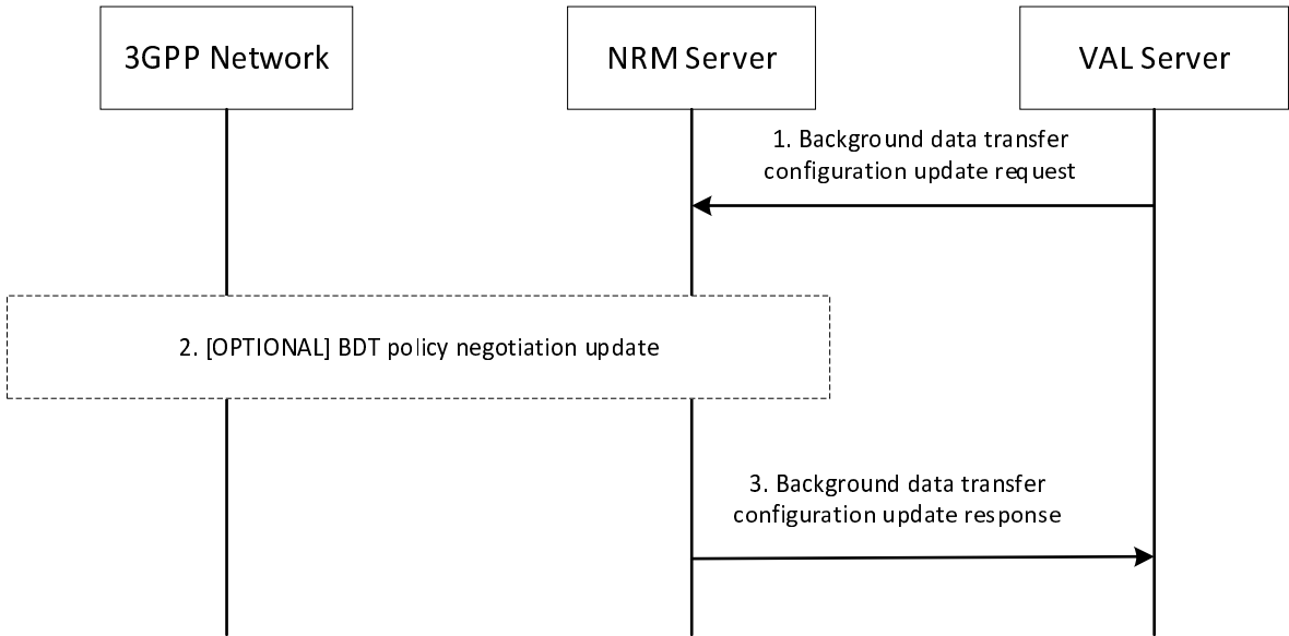
Figure 14.3.13.5-1: BDT configuration update
