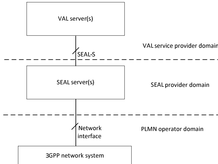
Figure 8.2.3-1: Deployment of SEAL server(s) outside of VAL service domain and PLMN operator domain
