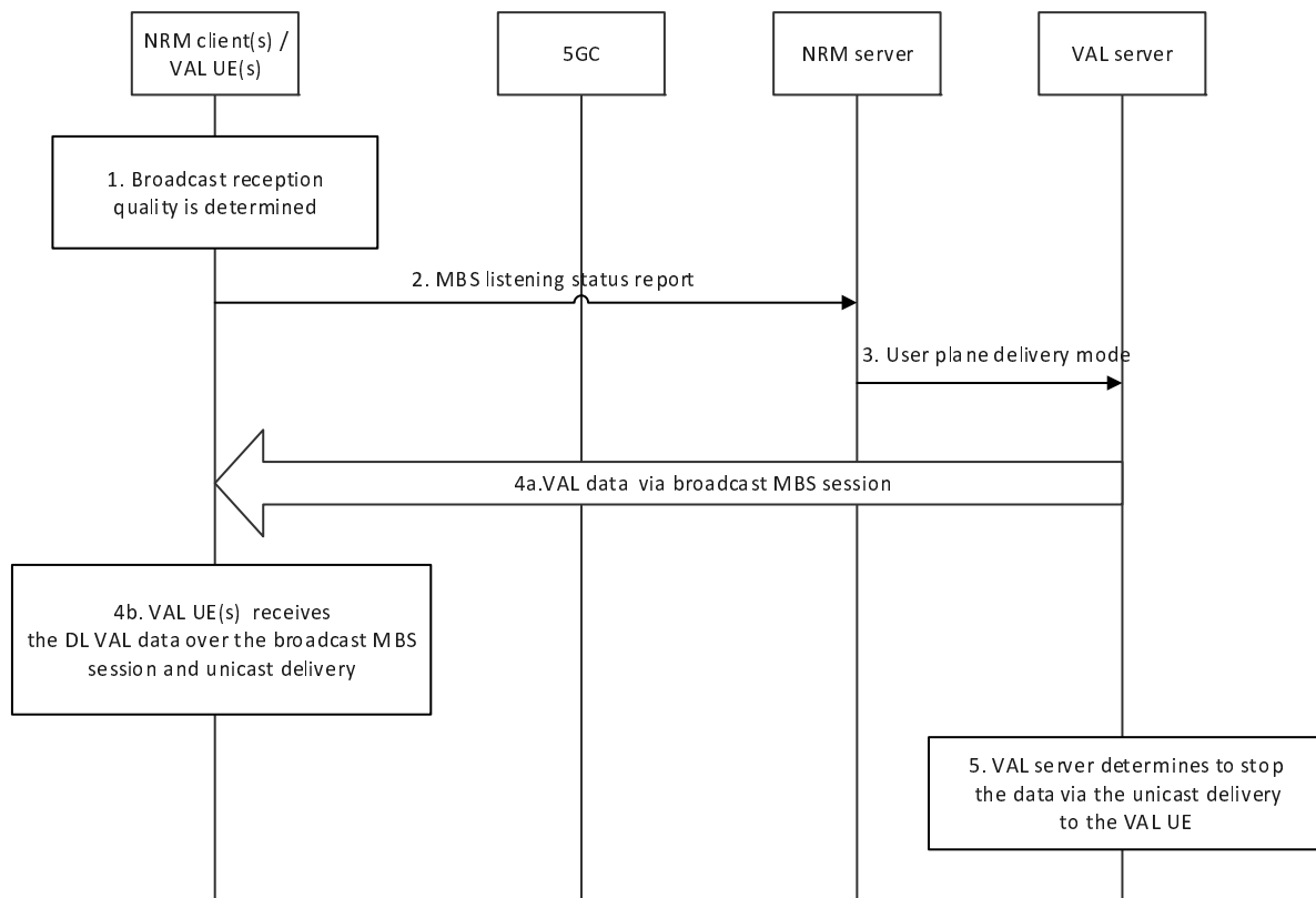
Figure 14.3.4A.8.2.2-1: Service continuity from unicast to broadcast
