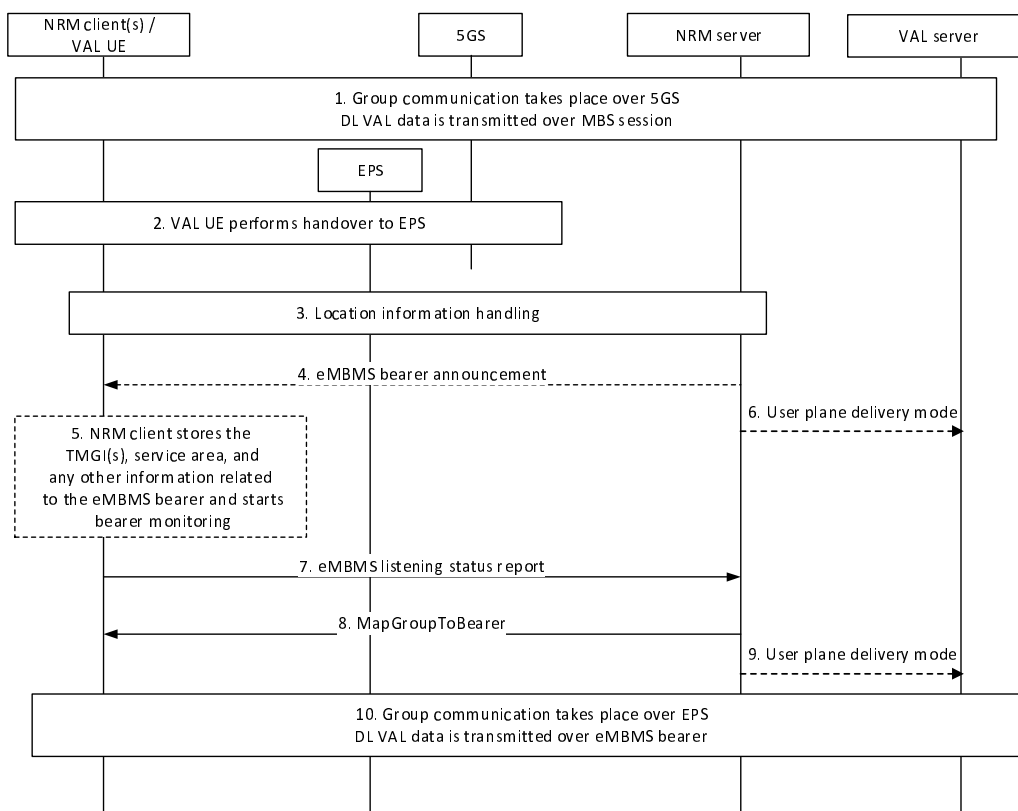
Figure 14.3.4A.10.2-1: Inter-system switching from 5G MBS session to LTE eMBMS bearer.
