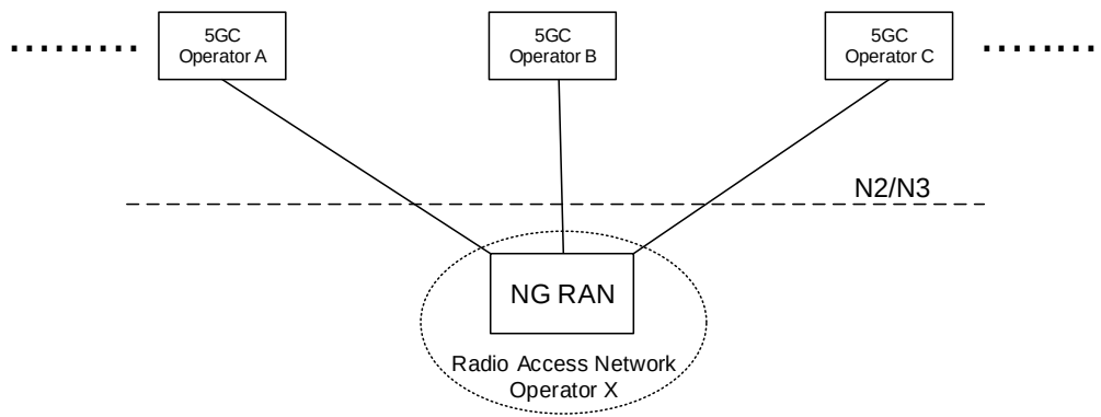
Figure 5.18.1-1: A 5G Multi-Operator Core Network (5G MOCN) in which multiple CNs are connected to the same NG-RAN
