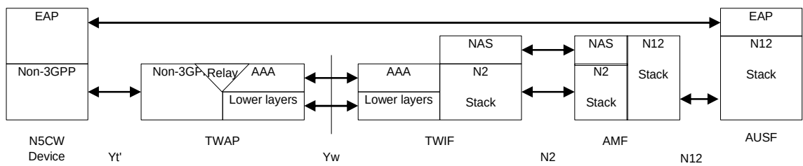
Figure 8.2.7-1: Control Plane for trusted WLAN access for N5CW device
