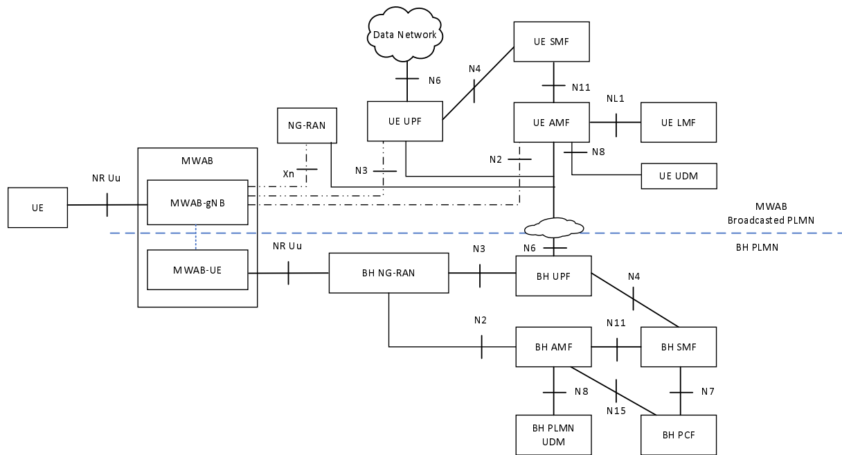
Figure S.2-2: Architecture for MWAB operation support - non-roaming with two PLMNs
