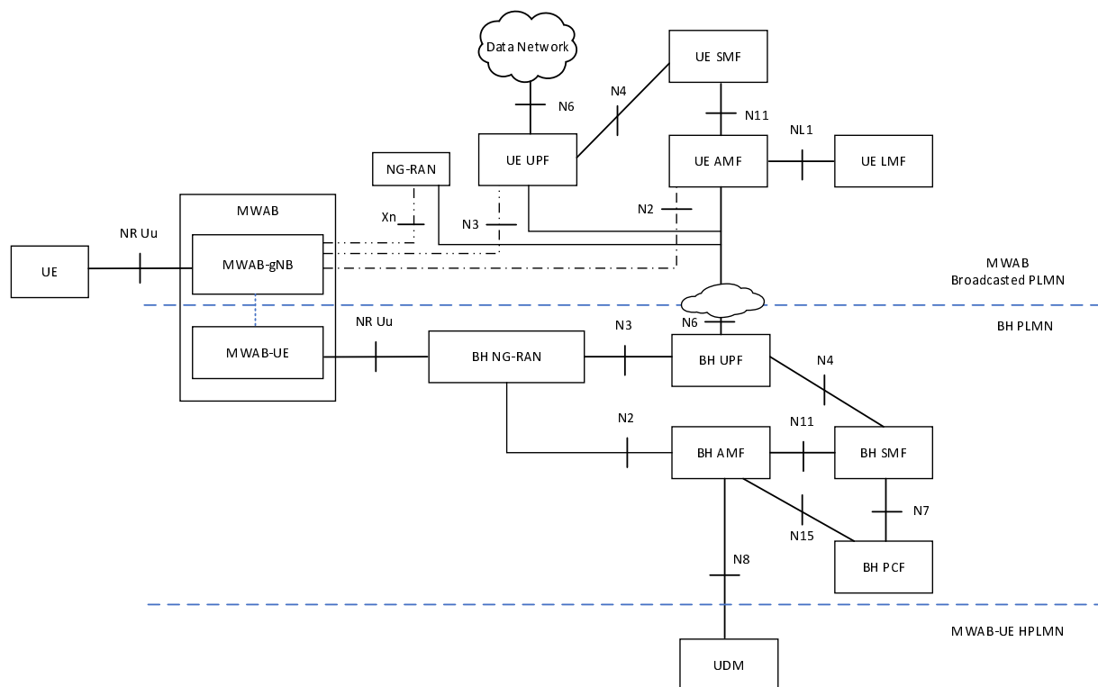
Figure S.2-3: Architecture for MWAB operation support - MWAB-UE roaming with Local Breakout
