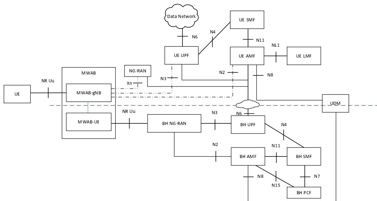
Figure S.2-1: Architecture for MWAB operation support - non-roaming with one PLMN
