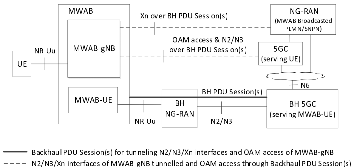
Figure 5.49.1.1-1: MWAB architecture for 5GS
