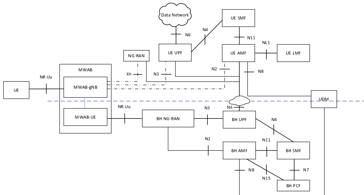
Figure S.3-1: Architecture for MWAB operation support for SNPN - with MWAB-UE served by the subscribed SNPN (BH SNPN) and MWAB-gNB in the same SNPN
