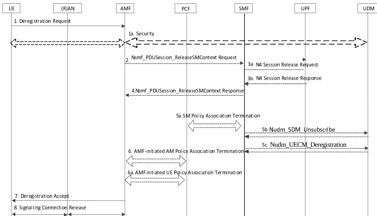
Figure 4.2.2.3.2-1: UE-initiated Deregistration
