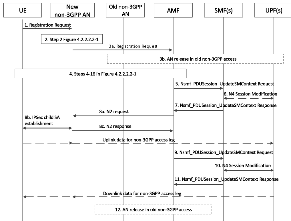
Figure 4.22.9.5-1: Mobility Registration procedure for non-3GPP access path switching
