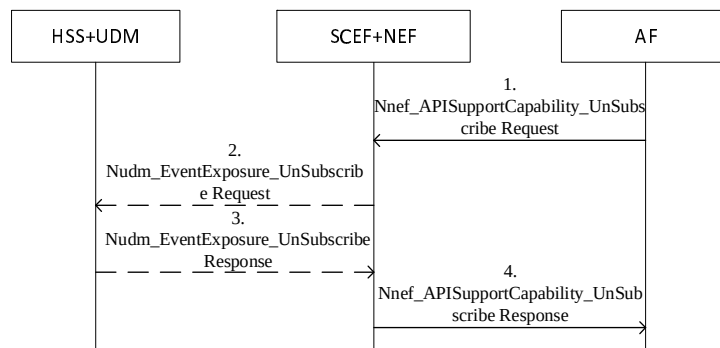
Figure 4.11.6.2 1: Unsubscribing to notification of the availability or expected level of support of a service API
