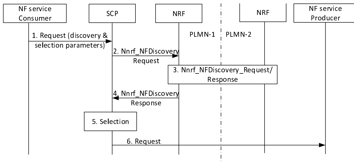
Figure 4.17.10-1: Delegated NF service discovery when NF service consumer and NF service producer are in different PLMNs
