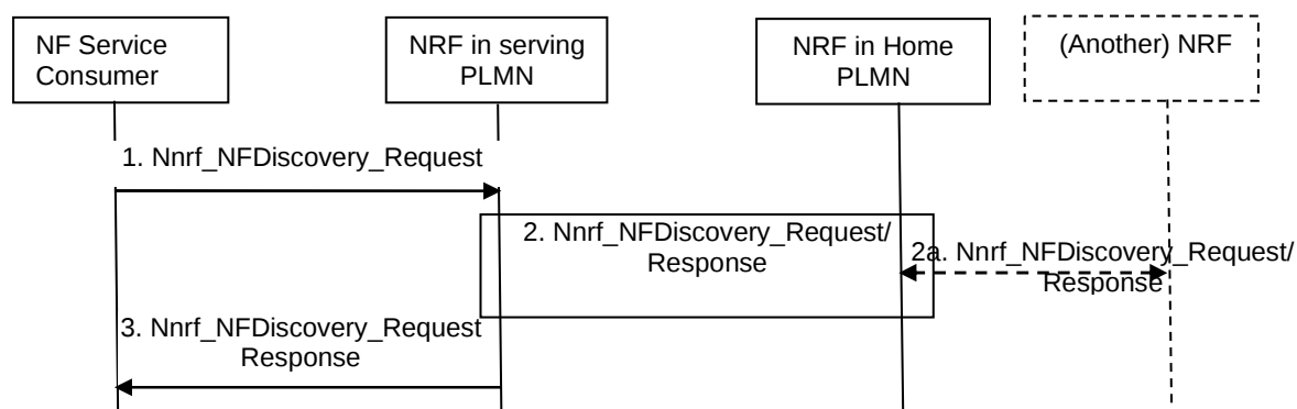
Figure 4.17.5-1: NF/NF service discovery across PLMNs
