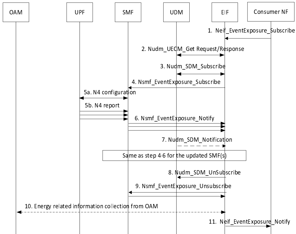
Figure 4.29.2-1: Energy Consumption information collection
