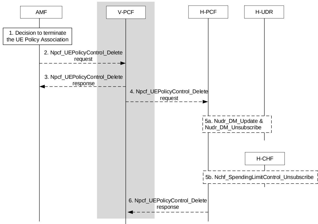
Figure 4.16.13.1-1: AMF-initiated UE Policy Association Termination
