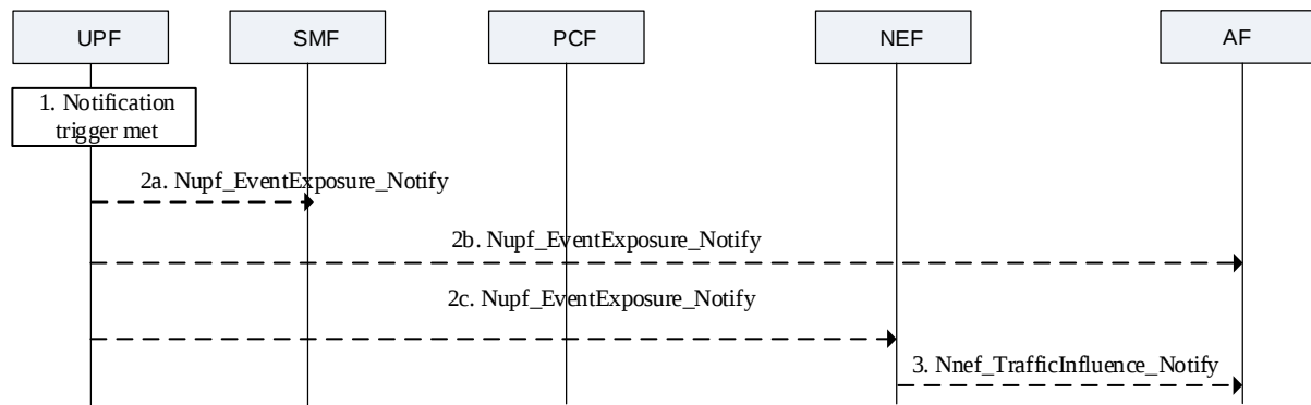
Figure 4.15.12.3-1: Notification of Handling of Payload Header Event
