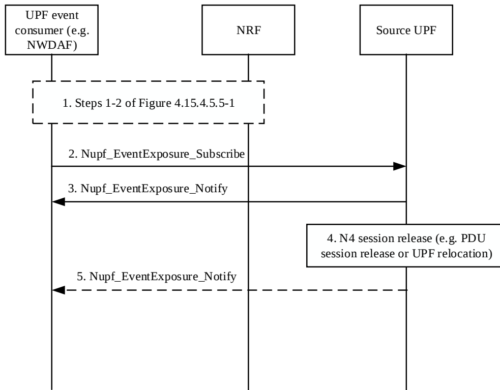
Figure 4.15.4.5.7-1: Subscription directly to UPF event exposure service during N4 session release
