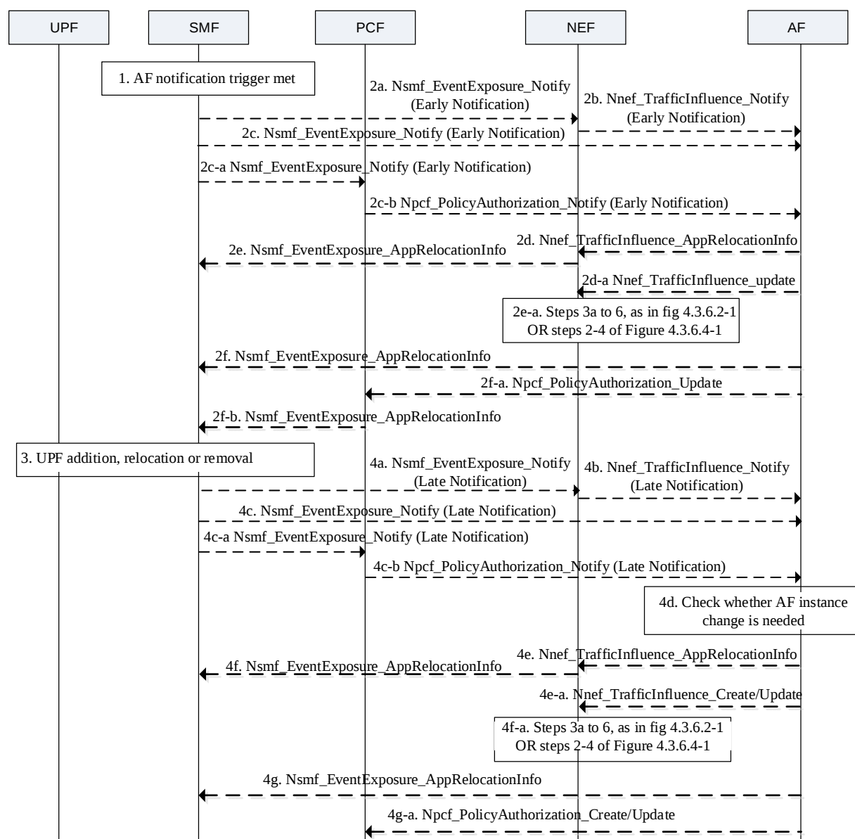
Figure 4.3.6.3-1: Notification of user plane management event
