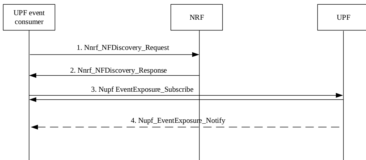
Figure 4.15.4.5.5-1: Subscription to UPF event exposure service for certain UE(s) directly using UE's IP address
