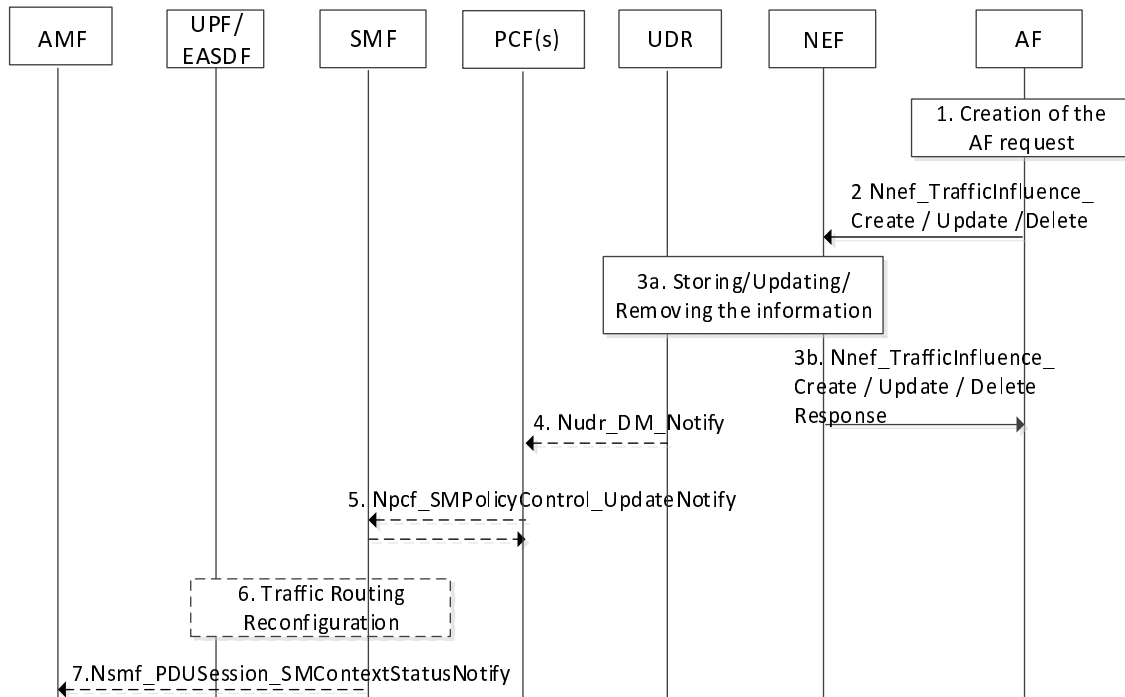
Figure 4.3.6.2-1: Processing AF requests to influence traffic routing and/or Service Function Chaining for Sessions not identified by an UE address
