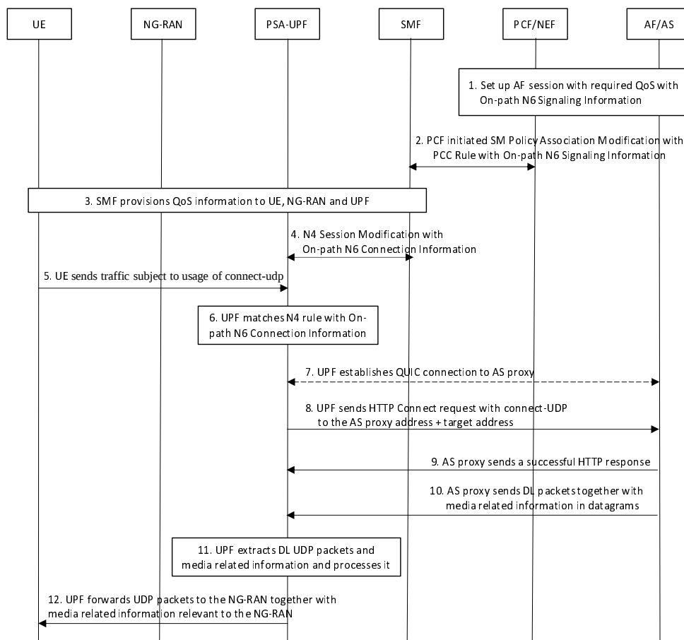
Figure K.1.1-1: Use of connect-udp for transmission of media related information
