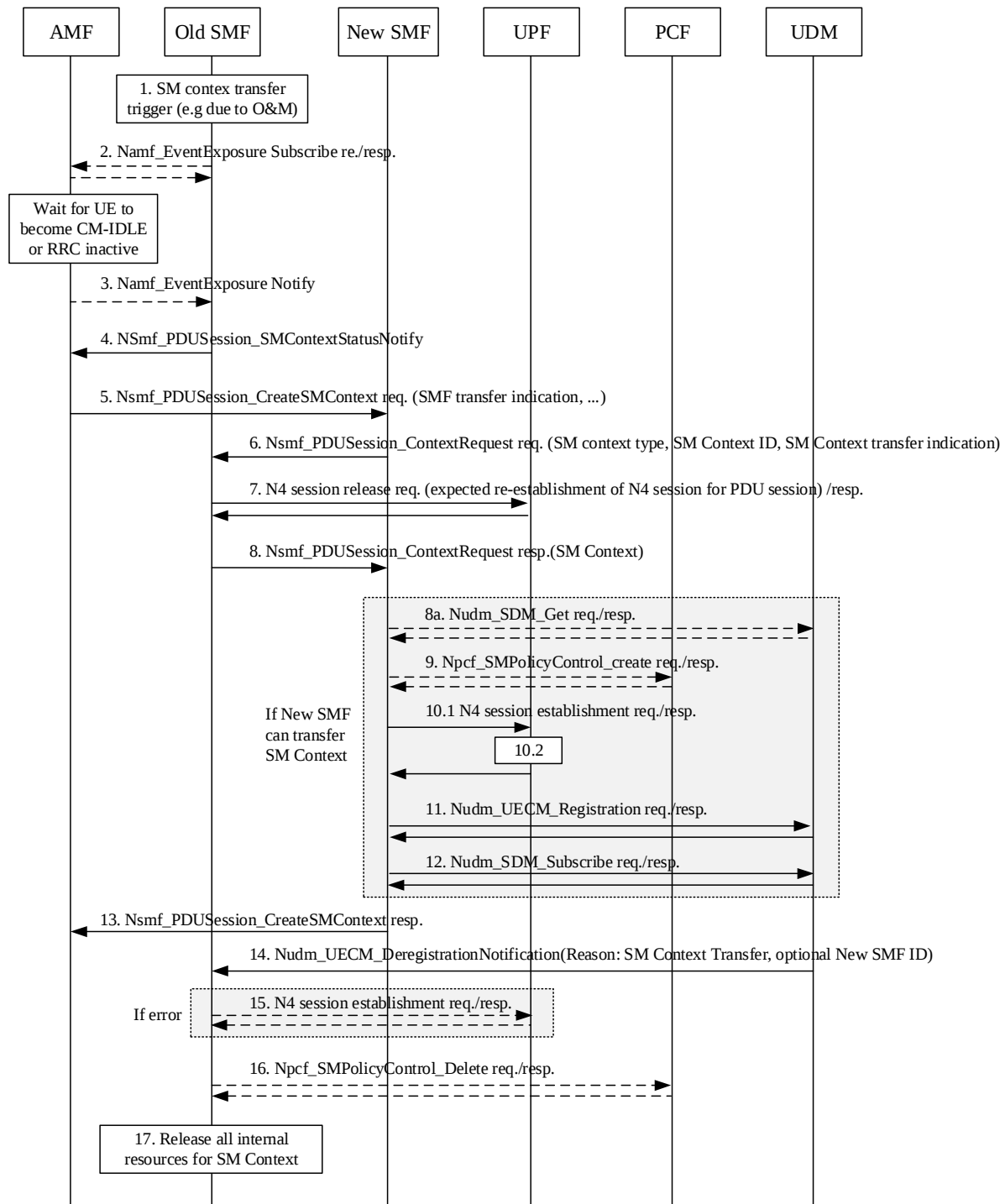
Figure 4.26.4.1.1-1: Context transfer of a PDU session
