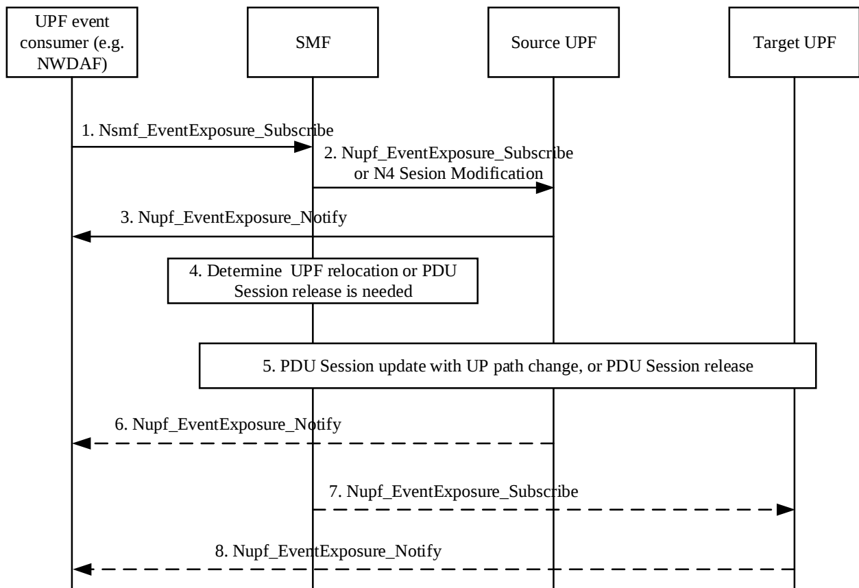
Figure 4.15.4.5.6-1: Subscription to UPF event exposure service via SMF during UPF relocation and PDU Session release
