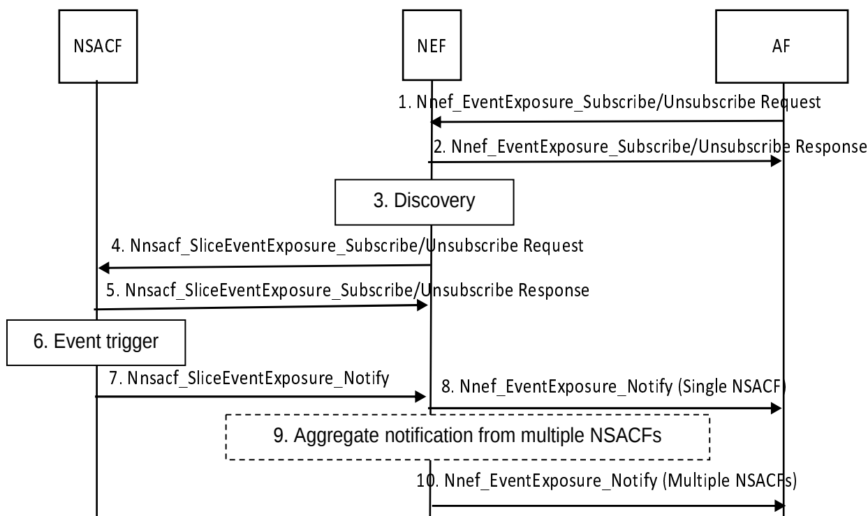
Figure 4.15.3.2.10.1-1: Reported value(s) aggregated at NEF per network slice notification procedure
