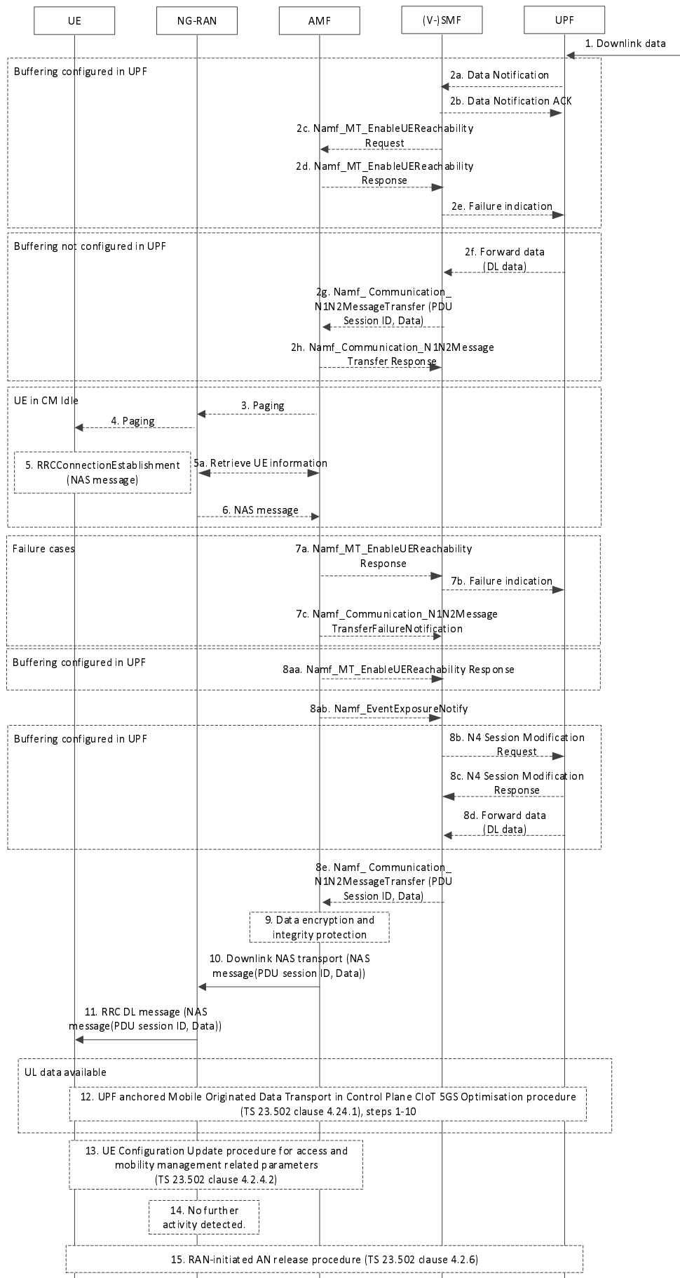
Figure 4.24.2-1: Mobile Terminated Data Transport in Control Plane CIoT 5GS Optimisation
