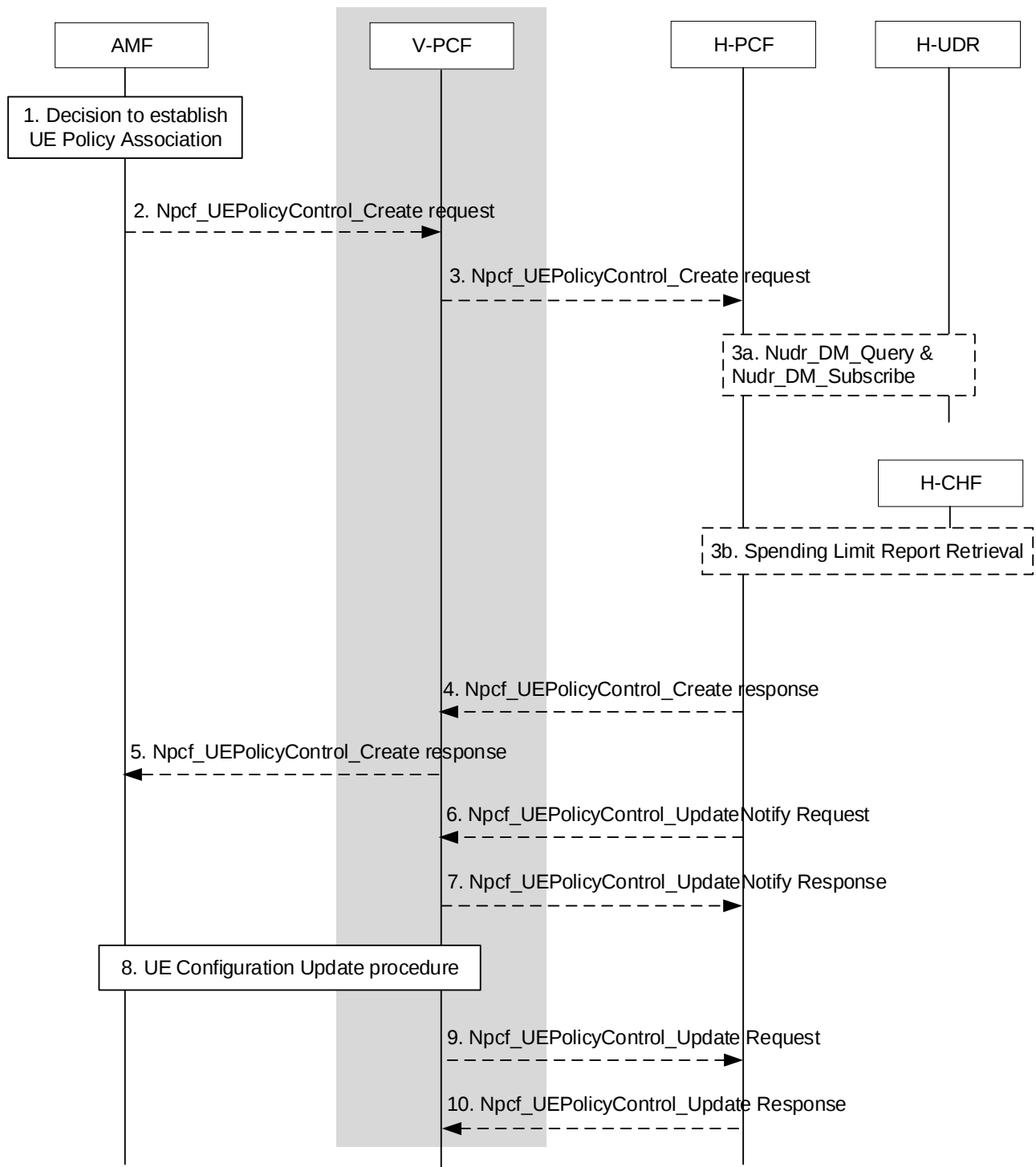
Figure 4.16.11-1: UE Policy Association Establishment
