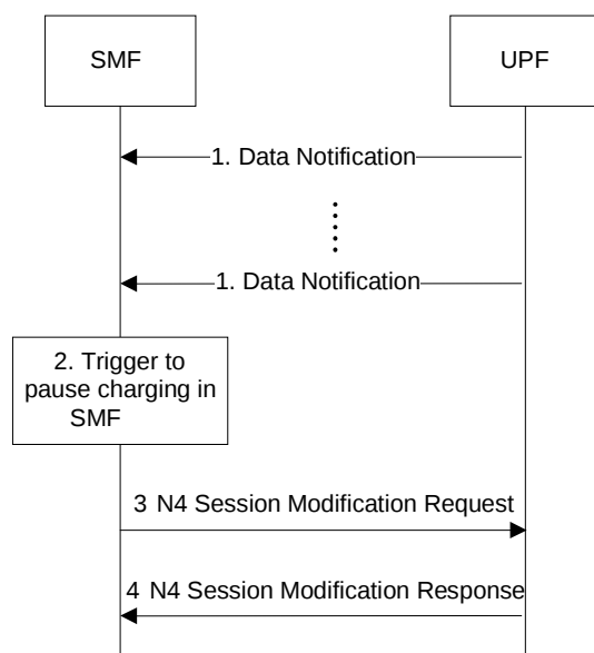
Figure 4.4.4-1: SMF Pause of charging procedure
