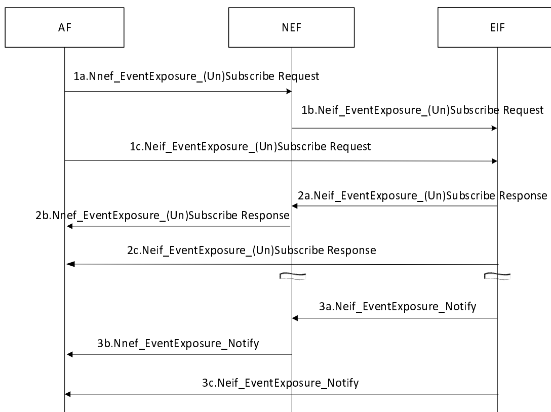
Figure 4.29.1-1: Energy consumption information exposure
