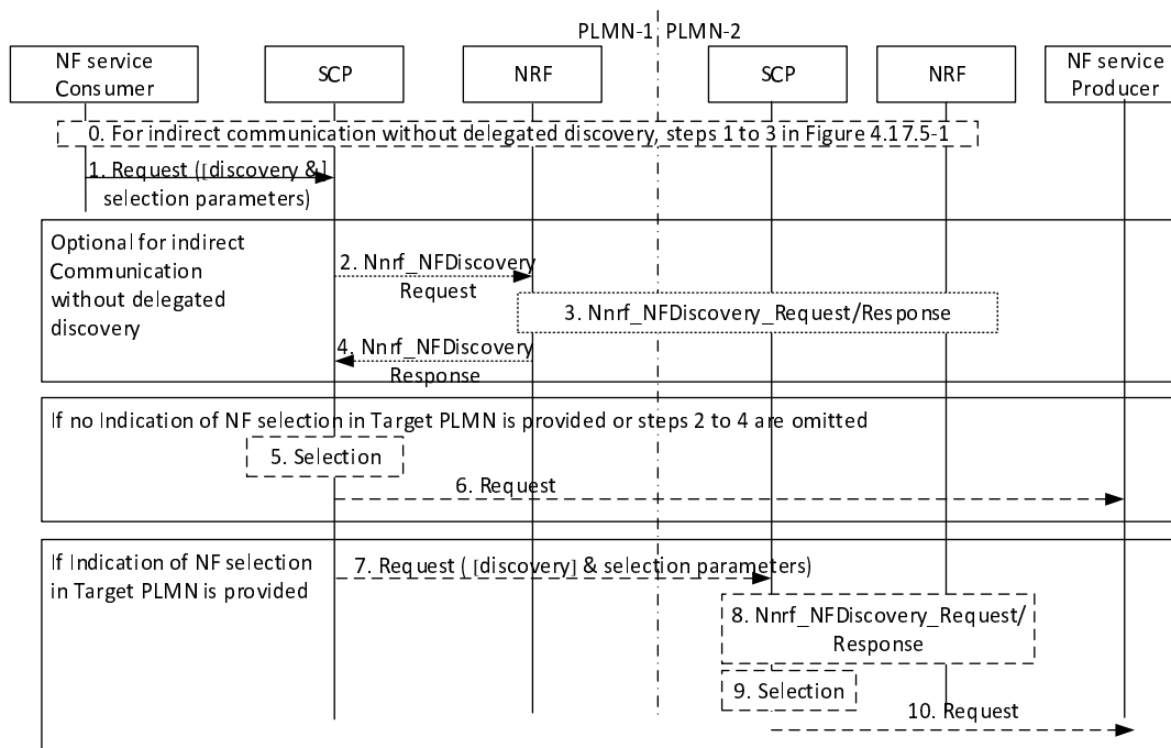
Figure 4.17.10a-1: Delegated NF service discovery when NF service consumer and NF service producer are in different PLMNs with possible NF selection at target PLMN
