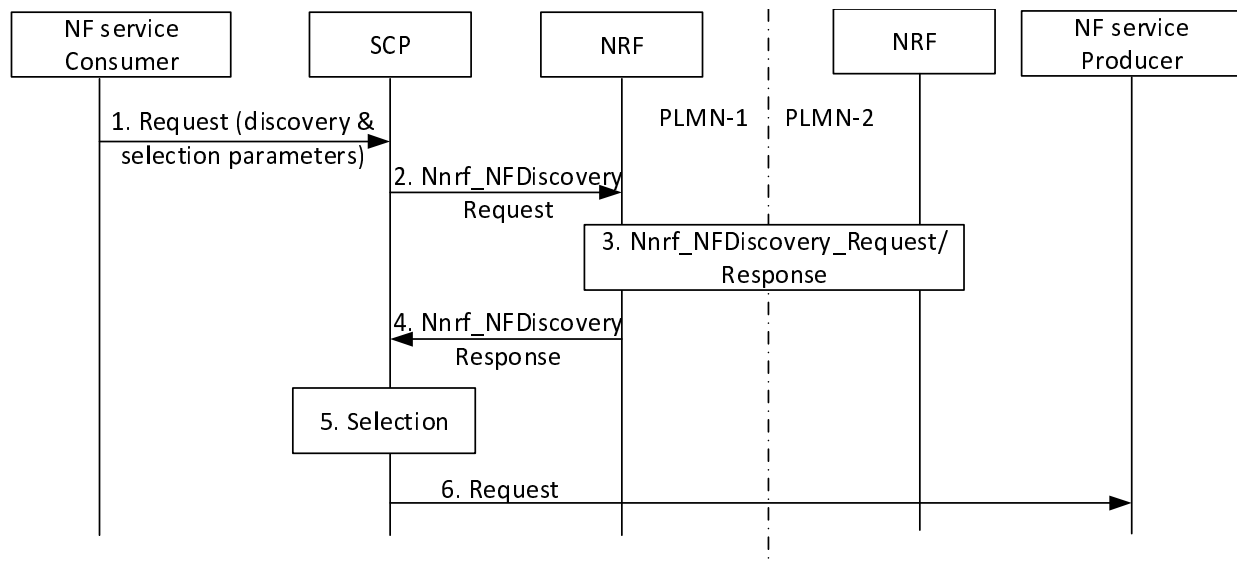
Figure 4.17.10-1: Delegated NF service discovery when NF service consumer and NF service producer are in different PLMNs without NF selection at target PLMN
