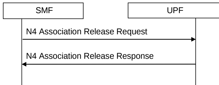
Figure 4.4.3.3-1: SMF initiated N4 association release procedure
