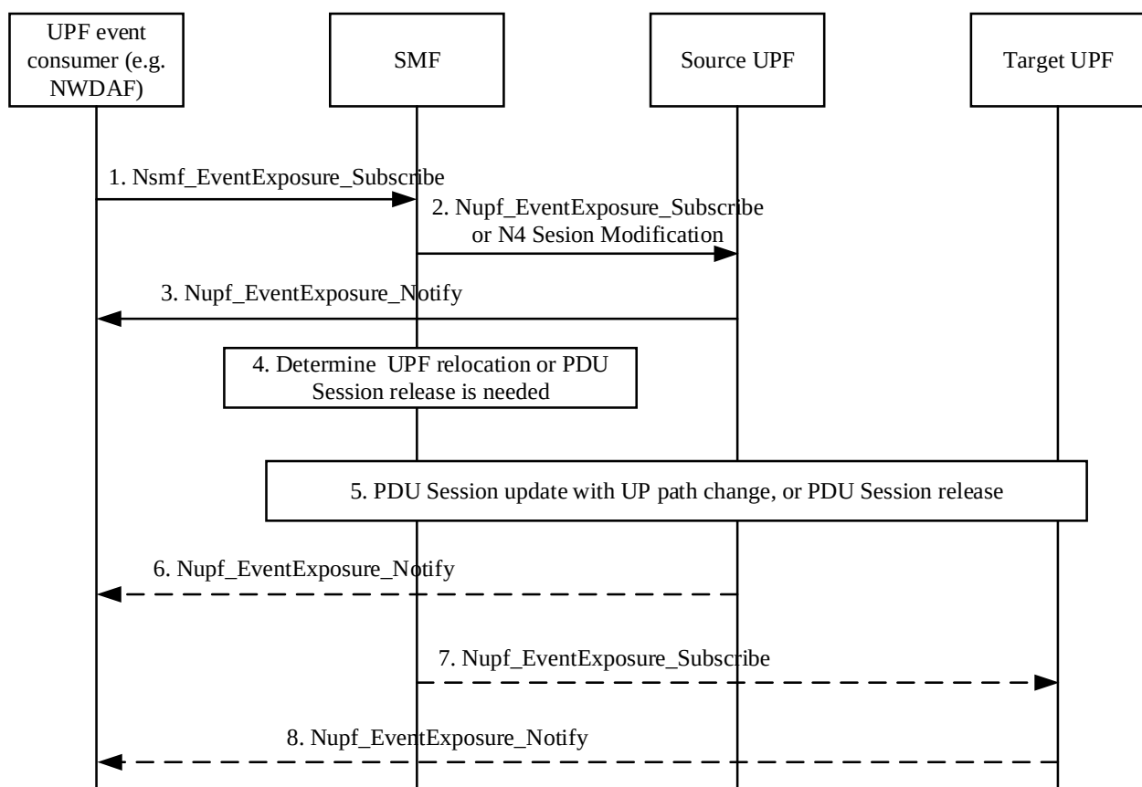
Figure 4.15.4.5.6-1: Subscription to UPF event exposure service via SMF during UPF relocation and PDU Session release
