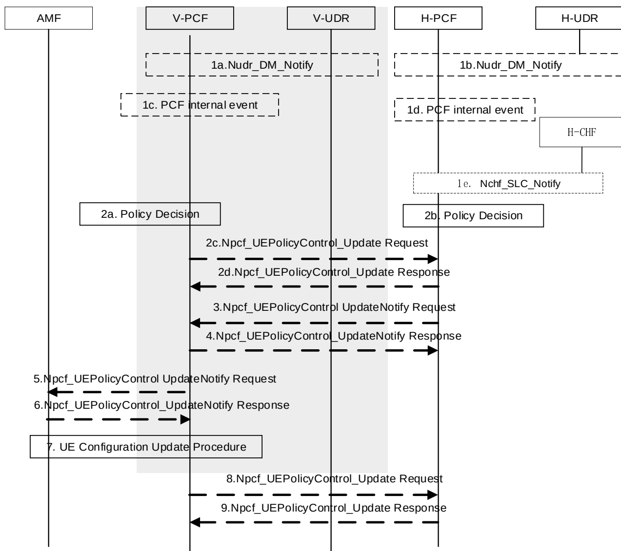
Figure 4.16.12.2-1: UE Policy Association Modification initiated by the PCF
