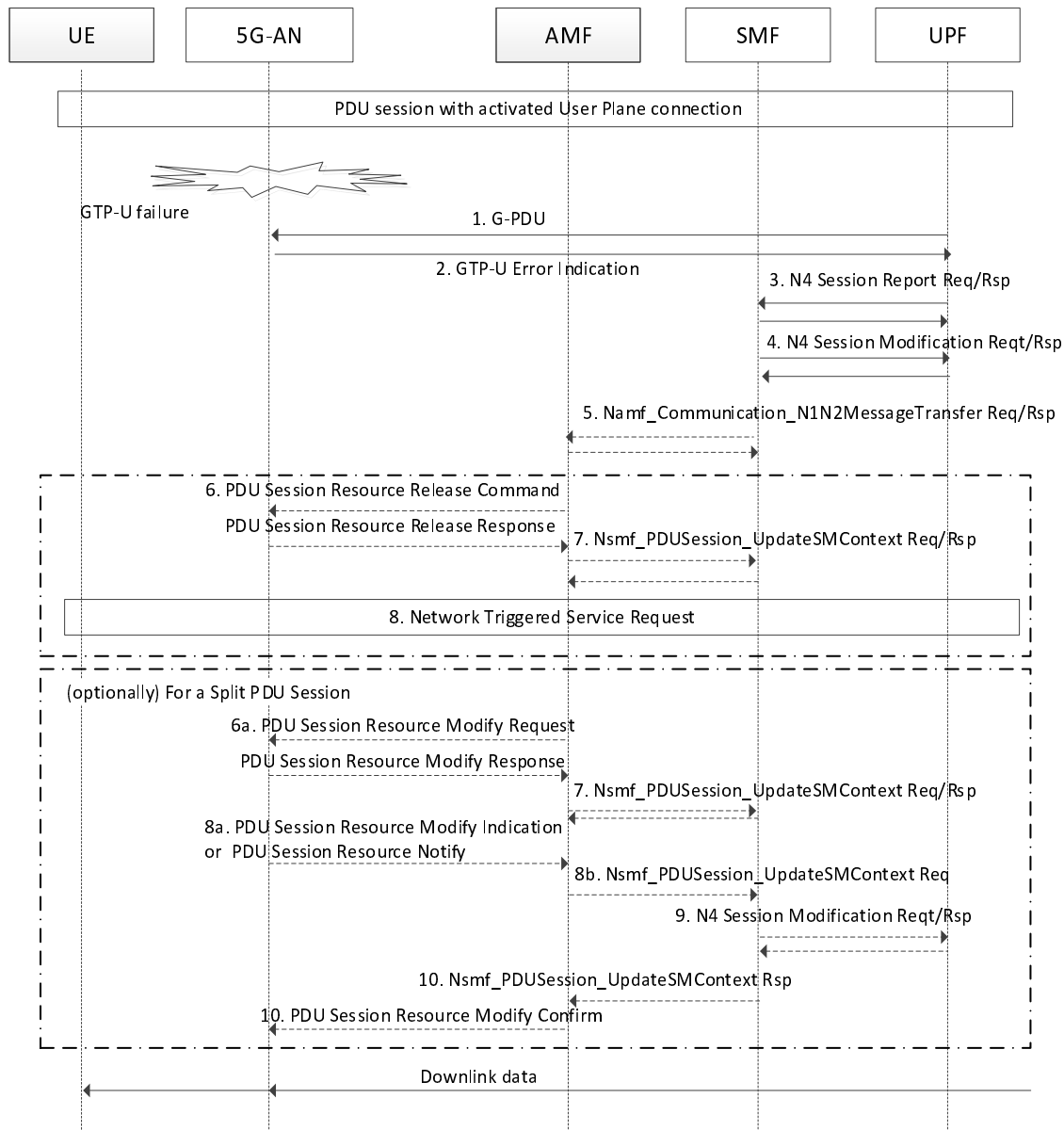
Figure 5.3.2.1-1: GTP-U Error Indication from 5G-AN
