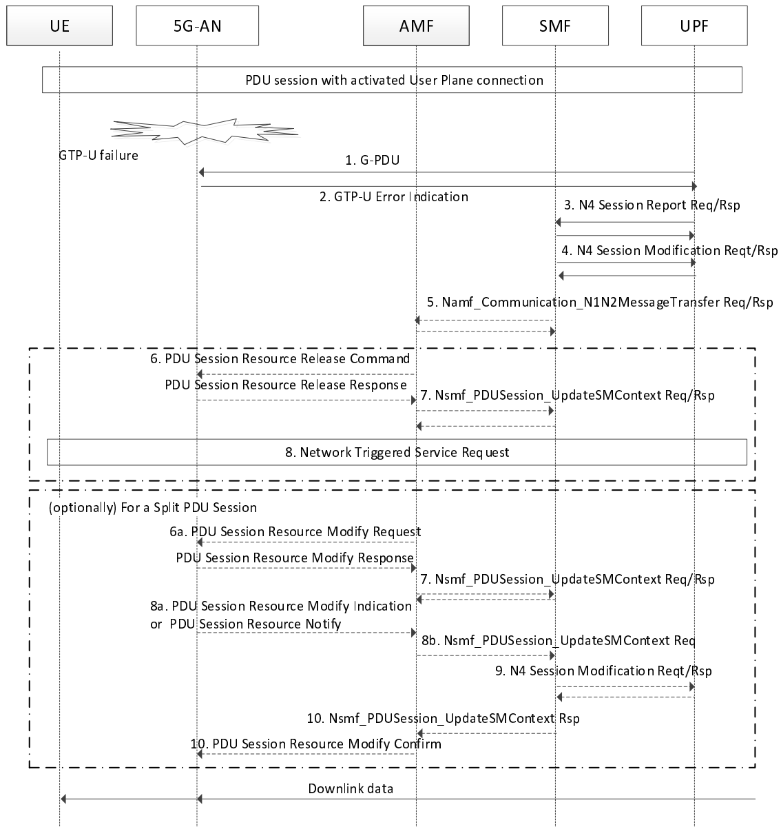
Figure 5.3.2.1-1: GTP-U Error Indication from 5G-AN
