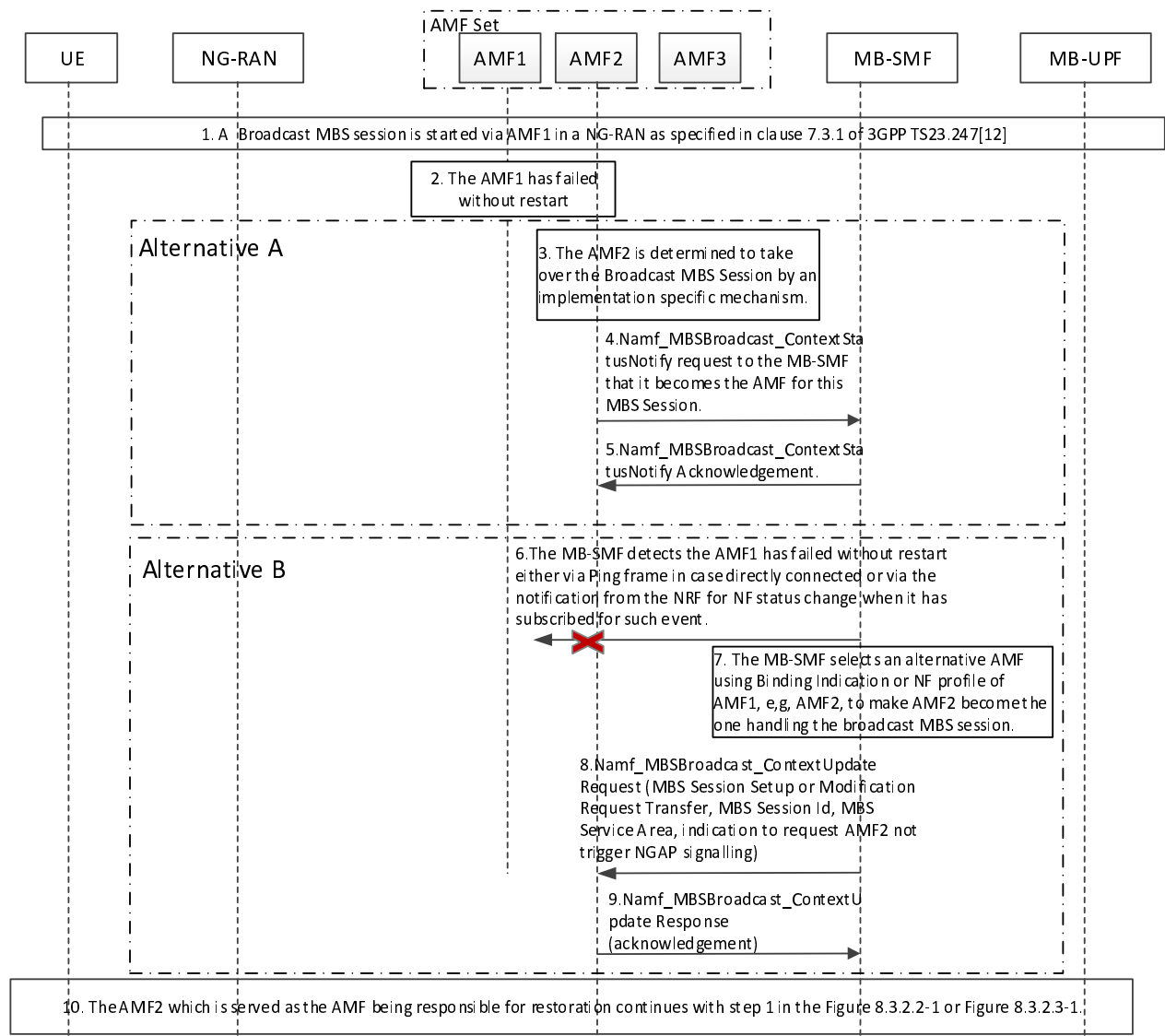
Figure 8.3.2.4-1 Selecting an alternative AMF at AMF failure.
