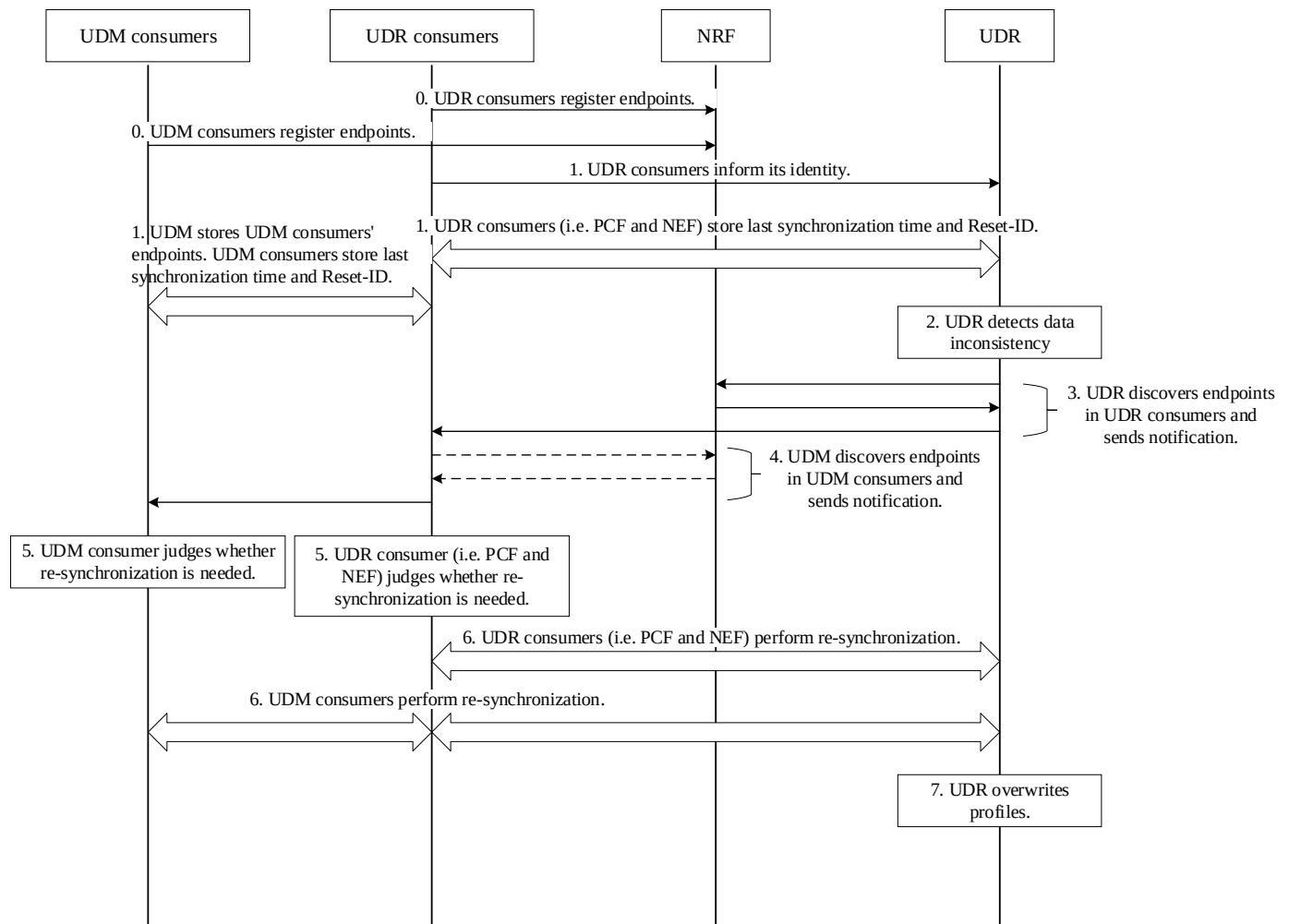
Figure 6.7.2-1: Restoration of Profiles related to UDR
