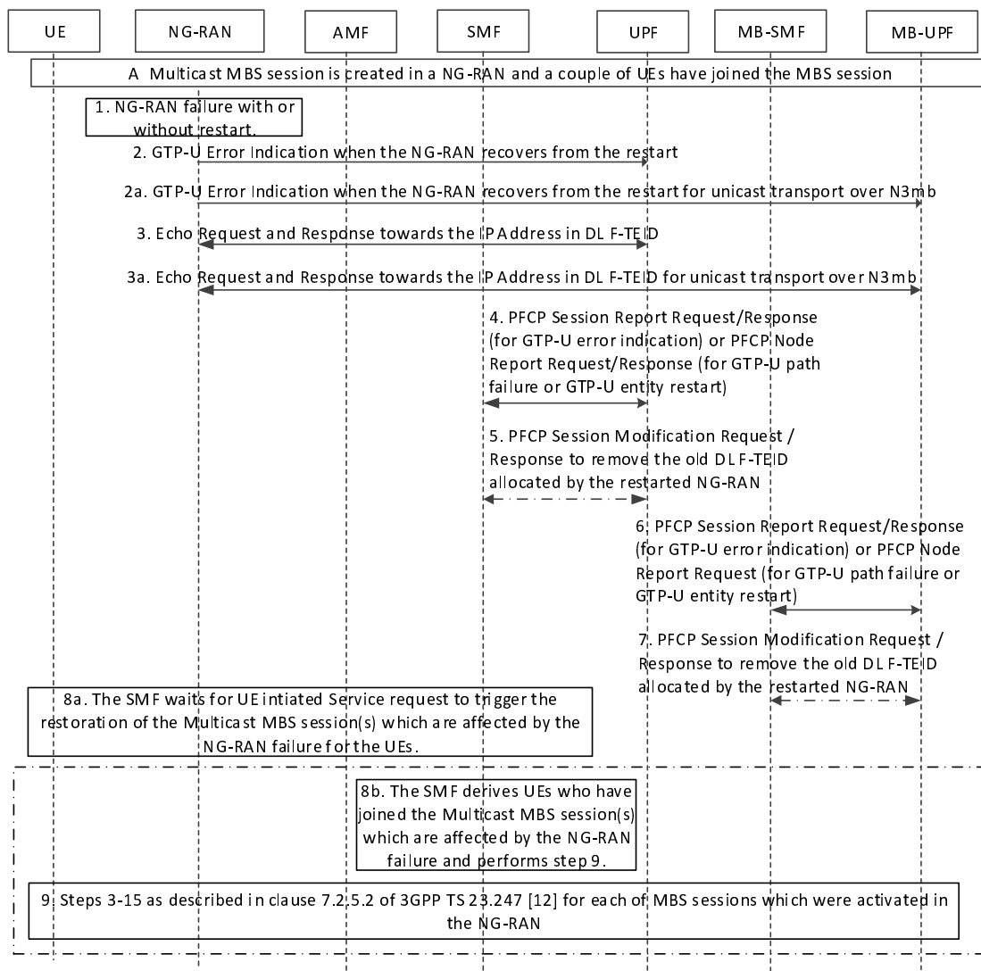
Figure 8.3.4-1: Multicast MBS session restoration upon NG-RAN failure with or without restart
