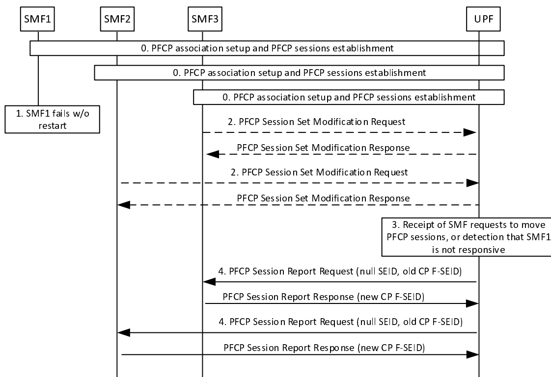
Figure 4.4.3.2-1: Failure (without restart) of an SMF in an SMF set using the MPAS or SSET feature
