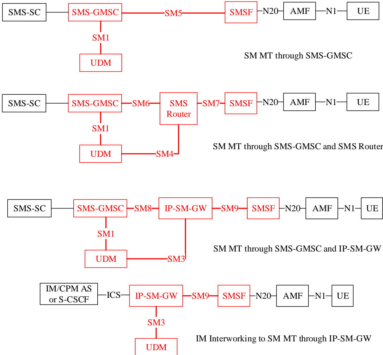
Figure 4.1-2a: Non-roaming System Architecture for SBI-based MT SMS in reference point representation
