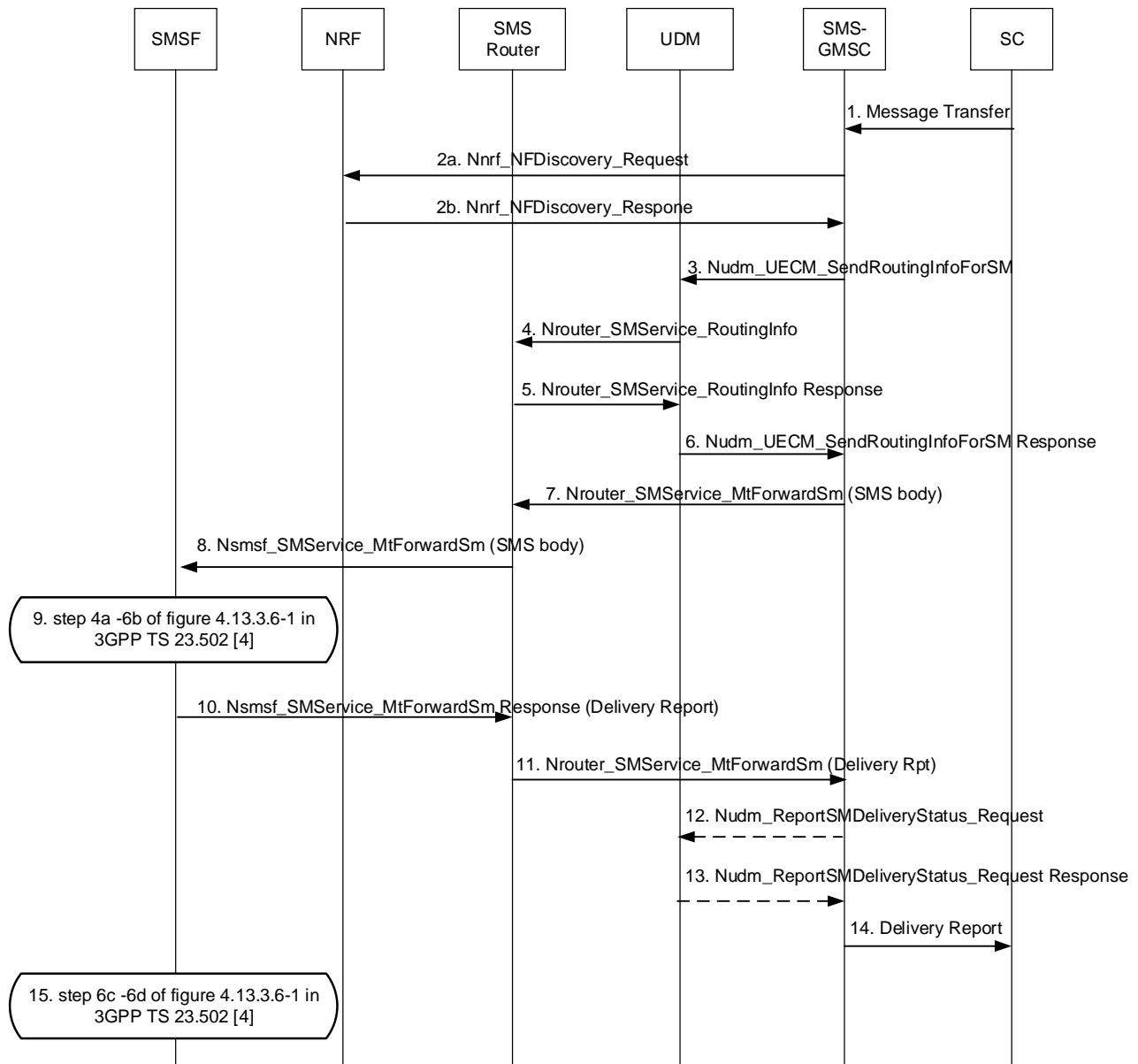
Figure 5.1.3-1: MT SMS over NAS via SMS Router
