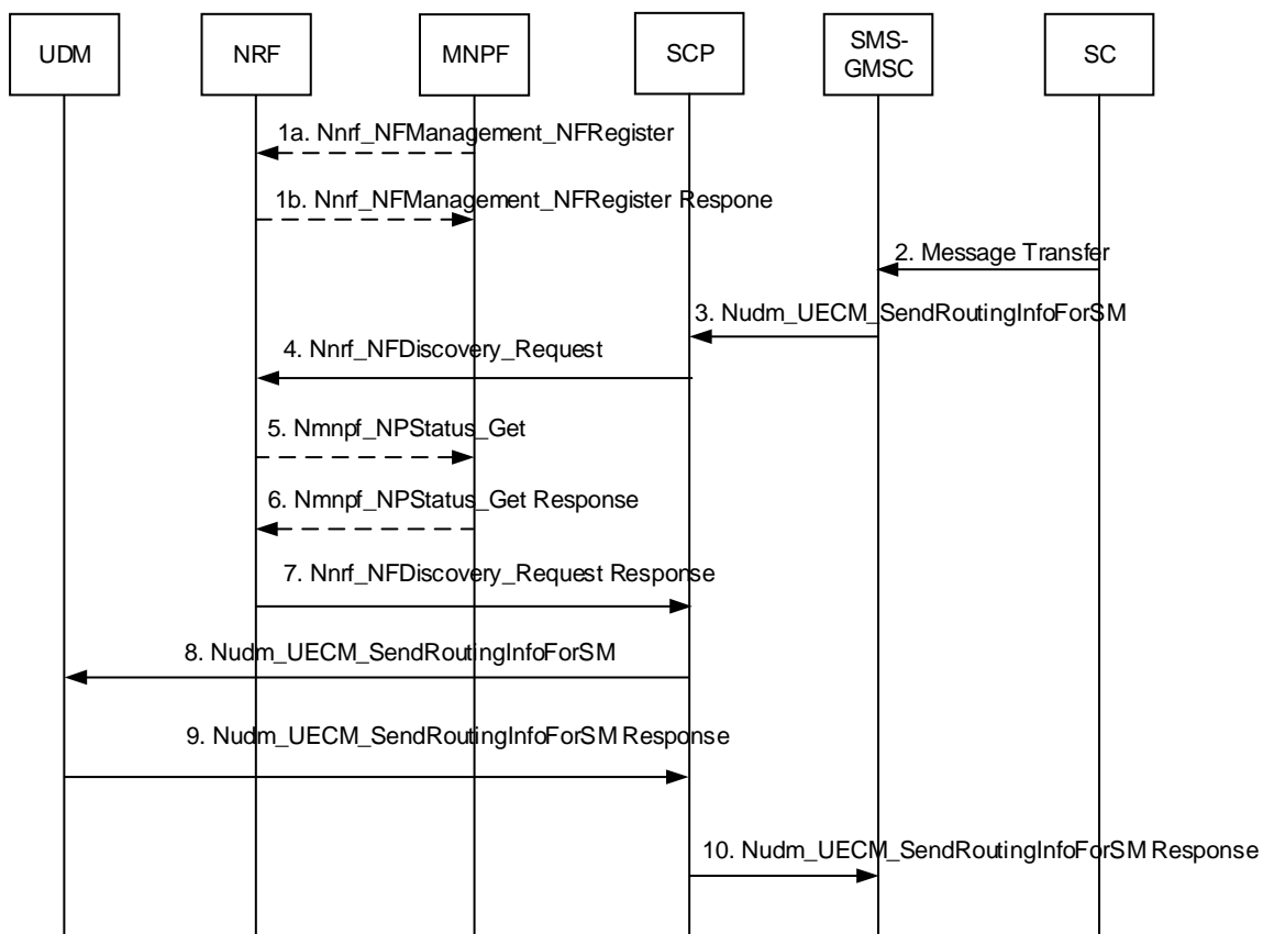
Figure 5.1.7.3.3-1: SCP supports GPSI-to-Subscription-Network resolution with NRF
