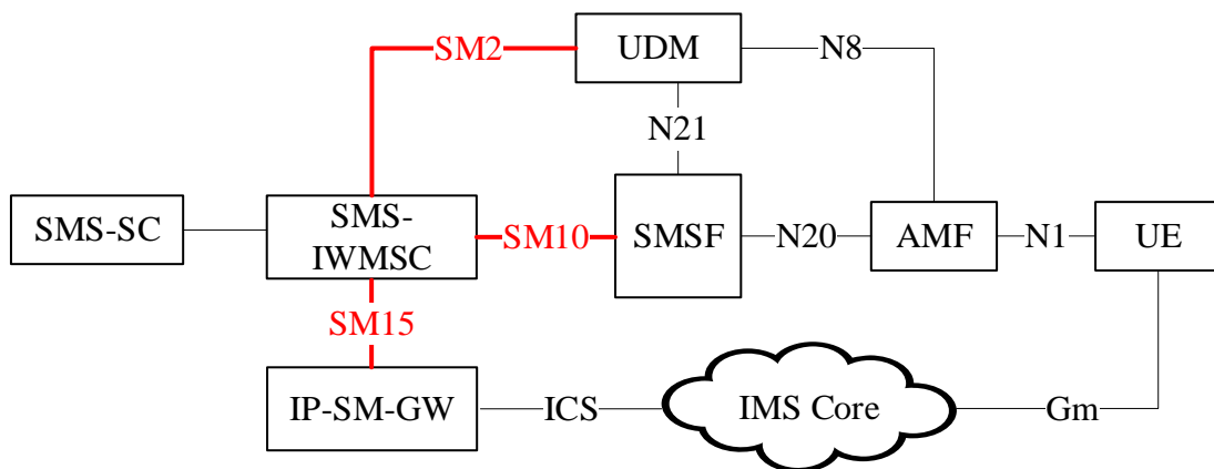
Figure 4.1-2b: Non-roaming System Architecture for SBI-based MO SMS in reference point representation
