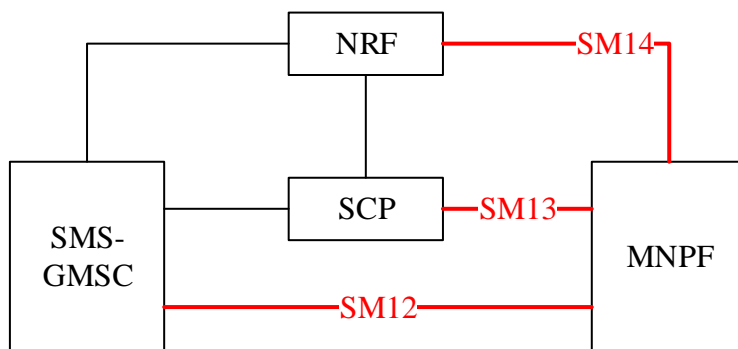
Figure 4.1-2d: Architecture for NP status Retrieval from MNPF in reference point representation
