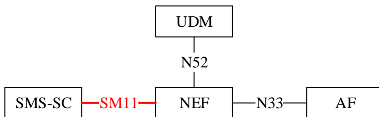
Figure 4.1-2c: Architecture for SBI-based MSISDN-less MO SMS and device triggering in reference point representation
