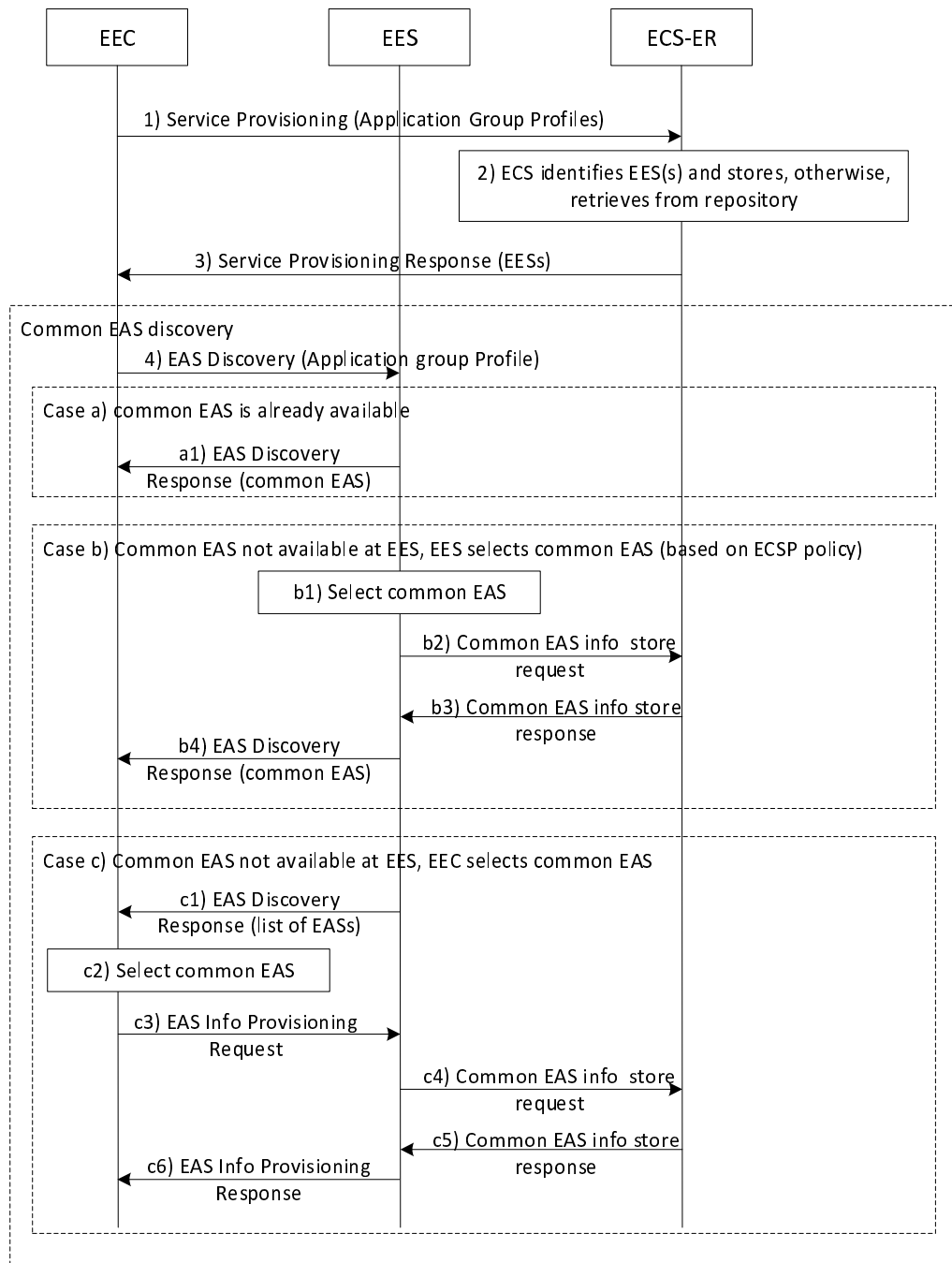
Figure E.2.3-1: Common EAS discovery and announcement (with repository)
