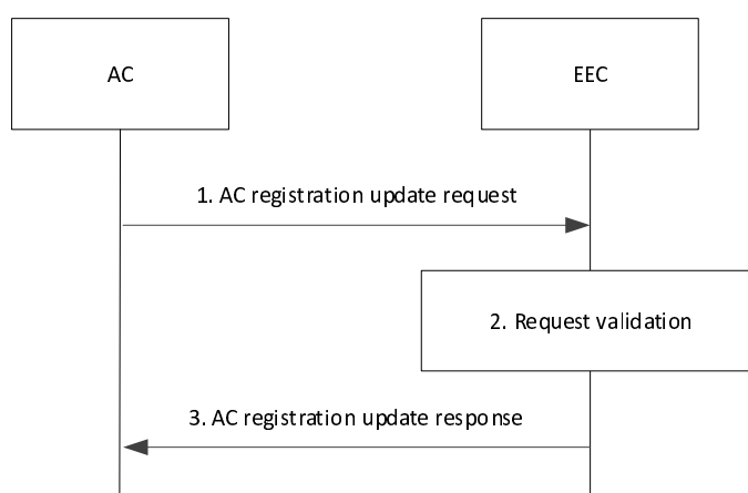
Figure 8.14.2.2.3-1: AC registration update procedure
