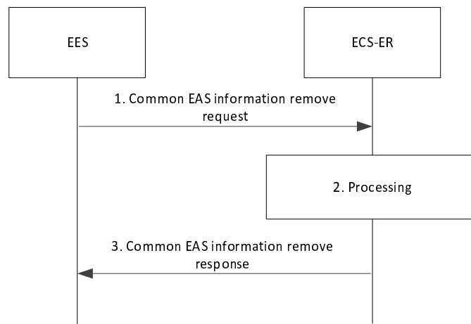
Figure 8.20.2.4-1: Common EAS information removal
