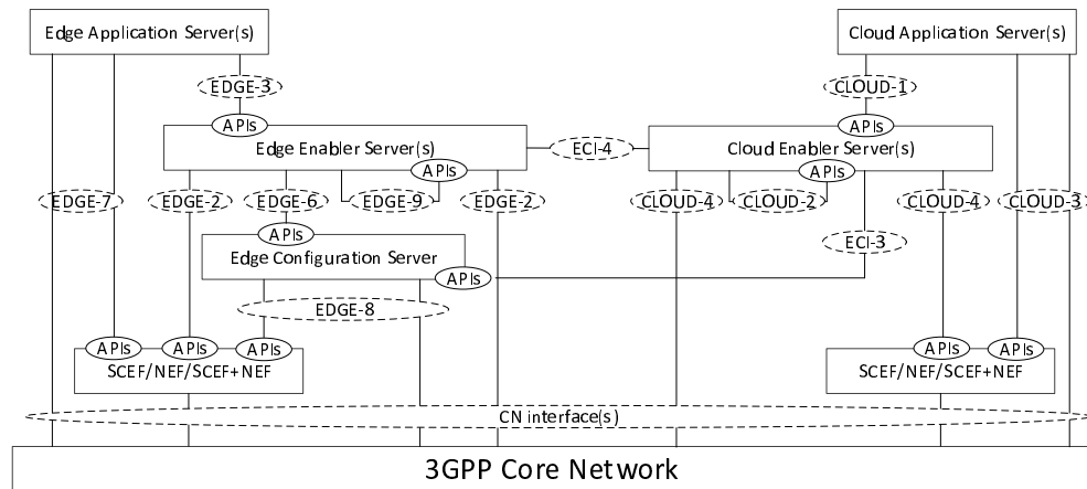
Figure 6.8.1-1: Capability exposure for enabling cloud applications with edge applications with CES
