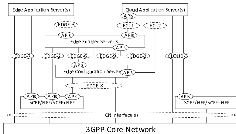
Figure 6.9.1-1: Capability exposure for enabling cloud applications with edge applications
