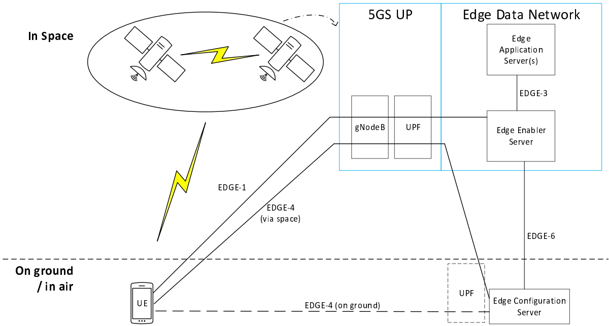
Figure A.2.5-1: EDN deployment with gNB on satellite
