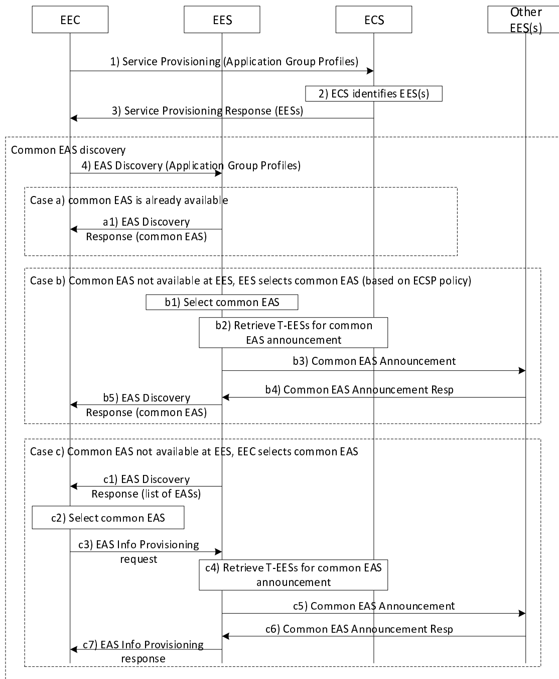
Figure E.2.2-1: Common EAS discovery and announcement (without repository function)
