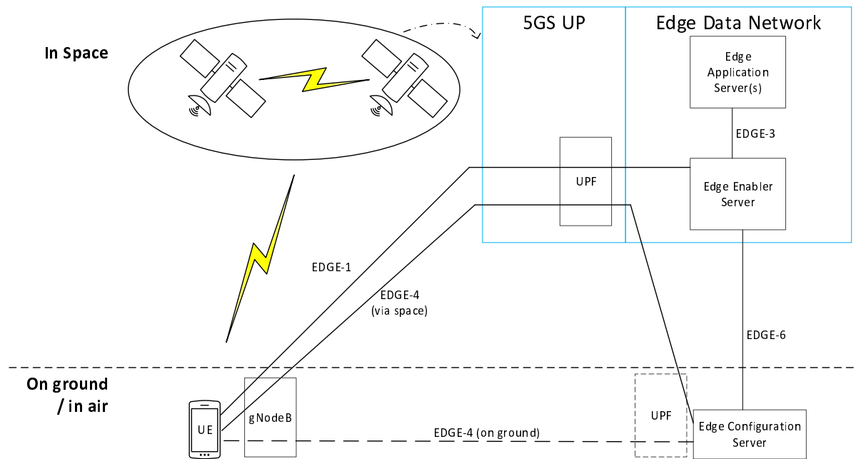
Figure A.2.5-2: EDN deployment with gNB on ground
