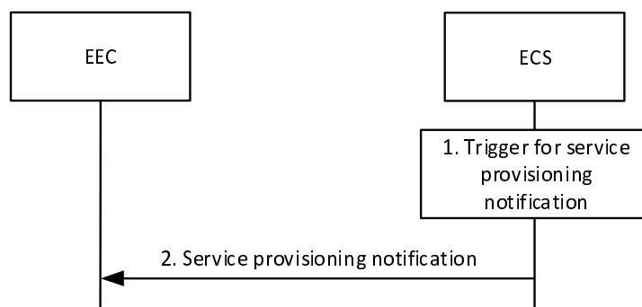
Figure 8.3.3.2.3-1: Service provisioning notification
