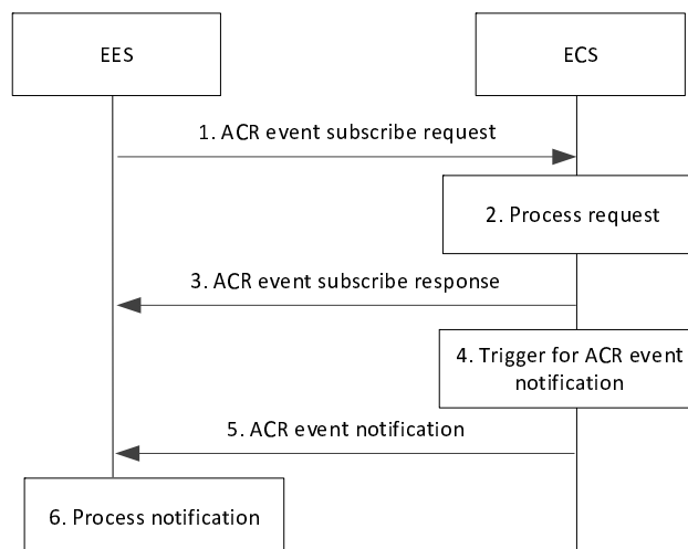
Figure 8.8.3.11-1: Subscribe and notify ACR event procedure
