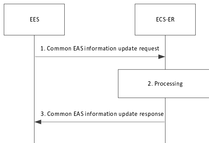
Figure 8.20.2.5-1: Common EAS information update
