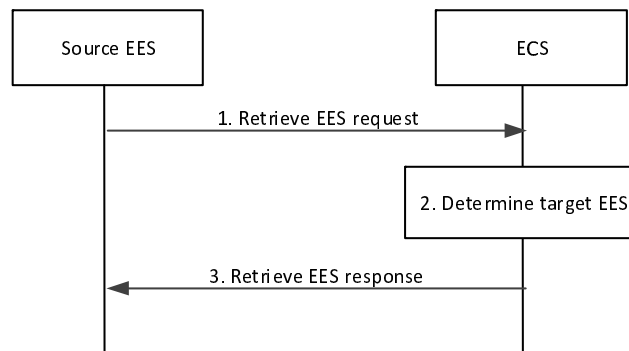
Figure 8.8.3.3-1: Retrieve T-EES procedure
