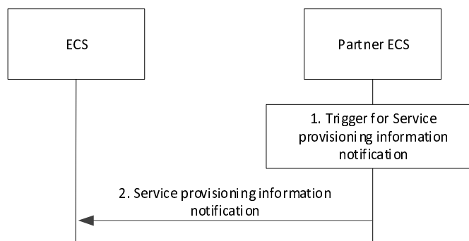
Figure 8.17.2.4.2.3.3-1: Service provisioning information notification
