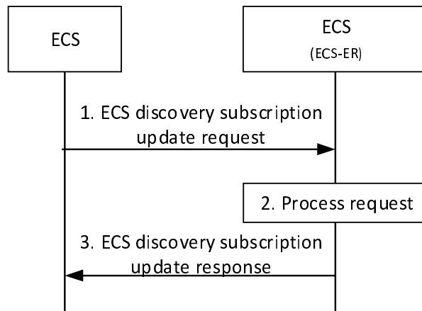
Figure 8.17.2.3.3.4-1: ECS discovery subscription update procedure
